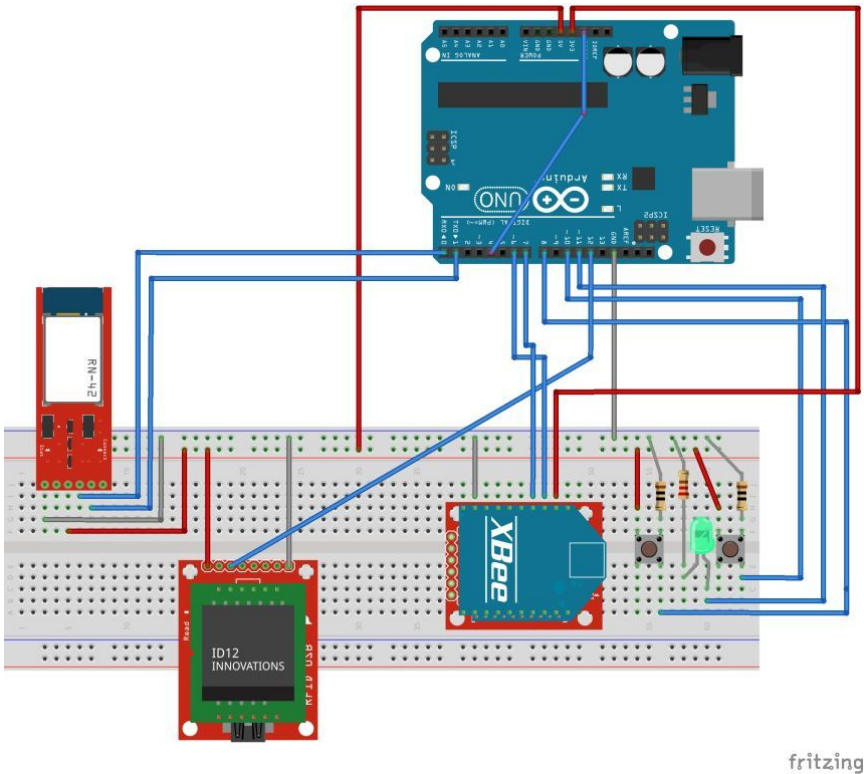
Figure C.2: Alpha Wiring
