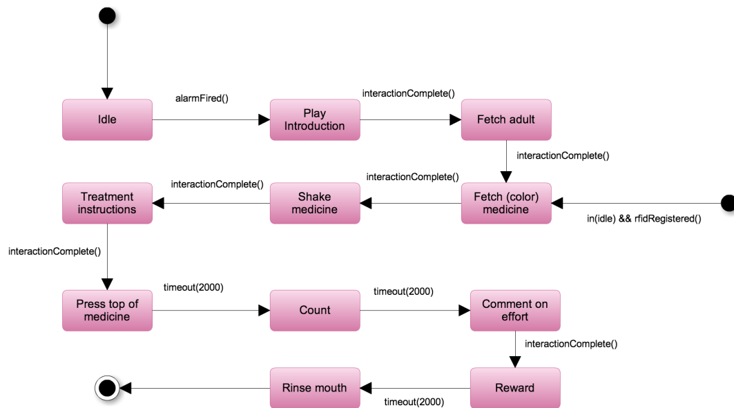
FIGURE 7.6: AsthmaBuddy State Diagram.
