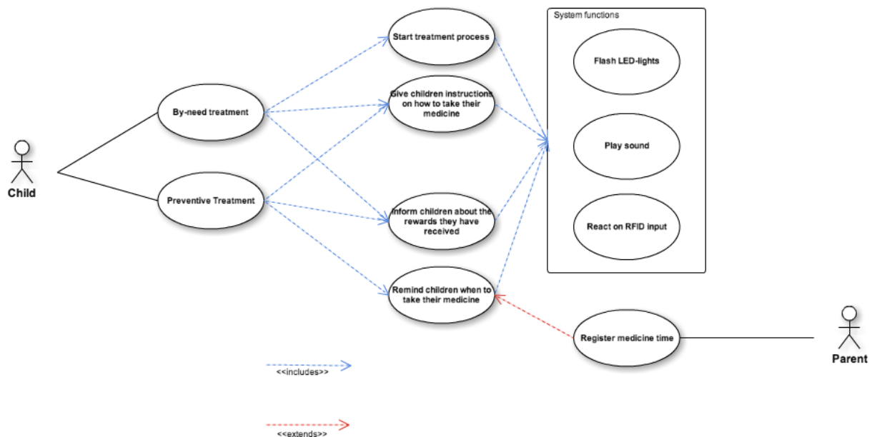
FIGURE 7.5: AsthmaBuddy Use Cases
