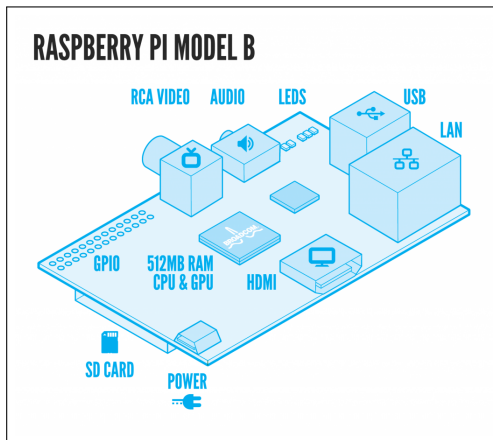
FIGURE 7.1: Raspberry Pi Model B architecture.
