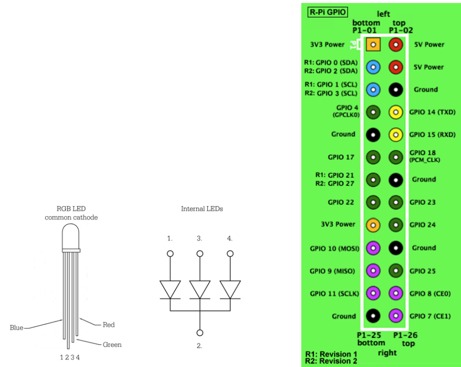
FIGURE D.1: RGB LED diagram. FIGURE D.2: Raspberry Pi GPIO.
