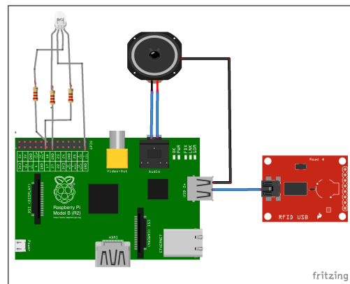
FIGURE 7.2: Digital schematic of the components
