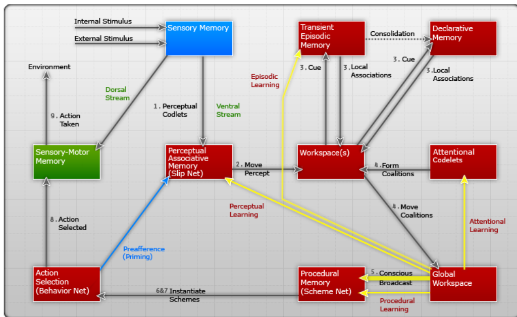
Figure 2.7: Overview of the LIDA cycle.[19]
