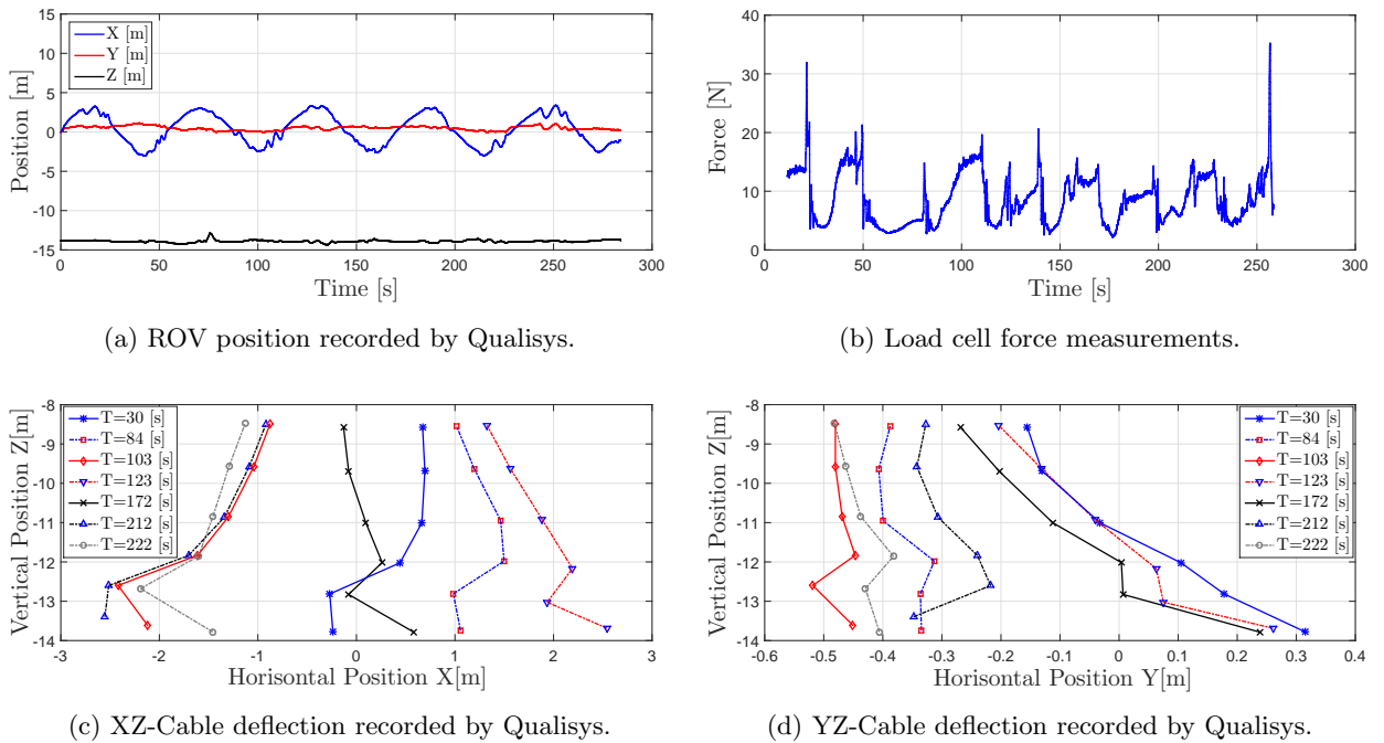
Figure 6: Experimental results from Experiment 1., where the ROV follows a forwards and backwards horizontal path.
