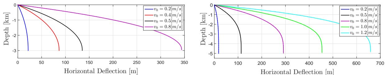
Figure 11: Static horizontal deflection for ROV-TMS with 3000 and 5000 meters cable length for different current velocities.
