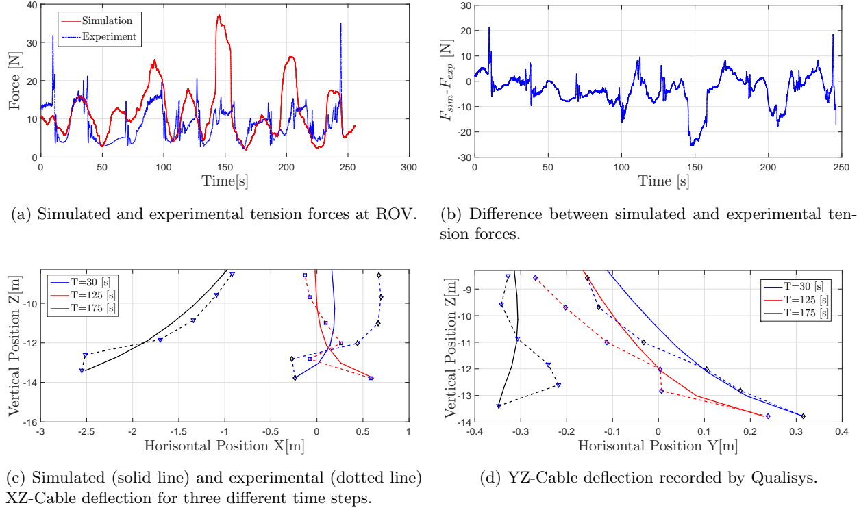
Figure 7: Experiment 1 (forward-backward): Simulated and experimental results.
