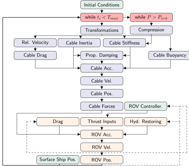
Figure 4: Flowchart of simulation program. Color code: green = external inputs, blue = cable related routines, yellow = ROV related routines and red = while loops. Dashed lines symbolize data-flow from previous time-step.
