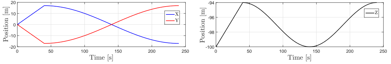
Figure 12: ROV reference motion for sensitivity analysis of hydrodynamic parameters
