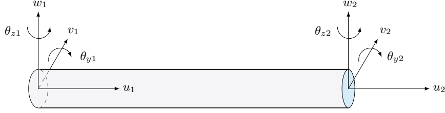
Figure 2: Sketch of two-node beam element in three-dimensional space. (u,v,w) are translational deflections and (\theta_y,\theta_z) are rotational deflections.
