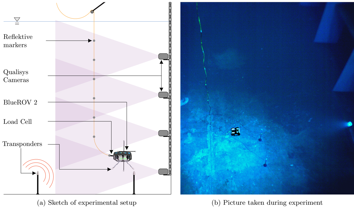
Figure 5: The Experimental setup with ROV, cameras and transponders
