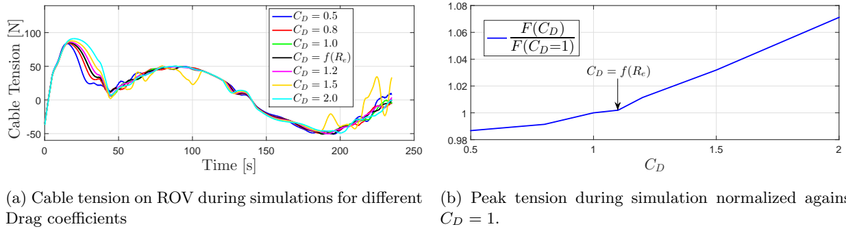
Figure 14: Drag coefficient sensitivity results
