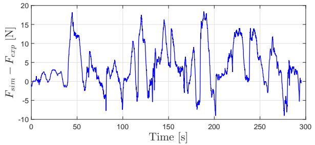
(b) Difference between simulated and experimental tension forces.
