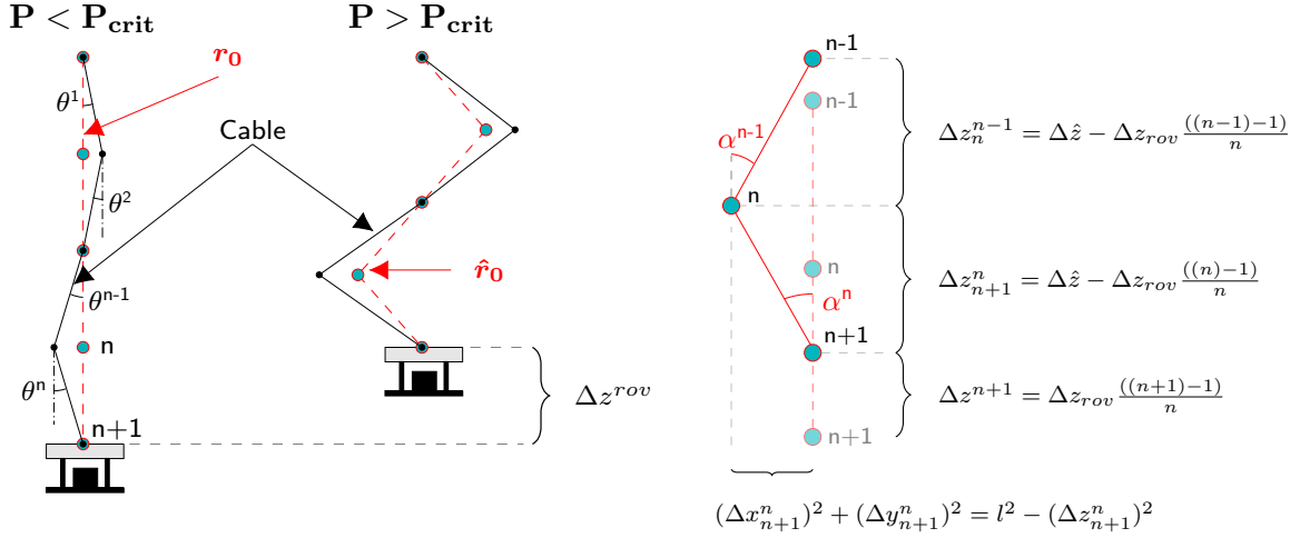
(a) Schematic representation of the equilibrium ( \mathbf{r}_0 ) and buckled equilibrium ( \hat{\mathbf{r}}_0 ) positions.
