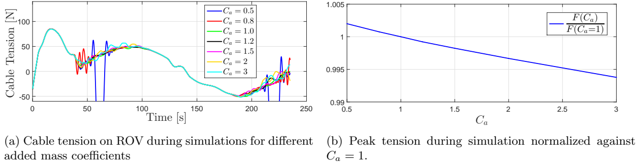
Figure 13: Added Mass coefficient sensitivity results
