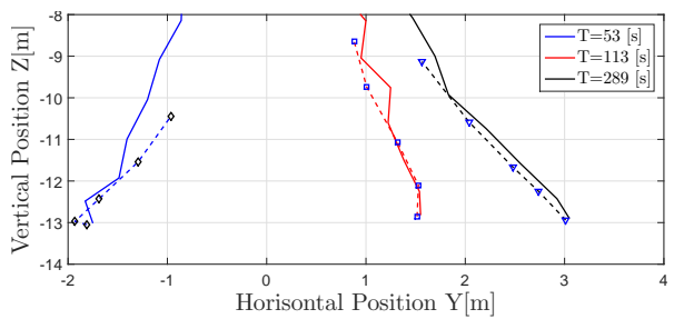
(d) Simulated (solid line) and experimental (dotted line) YZ-Cable deflection for three different time steps.
