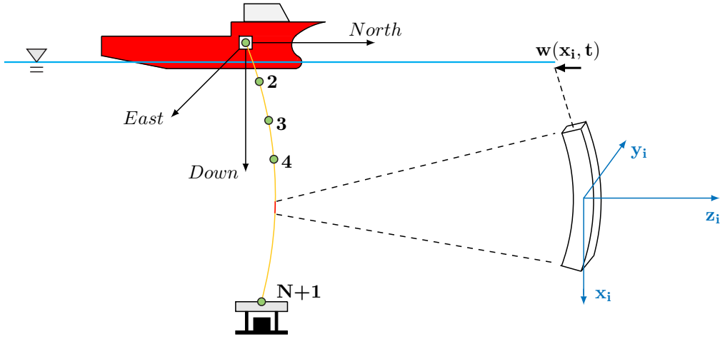
Figure 1: Reference frames, Inertial (NED) and for element i
