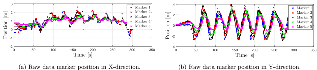
Figure 10: XY raw-data position measurement for experiment 2. Marker 1 is on the ROV
