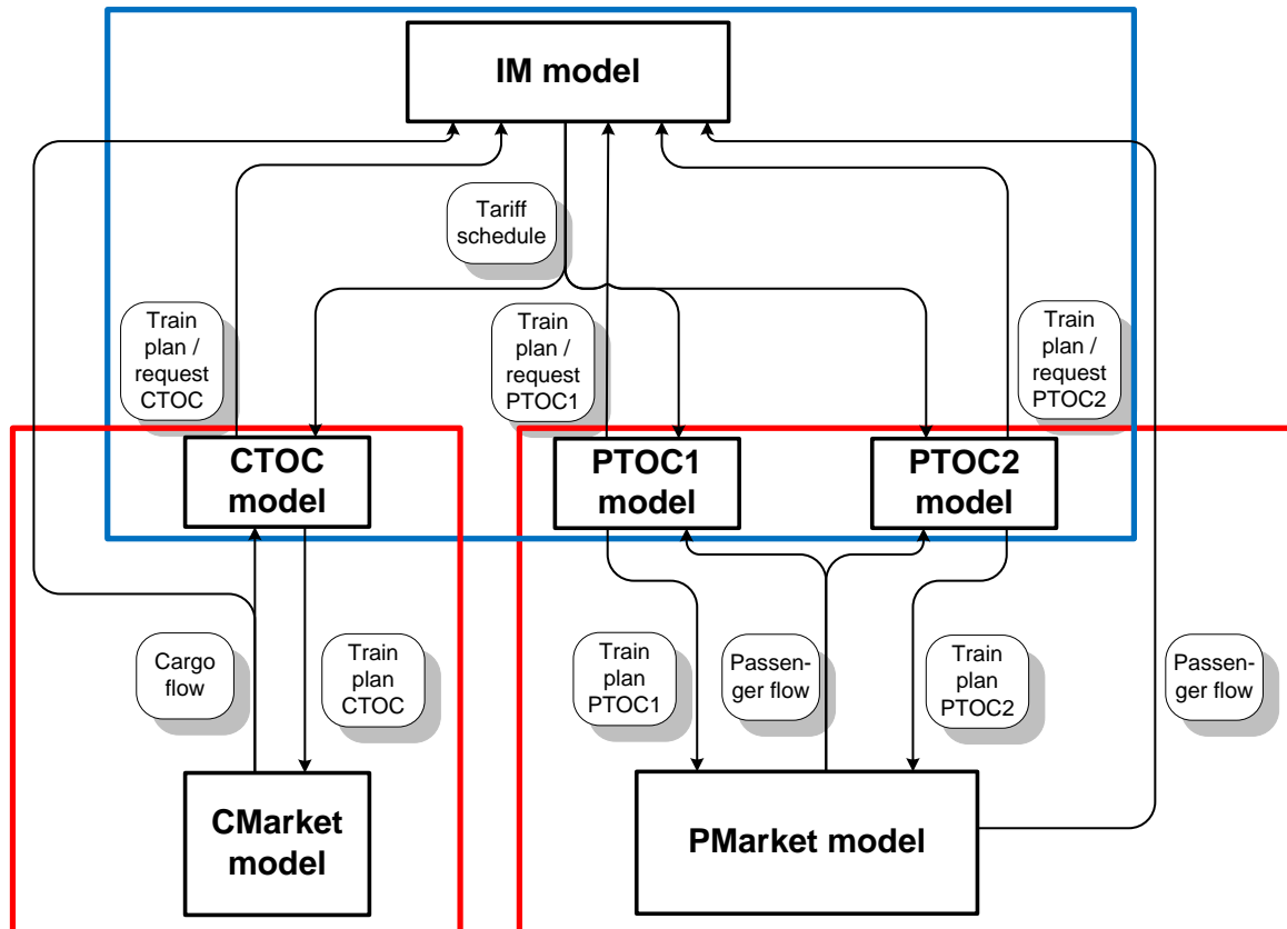
Figure 1: Three-level structure with two passenger TOCs and one cargo TOC; decomposition into IM–TOC and TOC–M sub-problems. The model presented in this report focusses on the IM–TOC relation.
