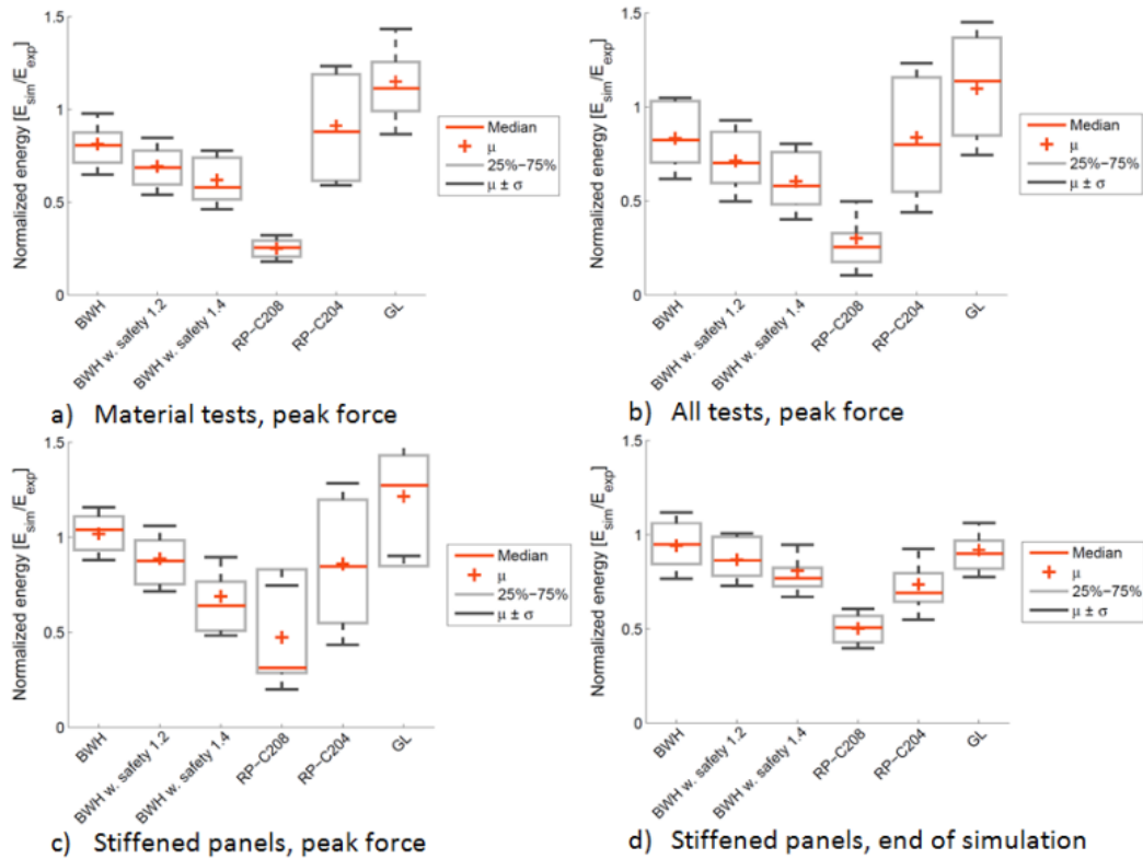
Fig. 5 Graphical view of statistical comparison of behavior of the tested fracture criteria.
