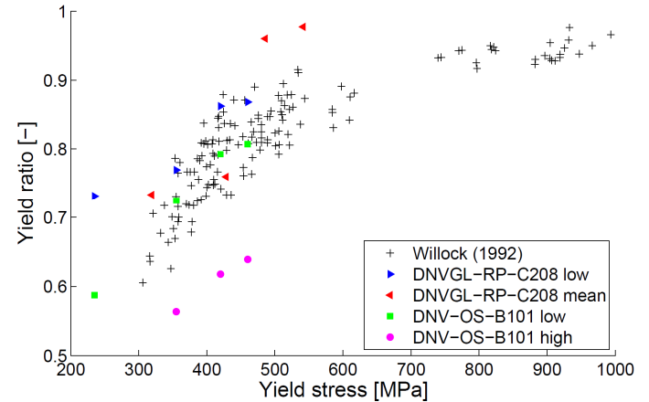
Fig. 1 Yield ratios for high-strength steels.
