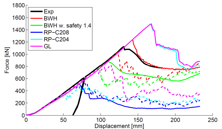
Fig. 4 Force-displacement results from simulation of the indentation experiment 2FB from Alsos and Amdahl [20].
