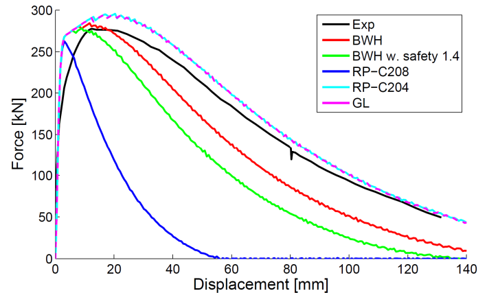
Fig. 3 Force-displacement results from simulation of the plate tearing tests from Simonsen og Törnqvist [19], 5 mm steel plate, element length equal to thickness.
