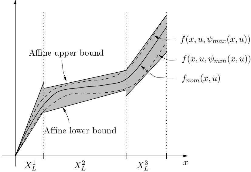
Figure 3.1: Illustration of the uncertainty modeling. The shaded area is accounted for in the controller synthesis. \psi_{max} and \psi_{min} should be taken as the “extreme” values of the uncertainty parameter, i.e something like \psi_{max}(x, u) = \arg \max_{\psi \in \Psi} f(x, u, \psi) .
