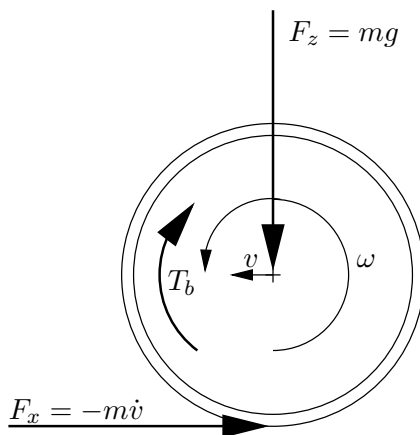
Figure 3.11: Velocities, forces and torque on quarter car
