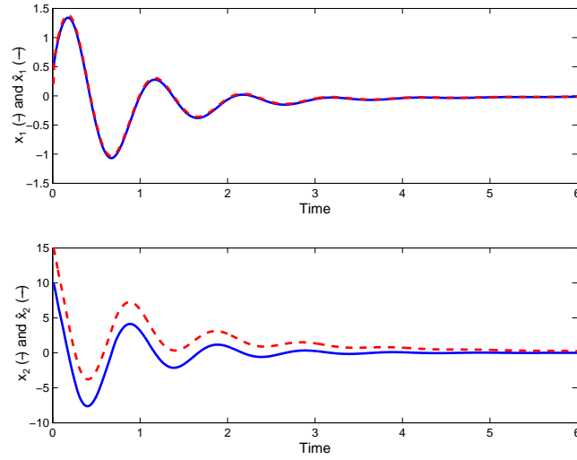
Figure 3.9: The state and the observer state simulated with the observer/controller synthesized using the separated synthesis, with initial conditions x = (.5, 10) and \tilde{x} = (.2, 15) .
