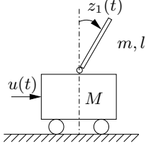
Figure 4.2: Inverted pendulum on a cart.
