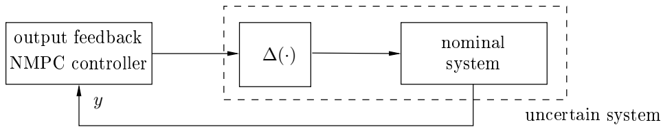
Figure 4.1: Closed loop with unknown static input nonlinearity
