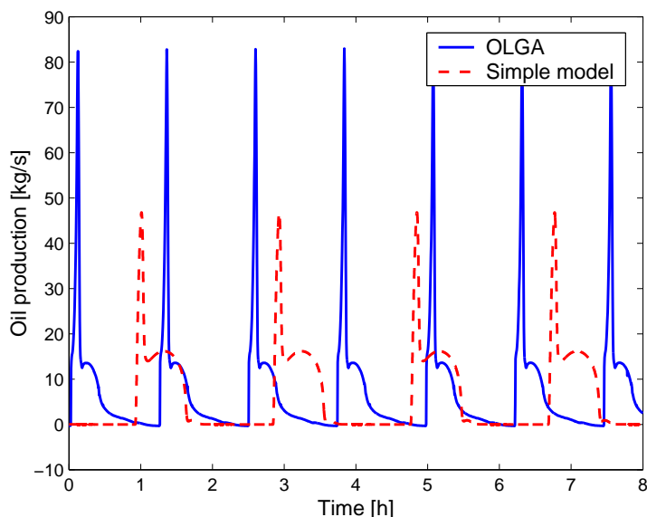
Figure 6.12: Comparison of open loop (gas lift choke is 50% open, production choke is 80% open) behavior between simple model and the rigorous multiphase flow simulator OLGA 2000.
