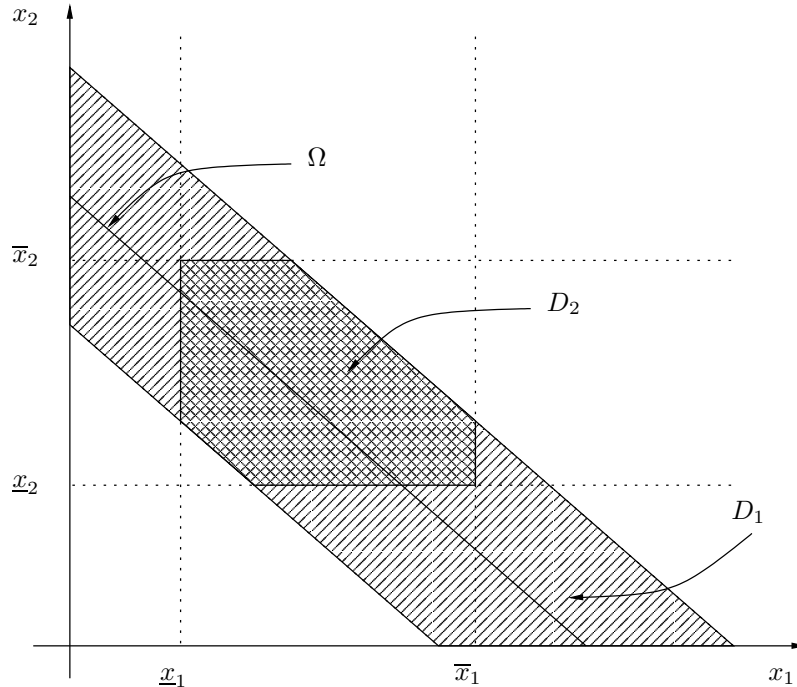
Figure 6.2: The sets D_1 and D_2 .
