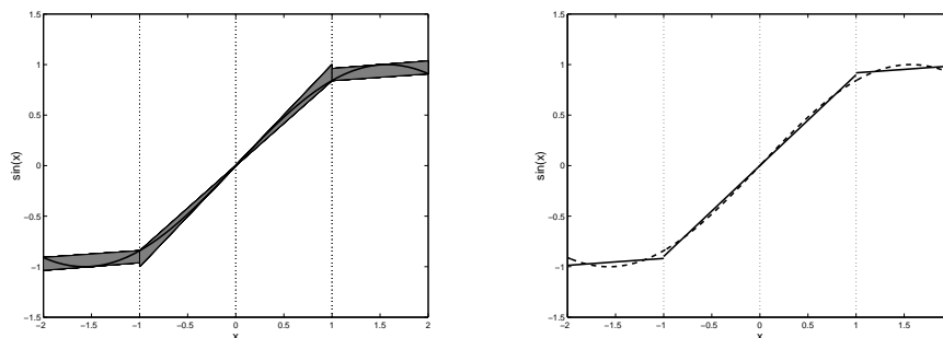
Figure 3.4: Piecewise affine bounding and approximation.
