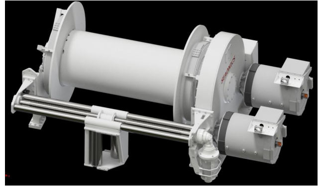
Figure 1: Seonics Big Drum Trawlwinch PM, designed for trawling on deep water and rough bottoms, in arctic conditions. The winch is delivered with permanent magnet (PM) or conventional AC motors for both demersal and pelagic trawling. Image courtesy of Seonics AS.
