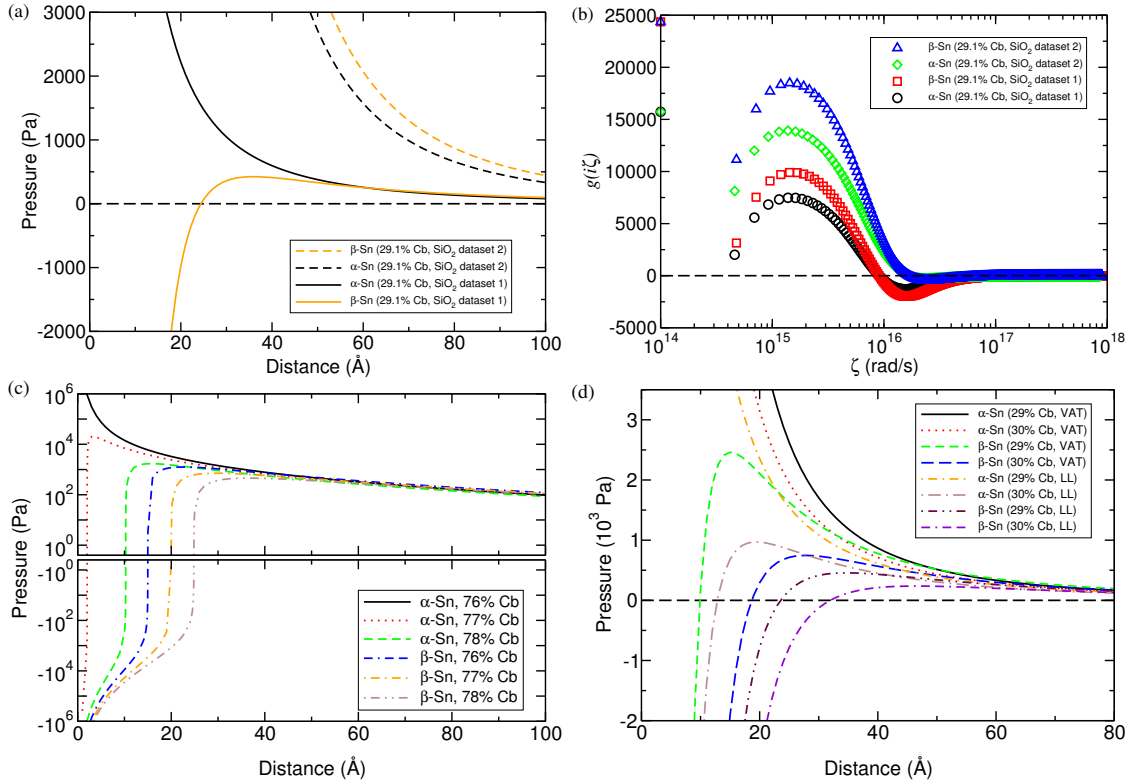
Figure 8. (Color online) (a) The Lifshitz pressure as a function of the separation distance between SiO 2 and α-Sn or β-Sn across a liquid mixture of chlorobenzene and bromobenzene using two different parameterizations for the dielectric function of SiO 2 , i. e., datasets 1 and 2. (b) Spectral functions revealing the contribution of each frequency mode to the Lifshitz pressures for the two different dielectric functions of SiO 2 . The zero frequency term is divided by a factor of 2. (c) The Lifshitz pressure as a function of the separation distance between SiO 2 and α-Sn or β-Sn across a liquid mixture of chlorobenzene and bromobenzene using SiO 2 dataset 2; this can be compared with Fig. 3, where SiO 2 dataset 1 is used. (d) The Lifshitz pressure as a function of the separation distance between SiO 2 and α-Sn or β-Sn across a liquid mixture of chlorobenzene and bromobenzene using SiO 2 dataset 1 with two different models to describe the dielectric function of the liquid mixture, namely the Lorentz-Lorenz-like (LL) and the volume average theory (VAT) models.
