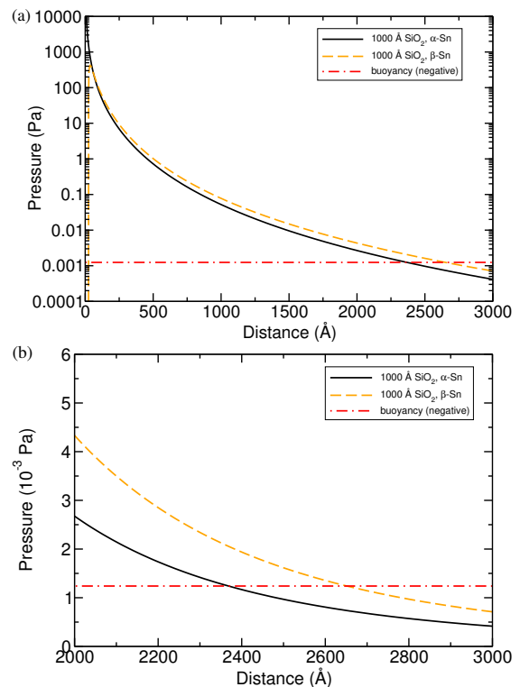
Figure 7. (Color online) (a) The Lifshitz pressure as a function of the separation distance between SiO 2 (dataset 1) and \alpha -Sn or \beta -Sn across a liquid mixture (29.1% chlorobenzene in bromobenzene) compared to the attractive buoyancy pressure (here, presented on a positive scale). (b) Magnification of the distance region where the repulsive Lifshitz and the attractive buoyancy pressures compensate each other.
