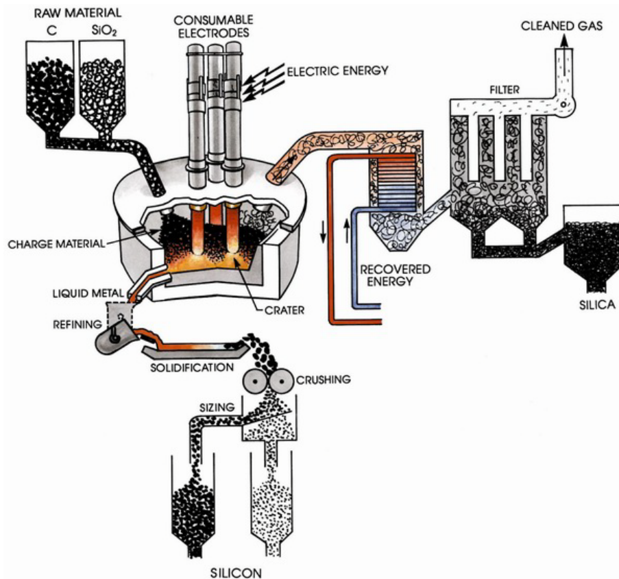
Figure 2: Typical plant layout: industrial production of metallurgical-grade silicon [12]
