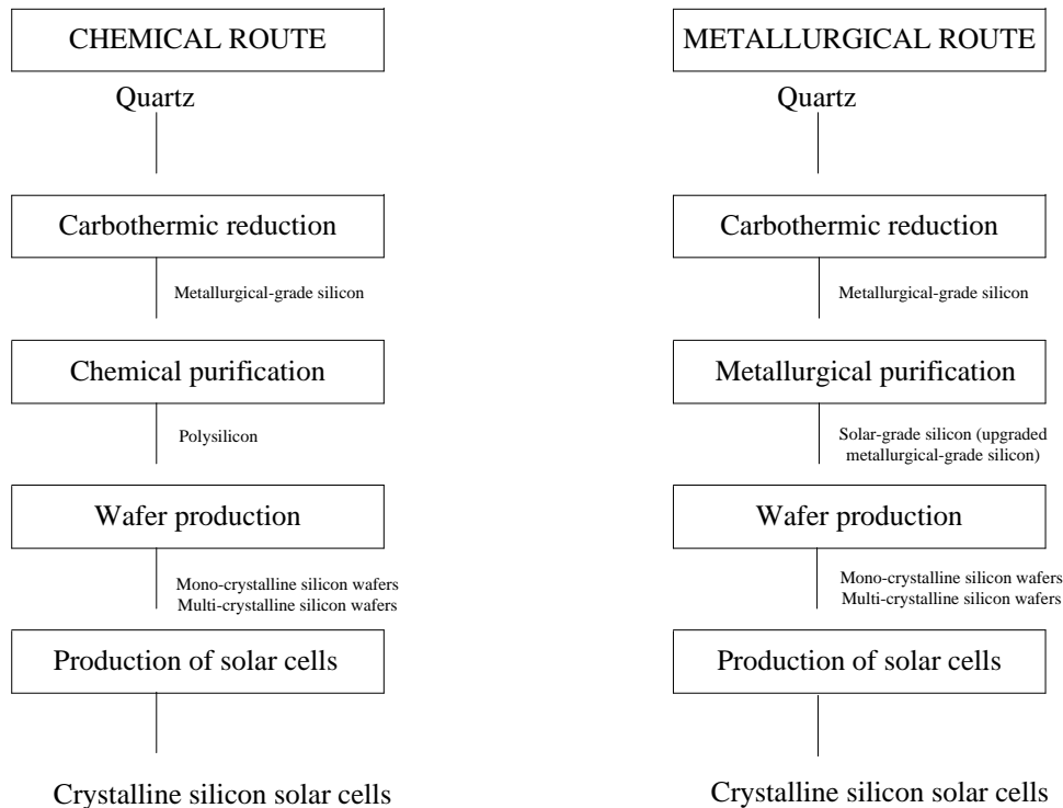
Figure 1: Stages for the production of crystalline silicon solar cells from quartz
