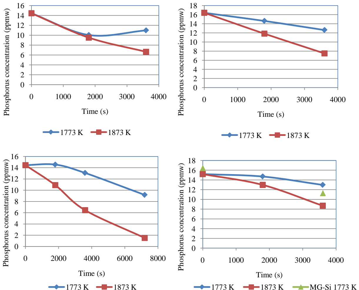
Figure 16: Phosphorus concentration as a function of refining time at different temperatures and iron concentrations: 0 ppmw (top left), 500 ppmw (top right), 2000 ppmw (bottom left), 5000 ppmw (bottom right).
