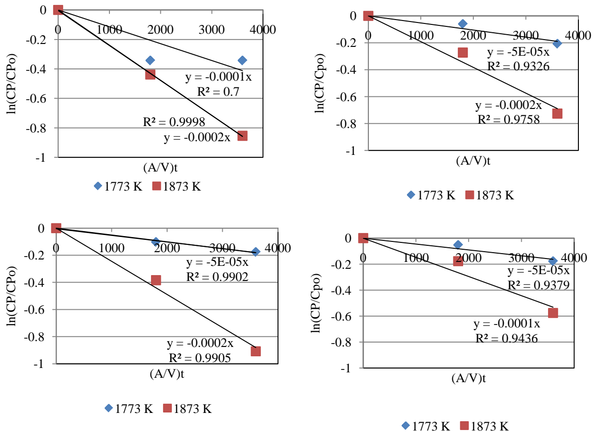
Figure 17: Plot of \ln(C_P/C_{P_0}) versus (A/V)t for phosphorus at different temperatures and iron concentrations: 0 ppmw (top left), 500 ppmw (top right), 2000 ppmw (bottom left), 5000 ppmw (bottom right).
