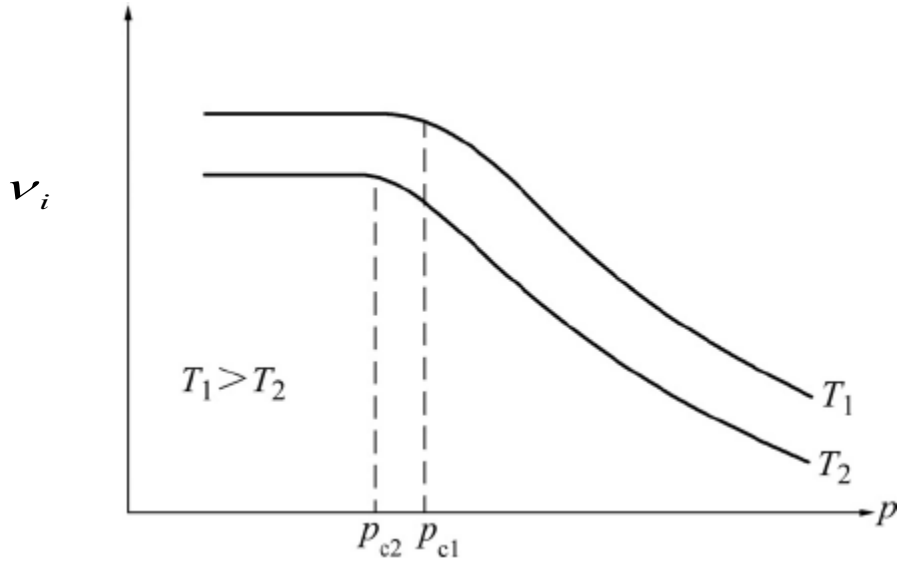
Figure 7: Relationship between evaporation rate and chamber pressure [35]
