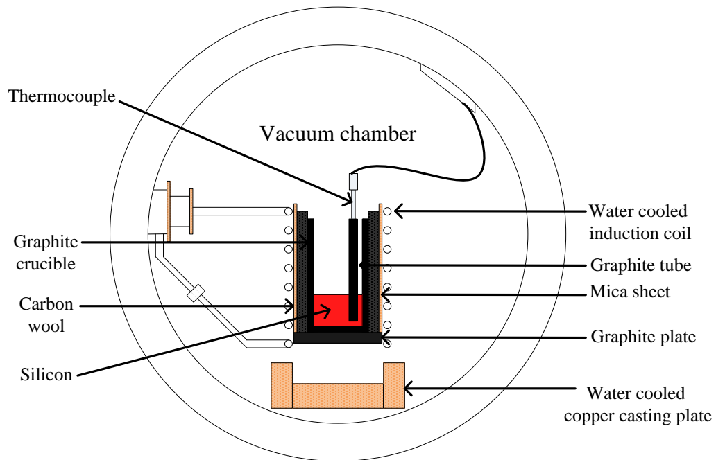
Figure 14: Schematic diagram of the vacuum chamber with a crucible in place
