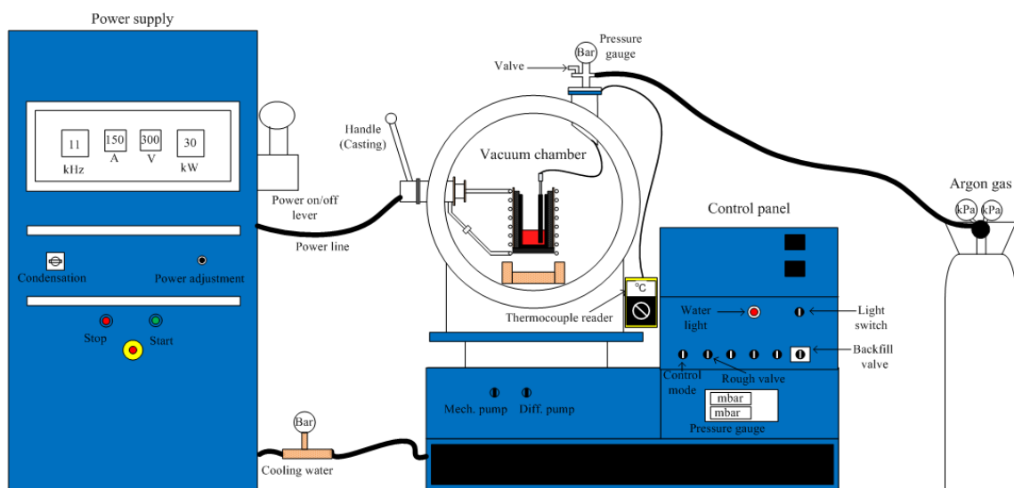
Figure 12: Schematic diagram of the experimental facility set-up
