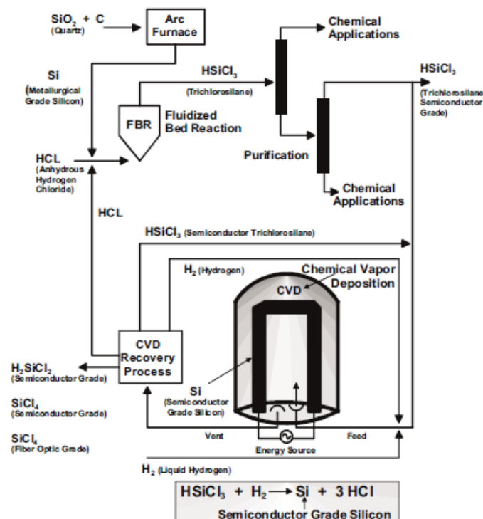
Figure 4: Typical flowsheet for industrial polysilicon production via the Siemens
