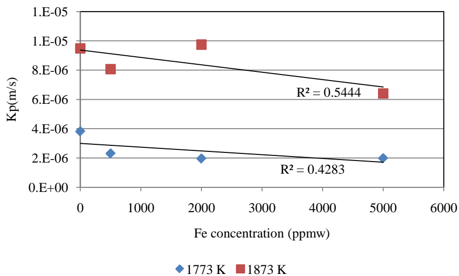
Figure 18: Mass transfer coefficients as a function of Fe concentration
