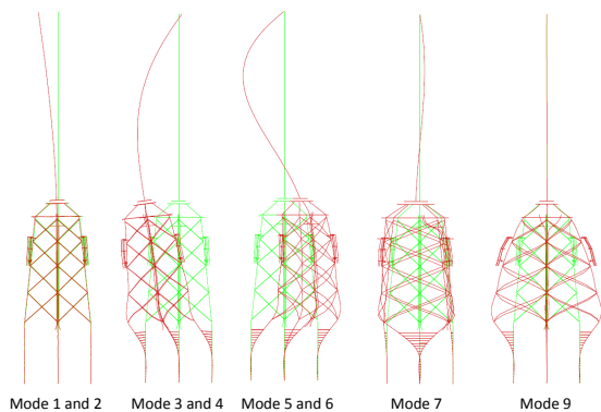
Figure 5. The first nine modeshapes of the ASAS model.
