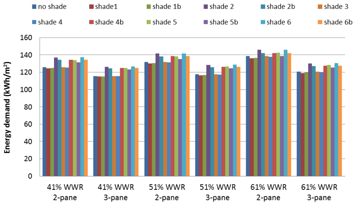
Figure 5. Net energy demand of two-person offices with south-facing façades for the different shading strategies.
