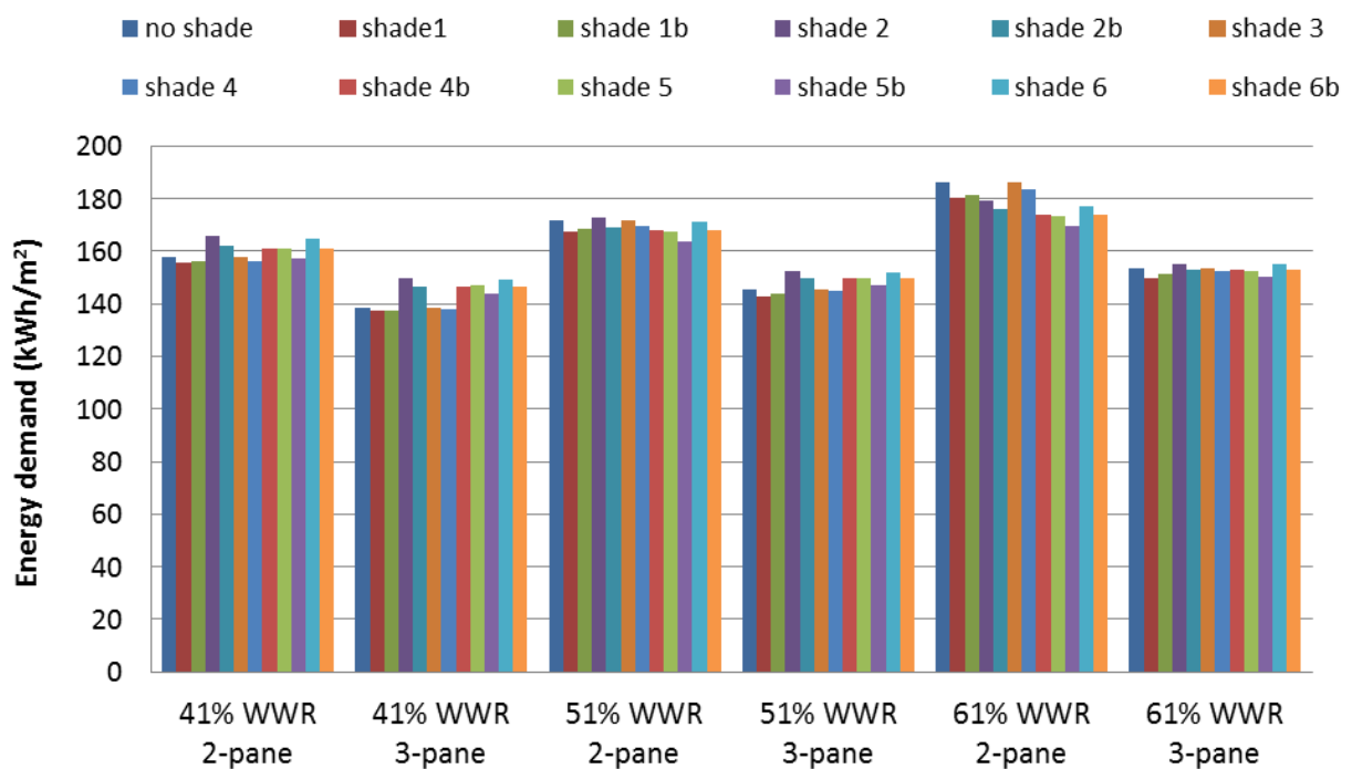
Figure 4. Net energy demand of single-person cubicles with south-facing façades for the different shading strategies.
