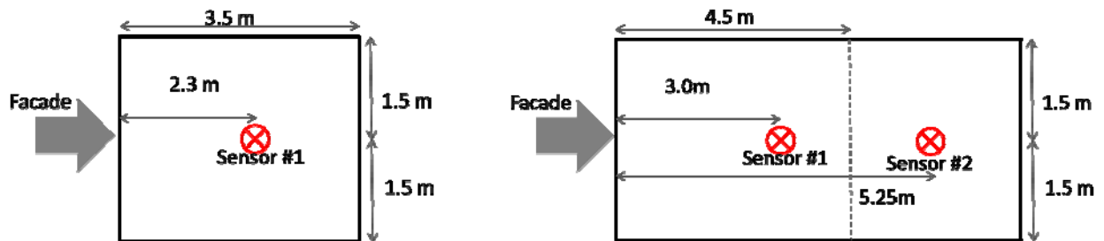
Figure 2. On the left: illustration showing the placement of the daylight sensor in the single-person cubicle. On the right: illustration showing the placement of the daylight sensors in the two-person office space.
