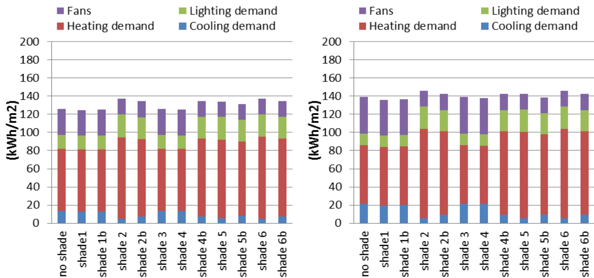
Figure 3. Energy demand for heating, cooling, lighting and ventilation fans (kWh/m 2 heated floor area) for south-facing offices. Upper-left graph shows the two-pane 41 % WWR single-person cubicle; the upper-right graph shows the two-pane 61 % WWR single-person cubicle; the lower-left graph shows the two-pane 41 % WWR two-person office; the lower-right graph shows the two-pane 61 % WWR two-person office.
