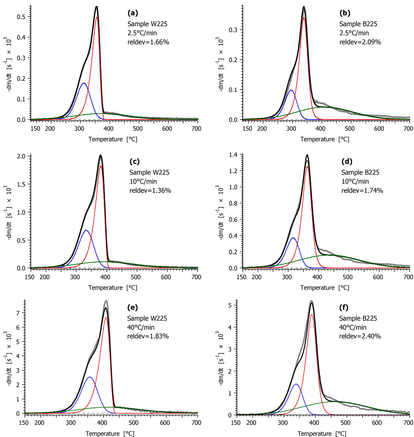
Figure 5. Kinetic curve fitting at linear T(t) programs from the results of Evaluation 3.1. The experiments on the samples torrefied at 225 ^{\circ}\text{C} are shown. Notation: thick gray line, -\frac{dm^{obs}}{dt} ; thick black line, -\frac{dm^{calc}}{dt} ; blue, red and green lines, mass loss rate curves of the pseudo-components. (See Figure 6 and the Supporting Information for more figures from this evaluation.)
