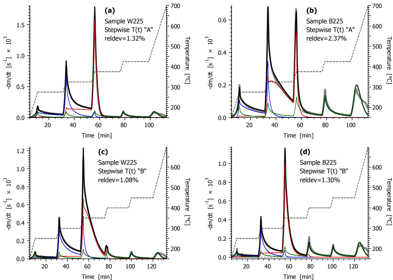
Figure 6. Kinetic curve fitting at stepwise T(t) programs from the results of Evaluation 3.1. The experiments on the samples torrefied at 225^{\circ}\text{C} are shown. Notation: dashed gray line, T(t) ; thick gray line, -dm^{obs}/dt ; thick black line, -dm^{calc}/dt ; blue, red and green lines, mass loss rate curves of the pseudo-components. (See Figure 5 and the Supporting Information for more figures from this evaluation.)
