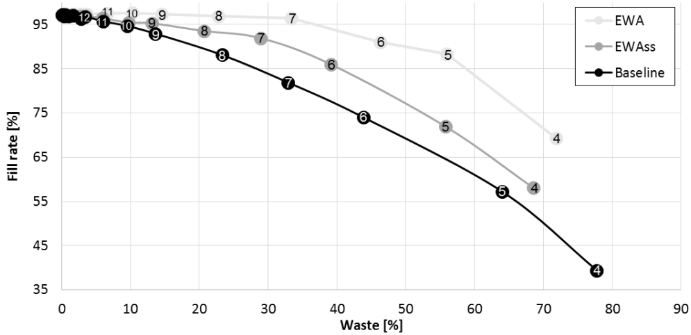
Figure 2: One year average waste across all stores and warehouse and fill rate across stores
