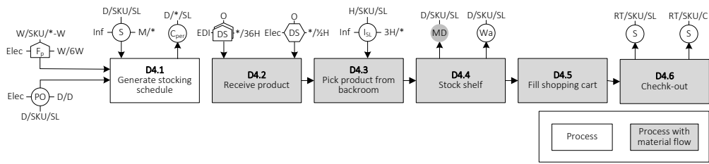
Figure 4.3: Information flow combined with SCOR Retail Deliver process (D4)
