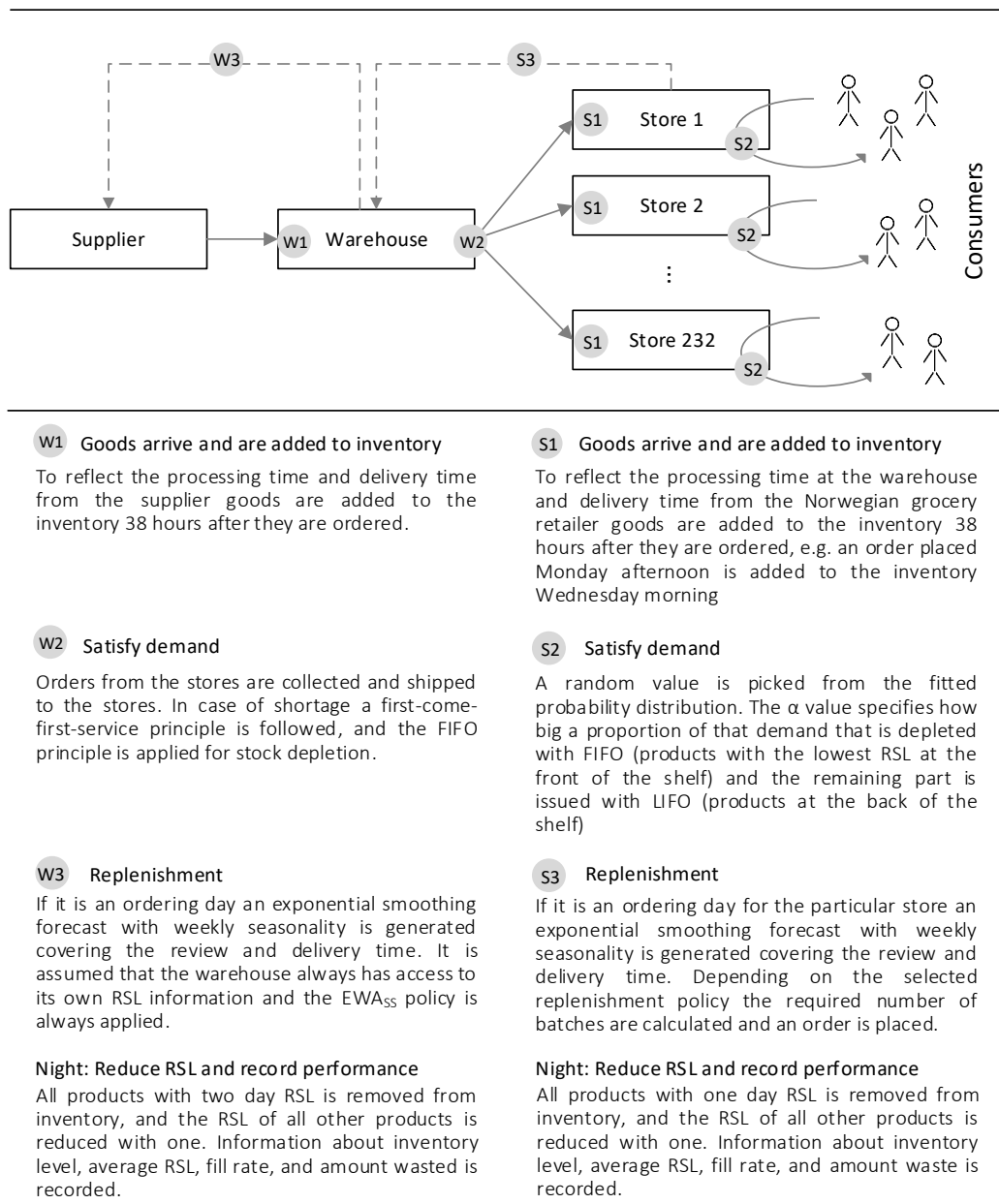
Figure 1: Events in the simulation model
