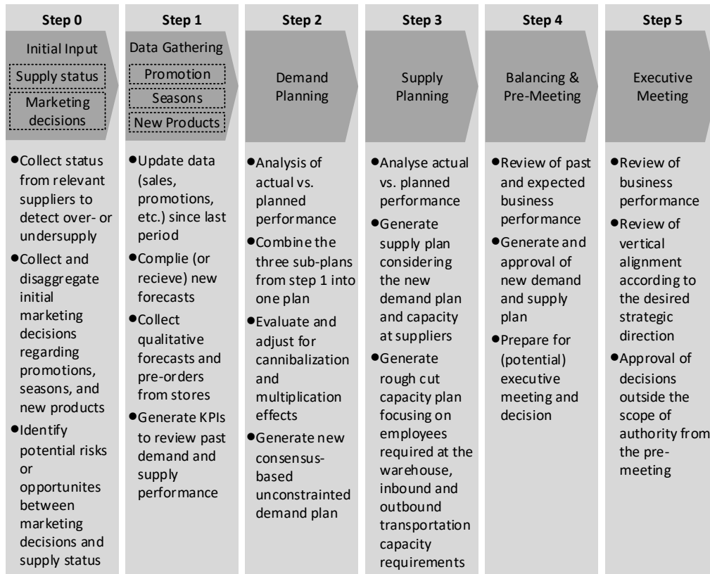
Figure 6: Proposed S&OP process for grocery retailing
