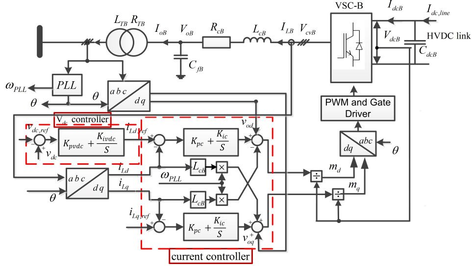
Fig. 4: The control structure of dc voltage control converter, VSC-B.
