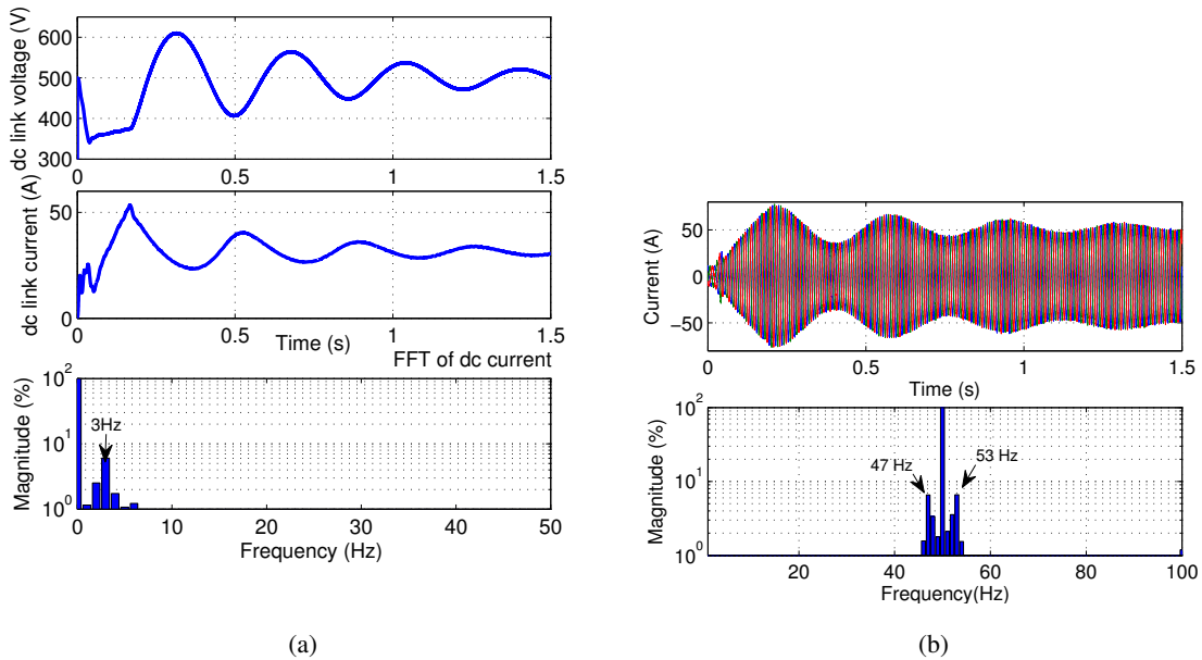
Fig. 20: Simulation results: (a) The dc link voltage and current and FFT of dc current for dc voltage controller proportional gain of 0.03, (b) The three-phase current at PCC of VSC-B for dc voltage controller proportional gain of 0.03.
