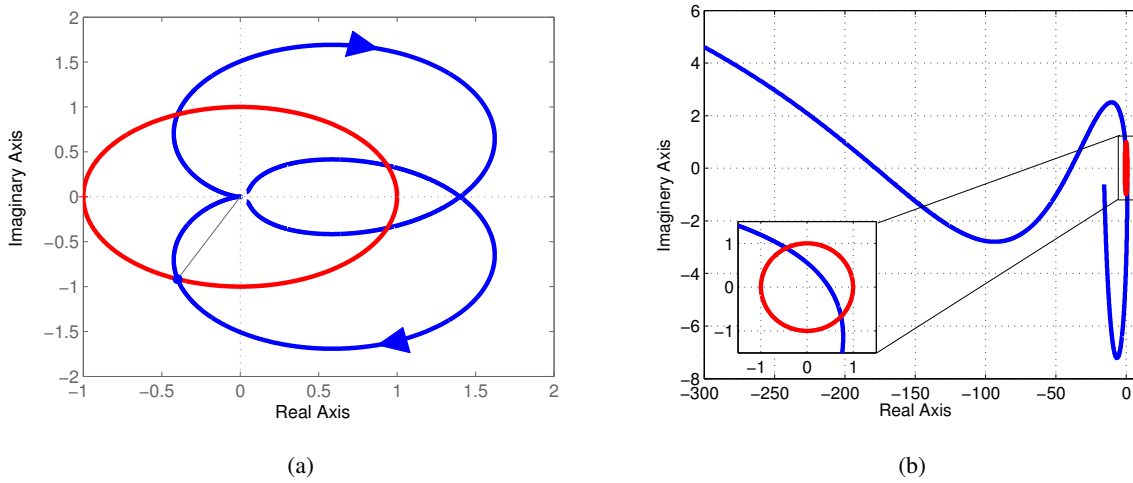
Fig. 17: Nyquist plot of impedance ratio for modified control tuning: (a) Negative power reference: Z_{Vdc}(s)/Z_P(s) and (b) Positive power reference: Z_P(s)/Z_{Vdc}(s) .
