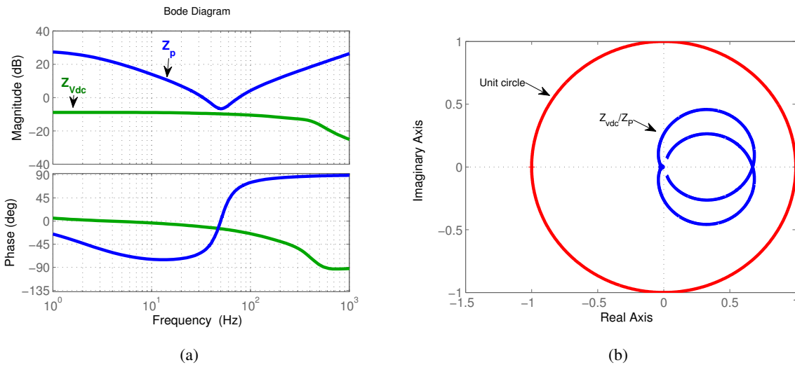
Fig. 12: Negative power reference: (a) Impedance frequency response of the voltage source and current source subsystem and (b) the Nyquist plot of the impedance ratio ( Z_{Vdc}(s)/Z_P(s) ).
