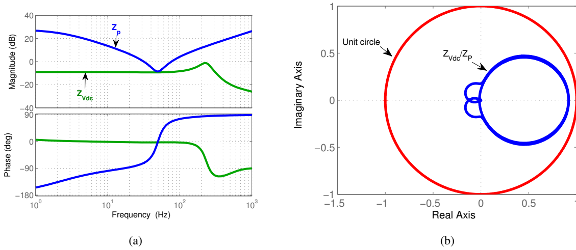
Fig. 13: Positive power reference: (a) Impedance frequency response of the voltage source and current source subsystem and (b) the Nyquist plot of the impedance ratio ( Z_{Vdc}(s)/Z_P(s) ).
