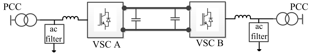
Fig. 1: Point-to-point connection VSC-based HVDC system
