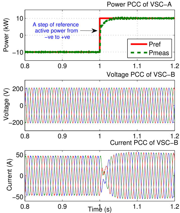
Fig. 18: Simulation results for a step change of power reference from negative to positive 10 kW.
