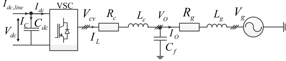
Fig. 2: Overview of VSC-HVDC converter station
