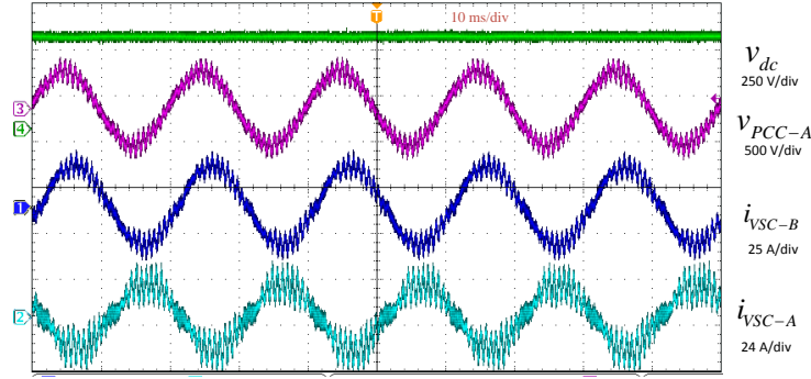
Fig. 25: Experimental results for power controller proportional gain of 2 \times 0.005 : (i) dc link voltage, (ii) voltage at PCC of VSC-A (phase-a), current of (iii) VSC-B (phase-a) and (iv) VSC-A (phase-a).
