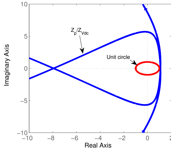
Fig. 15: Nyquist plot of impedance ratio, Z_P(s)/Z_{Vdc}(s) .
