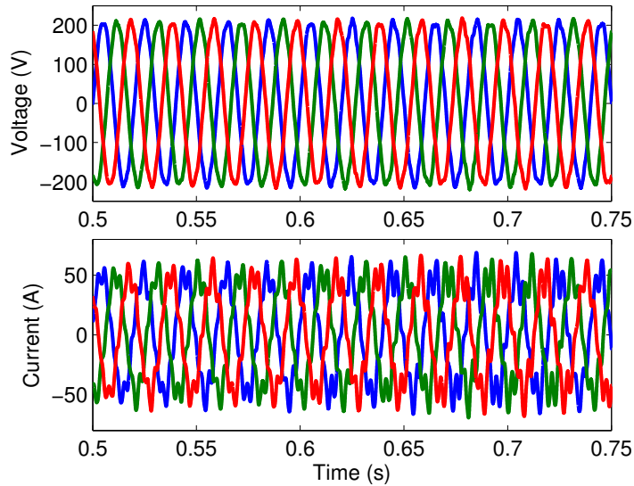
Fig. 7: Simulation results for +10 kW power reference to the VSC-A (Unstable case): The three-phase voltage and current at PCC of VSC-B.
