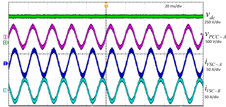
Fig. 6: Experimental results for -10 kW power reference to the VSC-A (Stable case): dc link voltage, voltage at PCC of VSC (phase-a), current of VSC-A (phase-a) and VSC-B (phase-a).
