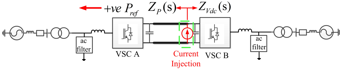
Fig. 9: Investigated point-to-point VSC-based HVDC system including current injection structure for impedance model verification
