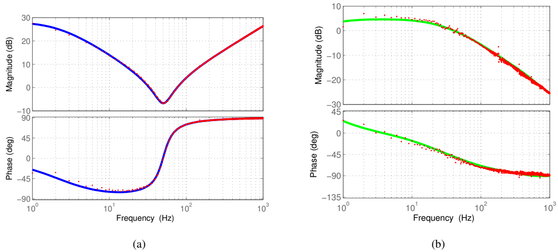
Fig. 11: Frequency response of the impedance: (a) the impedance of the current source subsystem and (b) the impedance of the voltage source subsystem (solid-line is from model prediction and the red-points are from detailed simulation).
