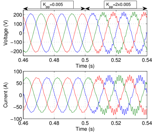
Fig. 24: The three-phase voltage and current at PCC of VSC-A for a change of the power controller proportional gain from 0.005 to 2x0.005 at 0.5 s.
