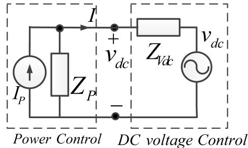
Fig. 10: Equivalent small-signal impedance model of VSC-HVDC system consisting of both the voltage source and the current source.
