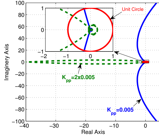
Fig. 23: Nyquist plot of impedance ratio, Z_{V_{dc}}^*(s)/Z_P^*(s) (blue line is for k_{pp} = 0.005 and green-dash line is for k_{pp} = 2x0.005 ).
