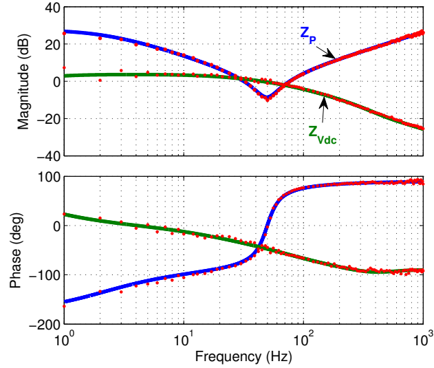
Fig. 16: Frequency response of the impedance model at interfacing point for modified control tuning (the solid-line is from model prediction and the red-points are from detailed simulation).
