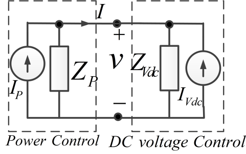
Fig. 14: Equivalent small-signal impedance model of VSC-HVDC system: current source equivalent model.
