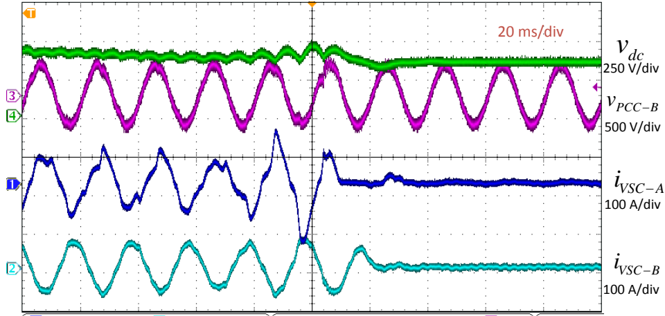
Fig. 8: Experimental results for +10 kW power reference to the VSC-A (Unstable case): dc link voltage, voltage at PCC of VSC (phase-a), current of VSC-A (phase-a) and VSC-B (phase-a).
