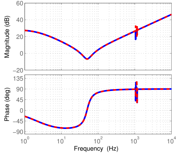
Fig. 21: Impedance frequency response for different value of proportional gain of power controller (Solid-blue line is for k_{pp} = 0.005 and red-dash line is for k_{pp} = 2 \times 0.005 ).
