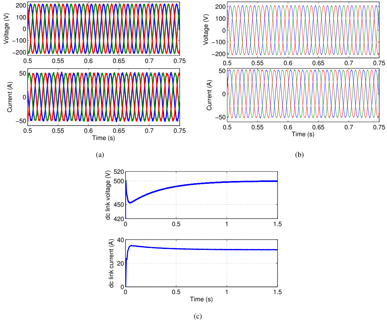
Fig. 5: Simulation results for -10 kW power reference to the VSC-A (Stable case): (a) Three-phase ac voltage and current at PCC of VSC-A, (b) Three-phase ac voltage and current at PCC of VSC-B and (c) dc link voltage and current of VSC HVDC system.
