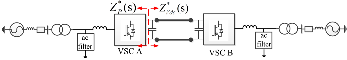
Fig. 22: Point-to-point VSC-based HVDC system to study the impact of power controller dynamics.
