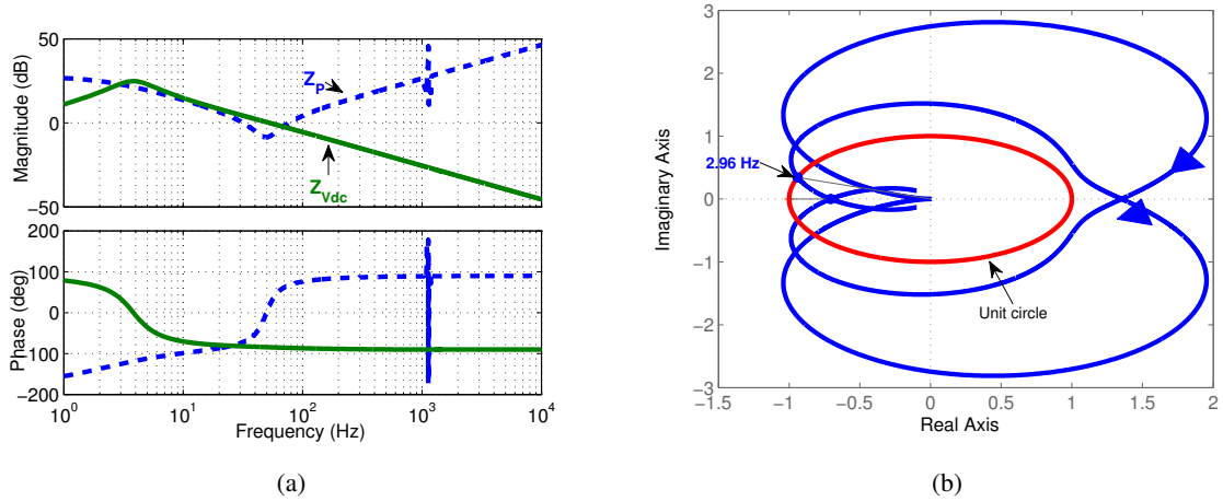
Fig. 19: (a) Impedance of the subsystem for dc voltage control proportional gain of 0.03 and (b) Nyquist plot of impedance ratio, Z_{Vdc}(s)/Z_P(s) .
