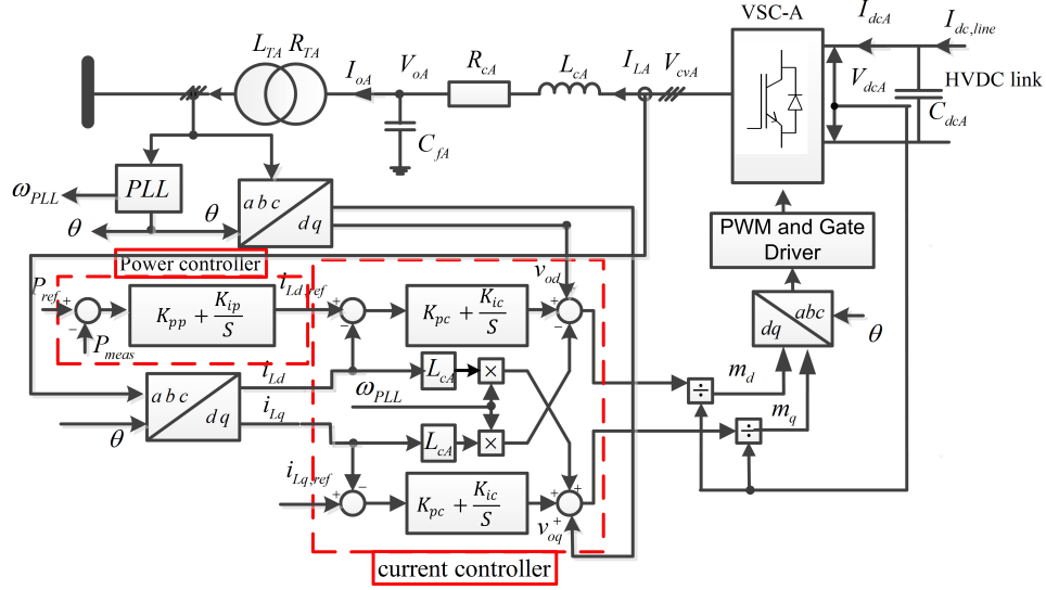
Fig. 3: The control structure of the power control converter, VSC-A.
