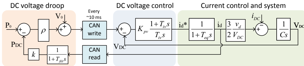
Figure 4 Block diagram of the implemented DC voltage droop control
