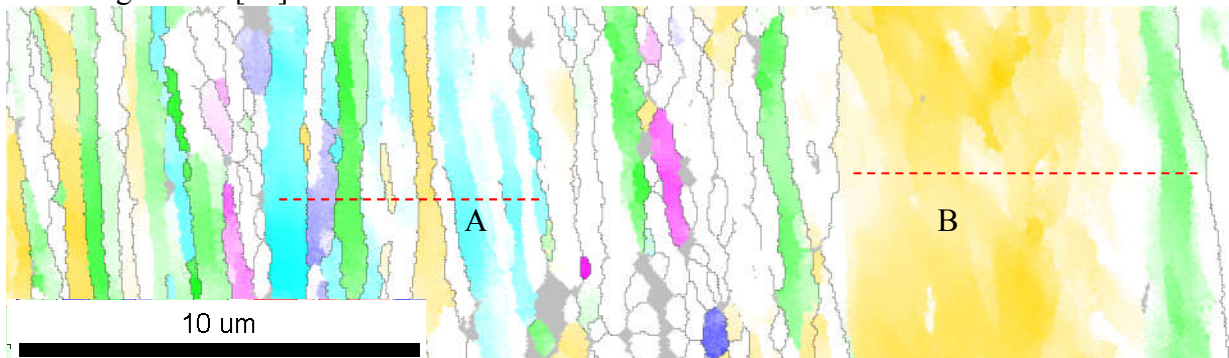
Fig. 4 The structure of BH at a strain of 3.3, illustrating the distributions of micro-textures and grain subdivision. Noise points are in grey; high angle grain boundaries are black lines. Several texture components are in color, i.e. Copper \{112\}\langle 111\rangle , S \{123\}\langle 634\rangle , Goss \{011\}\langle 100\rangle , Brass \{110\}\langle 112\rangle , and \{025\}\langle 100\rangle . Maximum deviation from the ideal orientation is 12^\circ .
