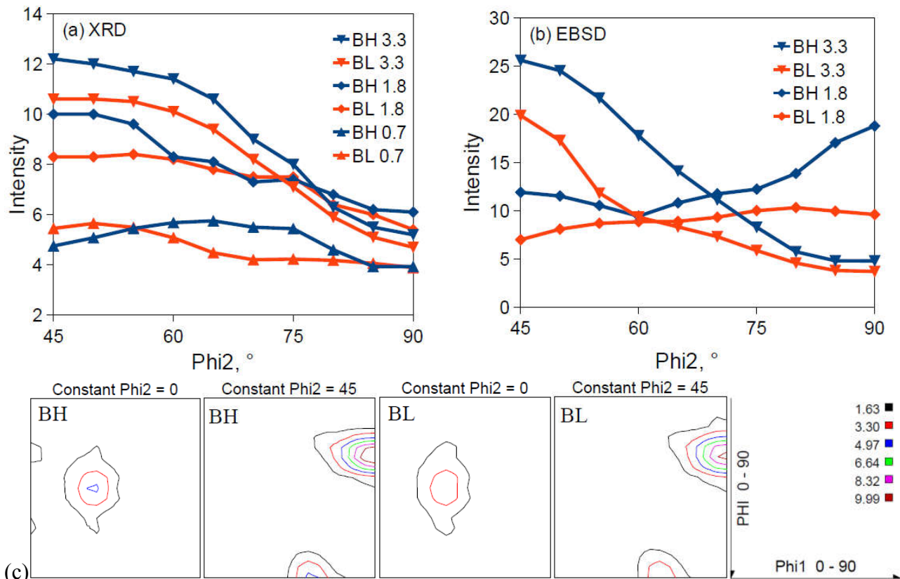
Fig. 3 a) macro-textures measured by X-ray diffraction; b) micro-textures measured by EBSD; c) Selected sections of ODF measured by X-ray diffraction at a strain of 3.3.
