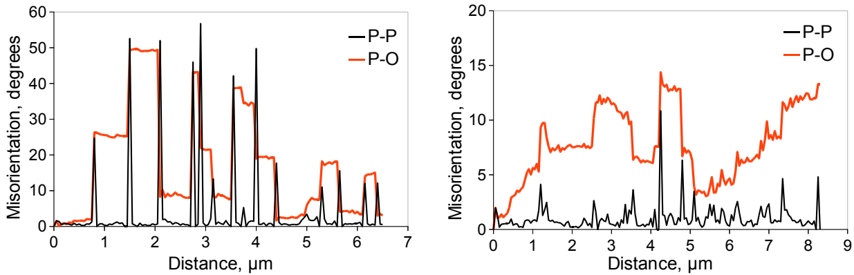
Fig. 5 misorientation profile along line A (a) and along line B (b) in Fig.7, showing (P-P shows the misorientations between adjacent points, P-O shows the misorientations compared to the original point.)
