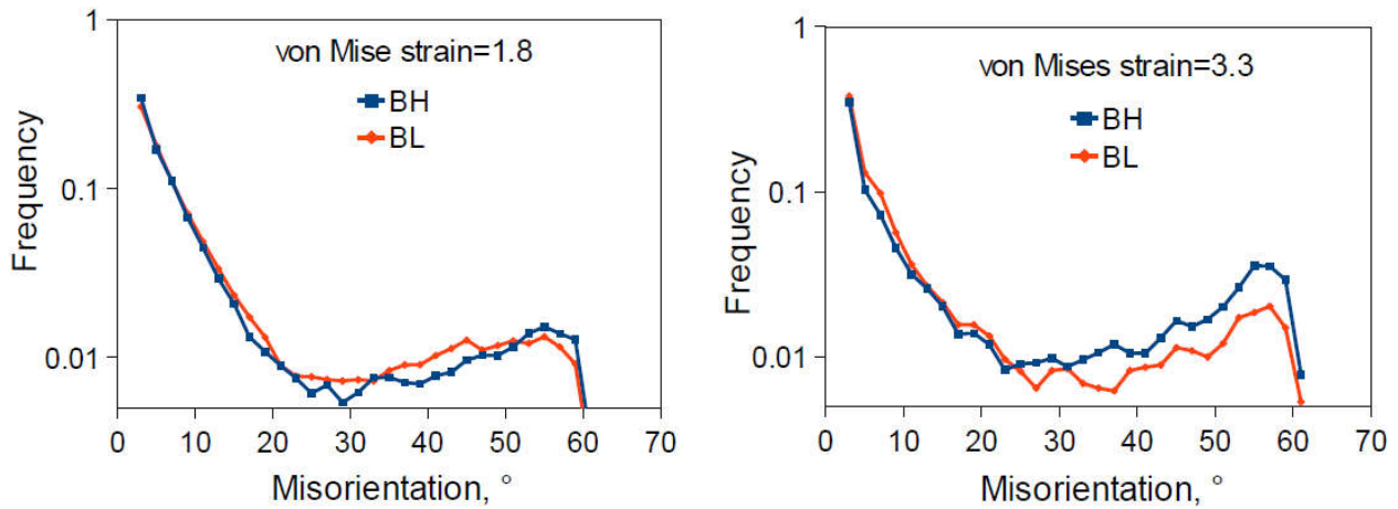
Fig.2 The frequency distributions of the boundary misorientation.
