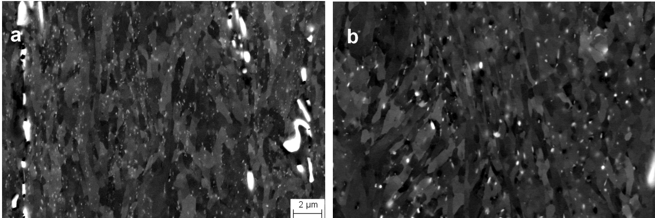
Fig.1 SEM backscattered electron images of subgrain structure and dispersoids at a strain of 1.8 (at the same magnification): (a) BH, (b) BL .
