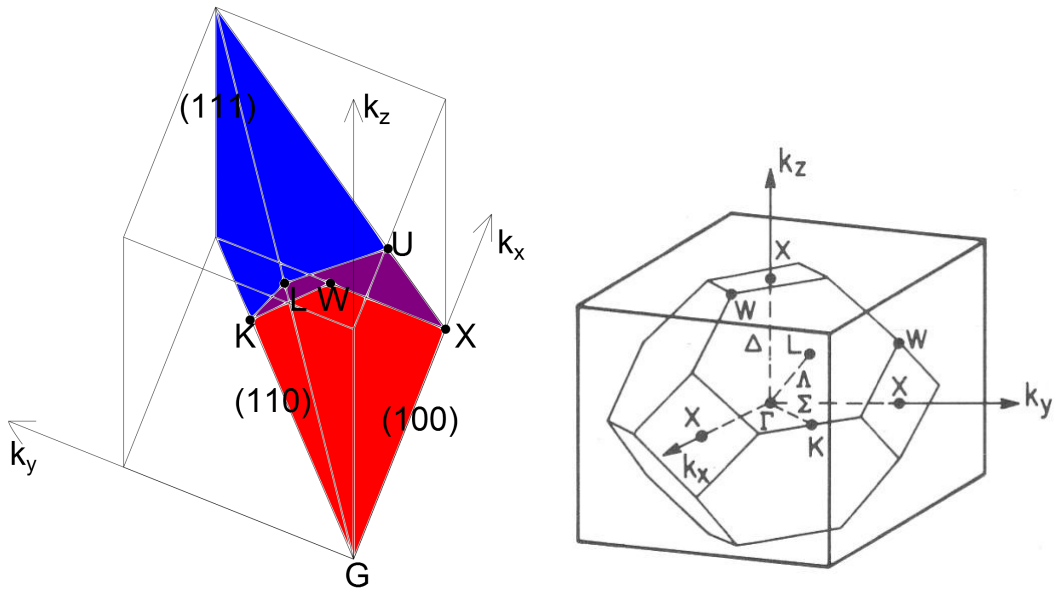
Figure 4: Left side: 1/48 wedge of the 1BZ. Red is actually inside 1BZ, blue is outside 1BZ, and purple is the 1BZ edge. Right The complete 1BZ for a general FCC structure such as zinblende.
