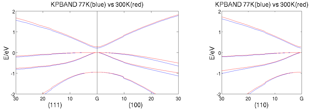
Figure 2: Comparison of close to \Gamma -point band structures in (100)-, (110)- and (111)-direction using KP BAND. X-axis values given in 1/\text{mm}
