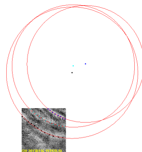
Figure 4.8: Airglow image with fitted circles and their epicentre at 16.jan 2013
