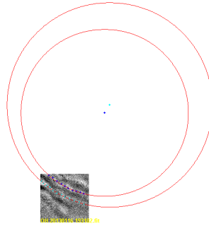
Figure 4.11: Airglow image with fitted circles and their epicentre at 16.jan 2013
