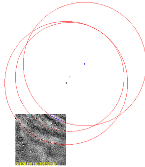
Figure 4.7: Airglow image with fitted circles and their epicentre at 16.jan 2013
