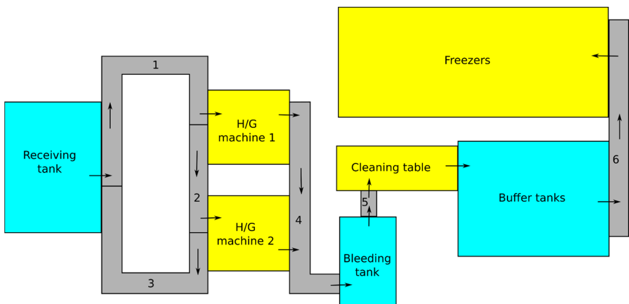
Figure 16: A possible "real-world" layout of the processing line we will simulate.
