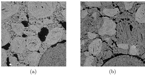
Figure 5: Zoom-in on anode cracks (a) Anode B. (b) Anode C.
