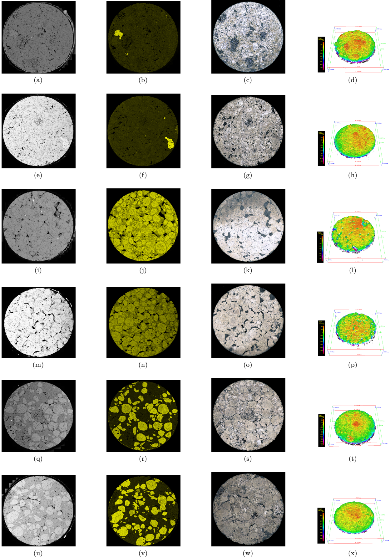
Figure 6: Anode A, parallel 1 ((a)-(d)) and parallel 2 ((e)-(h)). Anode B, parallel 1 ((i)-(l)) and parallel 2 ((m)-(p)). Anode C, parallel 1 ((q)-(t)) and parallel 2 ((u)-(x)). (a), (e), (i), (m), (q) and (u) are SEM surface maps. The pictures are stitched together of over 400 single pictures. (b), (f), (j), (n), (r) and (v)
