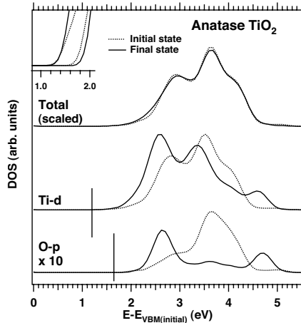
FIG. 2. Total (for the entire unit cell with s , p , and d electrons) and partial (projected on an atom with particular orbital character) density of states for anatase \text{TiO}_2 obtained by ab initio calculations. The energy scale is relative to the valence-band maximum of the initial state. Dashed lines: DOS curves for the initial state. Solid lines: DOS curves for the final state with an O 1s core hole present. The total density of states is scaled in order to facilitate a comparison. As indicated, the O- p DOS is comparable to the Ti- d DOS if divided by a factor of ten. The Ti- d and O- 2p onsets of the final states are marked with vertical solid lines. The inset shows a magnified view of the different Ti- d and O- 2p onsets for anatase.
