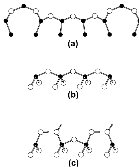
Figure 6. Schematic illustrations of the (4 × 1) reconstructed anatase TiO 2 (001) surface before and after hydroxylation. The atomic structures are based on the ADM model. 18 (a) The clean reconstructed surface projected along the [100] direction. (b) Illustration of how the ridges extend along the [010] direction. (c) Hydroxylation of the ridge Ti sites as proposed in ref 20. This corresponds to phase 1 in the present study.
