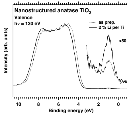
FIG. 4. Valence-band electronic states for an in situ prepared film of anatase \text{TiO}_2 nanoparticles before (dotted line) and after (solid line) insertion of 2% Li per Ti ion. The binding-energy scale is referenced to the sample holder Fermi level. The addition induces an increase in the intensity of the Ti 3d related band-gap state and a positive binding-energy shift of the valence band.
