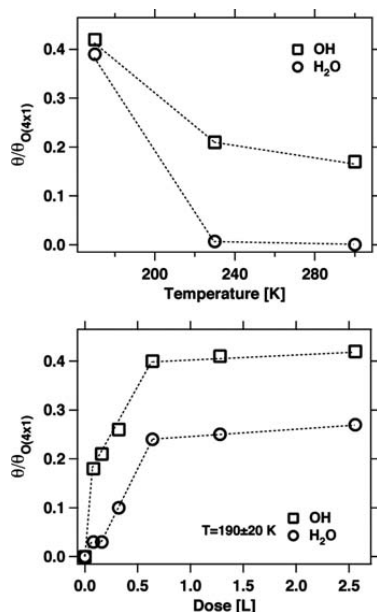
Figure 4. Summary of the quantitative results obtained from the O 1s spectra shown in Figure 1. The plots show the OH and H 2 O coverages as a function of temperature (top) and water dose at 190 ± 20 K (bottom). The coverages are given relative to the number of bridging surface oxygen atoms within the (4 × 1) unit cell.
