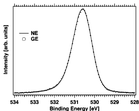
Figure 3. O 1s spectra for the pristine anatase \text{TiO}_2(001)-(4 \times 1) surface recorded in normal (NE, - ) and grazing (GE, \circ ) emission. A Shirley background has been subtracted in both spectra to facilitate the comparison.
