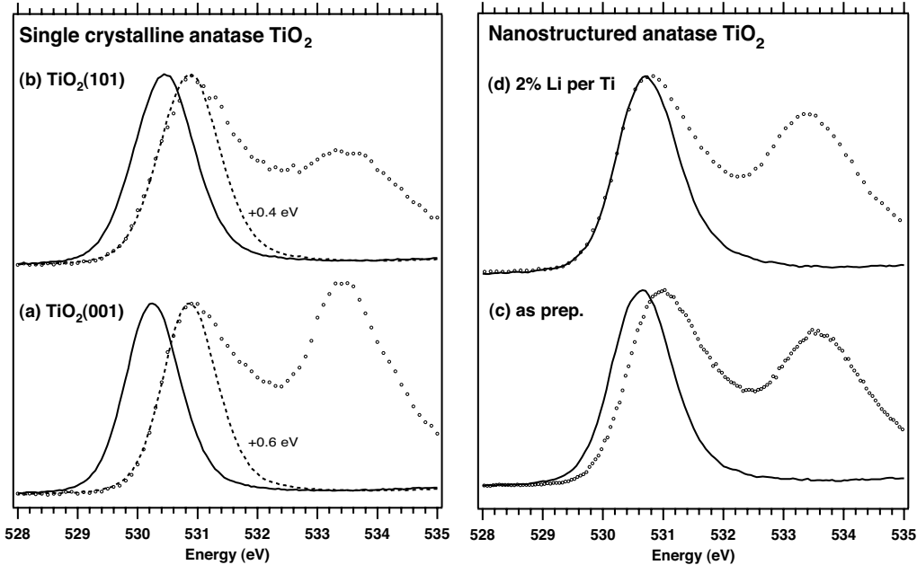
FIG. 3. O 1s XAS and PES spectra for anatase (a) \text{TiO}_2(001) -(4x1) and (b) \text{TiO}_2(101) -(1x1) on a common energy scale. The energy values of the PES spectra are relative to the Fermi level, whereas the energy values of the XAS spectra correspond to the absolute photon energy. The spectra are normalized as to have the same peak height. A clear separation between the XAS and PES peaks are observed for both surfaces with a smaller separation noted for the (101) surface. (c) The same comparison for an as-prepared nanostructured anatase film also reveals an XAS-PES separation. As shown in (d), this offset can be eliminated by the insertion of small amounts of lithium.
