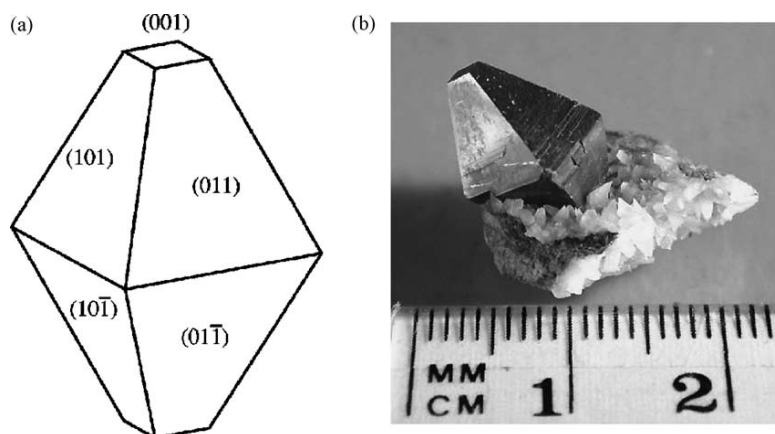
Figure 3.1: (a) The calculated equilibrium shape of an anatase \text{TiO}_2 crystal [19]. (b) Picture of an anatase mineral crystal. The figure is taken from [6].
