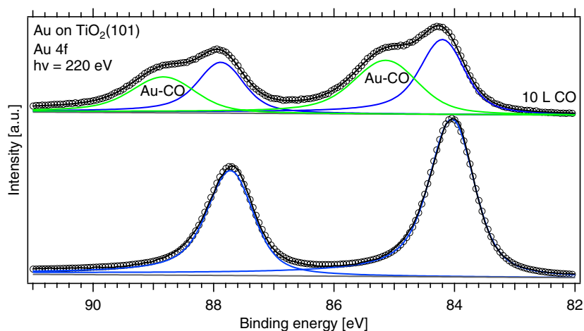
Figure 2.11: Au 4f photoemission spectra for the anatase \text{TiO}_2(101) surface with 0.5 ML Au evaporated on top, before (lower spectrum) and after (upper spectrum) adsorption of 10 L CO. The chemical shifted peaks (green curves) are due to Au atoms directly bonded to CO.
