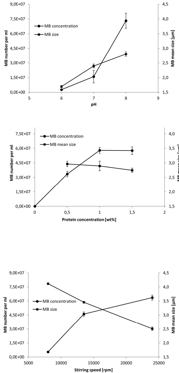
Fig. 8. Mean MB concentration and mean MB diameter as a function of (a) pH, (b) albumin concentration and (c) stirring speed during preparation. Standard settings were: NP concentration: 1% (w/v); BSA concentration: 1% (w/v); Stirring speed: 20,500 rpm; pH: 7.5. The error bars represent standard deviation of mean MB size and distribution from three MB batches.
