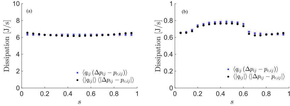
FIG. 9. The dissipation \langle q_{ij} (\Delta p_{ij} - p_{c,ij}) \rangle and \langle |q| \rangle \langle |\Delta p - p_{c,ij}| \rangle plotted against the non-wetting saturation for (a) Ca = 0.1 and (b) Ca = 0.01 . Equation (25) predicts that the two data sets should be equal. The syste size was 20 \times 20 .
