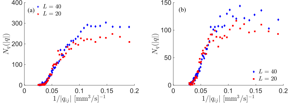
FIG. 4. Histogram N_q(|q|) of volume flow in links when 0.4 < s_{ij} < 0.5 and 0.2 \text{ mm} < r_{0,ij} < 0.3 \text{ mm} for Ca = 0.1 and (a) s = 0.3 or (b) s = 0.4 .
