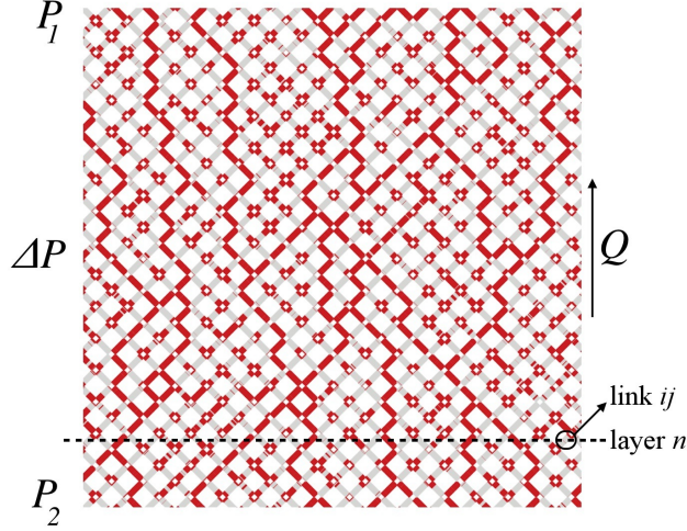
FIG. 1. Our network model, which is described in detail in the Appendix, consists of a square lattice oriented at 45^\circ with respect to the vertical direction, see arrow. The network is periodic both in the vertical and horizontal directions. Hence, fluids that leave the network along the upper border, reappear at the bottom border and fluids that leave along the left border enters at the right border and vice versa. The links are filled with an immiscible mixture of wetting (white) and non-wetting (red) fluids. A pressure difference \Delta P = P_1 - P_2 between the upper and lower borders drives the flow Q in the vertical direction. The non-wetting fluids forms channels that span the network once the flow has reached steady state as shown in the figure. Steady state flow means that the average flow parameters such as Q fluctuate around well-defined constant average values, whereas at the level of the links, the interfaces between the immiscible fluids move resulting in fluid clusters constantly merging and breaking up.
