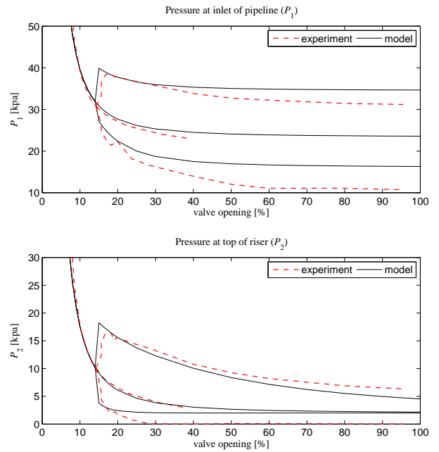
Fig. 6. Bifurcation diagrams of simplified model (solid) compared to experiments (dashed)
