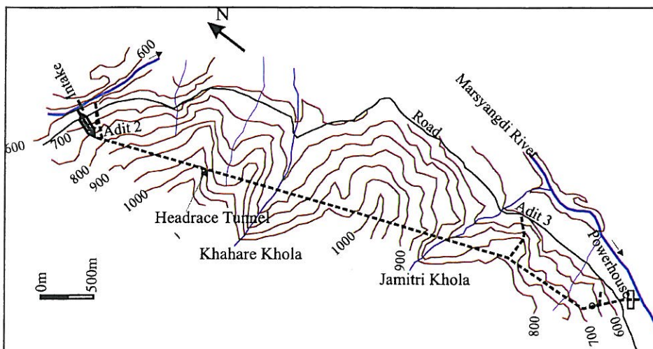
Figure 1. Project Layout (based on MMHEP, NEA)
