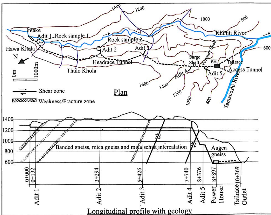
Figure 2a. Geological Section - Khimti I Hydropower Project (Panthi 2006).
