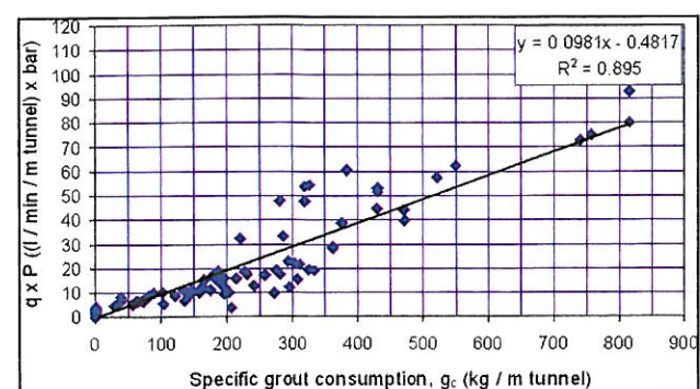
Figure 6c. Specific Grout Consumption at Khimti Headrace Tunnel (Panthi 2006).
