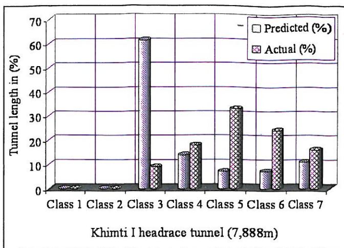
Figure 2b. Observed and Predicted Rock Mass Quality along the Headrace Tunnel in Khimti-I (Panthi 2006).
