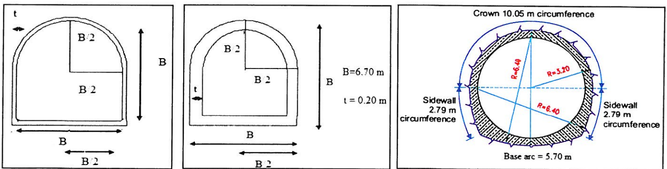
Figure 4. Proposed shotcrete lined and concrete lined sections (left and middle) and existing concrete lined section (right)
