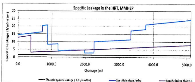
Figure 7a. Specific Leakage at HRT, MMHEP.
