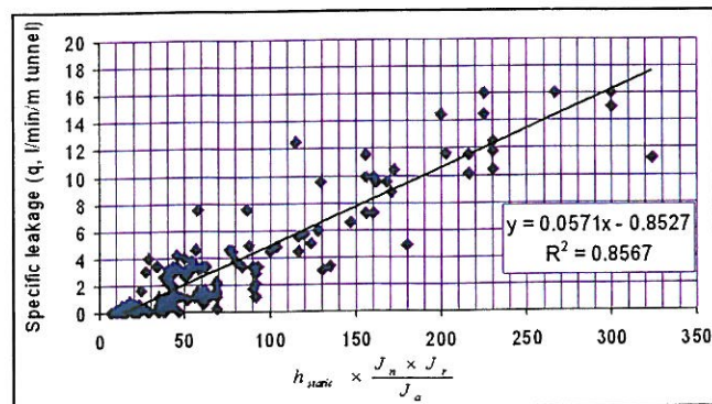
Figure 6b. Correlation of Specific Leakage to Joint Parameter and hstatic (Panthi 2006).
