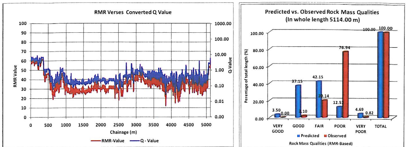
Figure 3. Geological Section and Observed and Predicted Rock Mass Quality along the Headrace Tunnel in MMHEP (Shrestha 2009)
