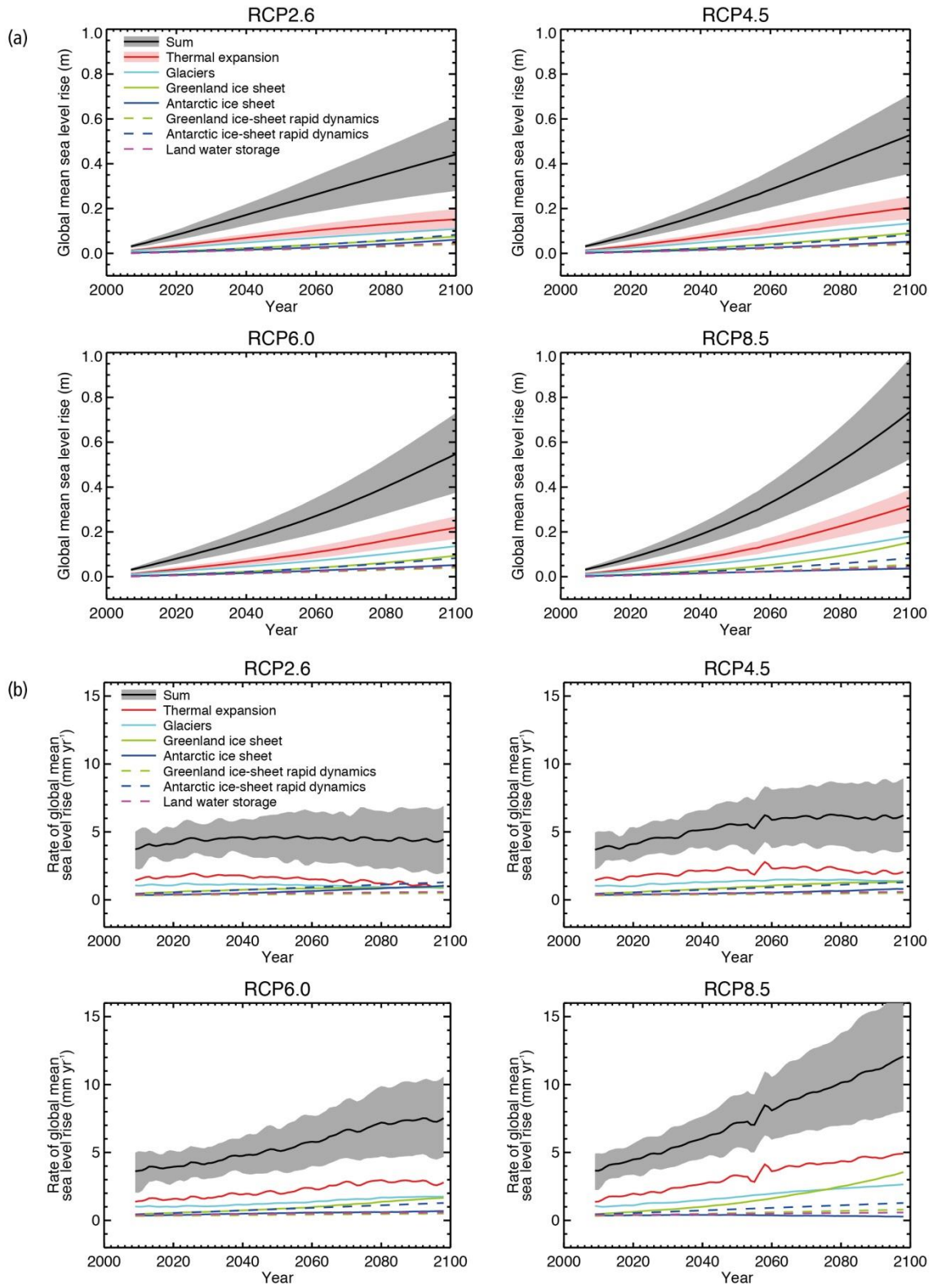
Figure 4-1 Data from IPCC
