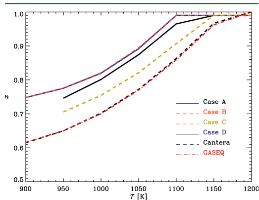
Figure 7. Conversion as a function of the temperature for different cases and two different equilibrium solvers.
