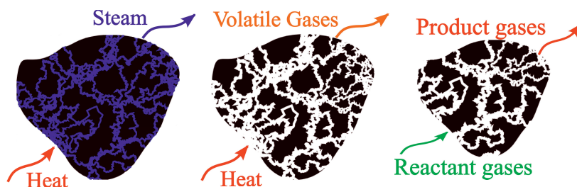
Figure 1.4: Coal combustion processes. From left to right: Drying, devolatilization/pyrolysis, combustion/gasification
