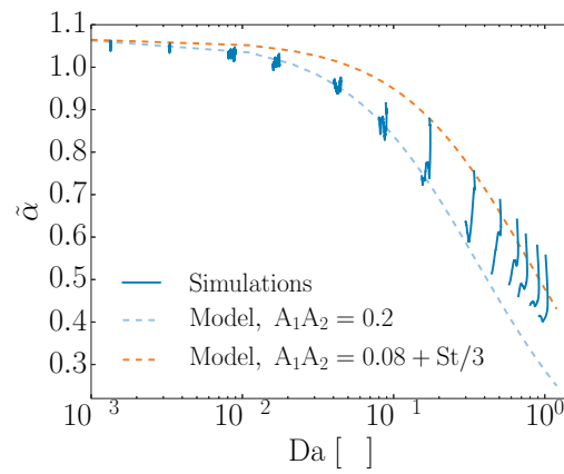
Figure 3.6: Mean mass loss rate normalized by the ideal mass loss rate assuming perfectly mixed fluid as a function of the Damköhler number. The dashed lines show the model from the previous work [75], with a fitting value obtained from the work of Haugen et al. [54] and a value of 0.2.
