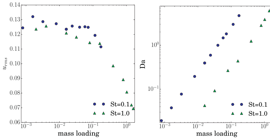
Fig. 6. Root mean square of velocity and Damköhler number as function of mass loading M_l = M_p/M_f for two different Stokes numbers.
