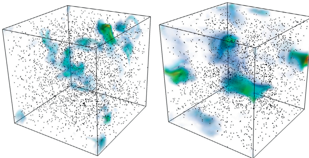
Fig. 4. 3D plot of the domain with every 300th particle and the 90th percentile of the reactant concentration: St = 0.1 (left) and St = 1.0 (right).
