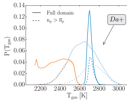
Figure 16: PDF of the domain temperature for cases with three different Da . The dashed line represents the subset of the domain where n_p > \bar{n}_p .
