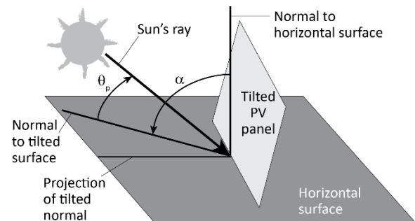
Fig.2 Angles of tilted surface [7]
