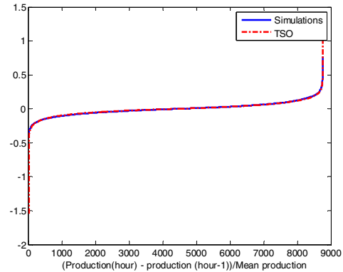
Fig.6 Delta production for the wind power production in DK for the COSMO simulated results (blue curve) and the TSO data sorted (red curve).
