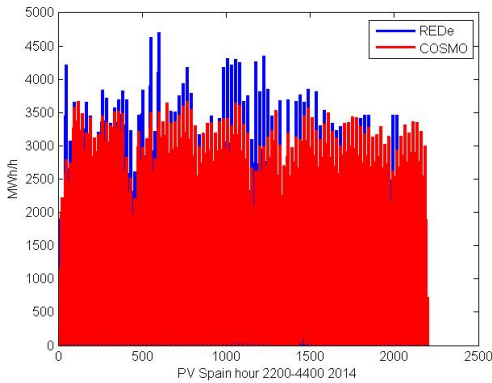
Fig.5 PV power production for ES hour 2200-4400 2014
