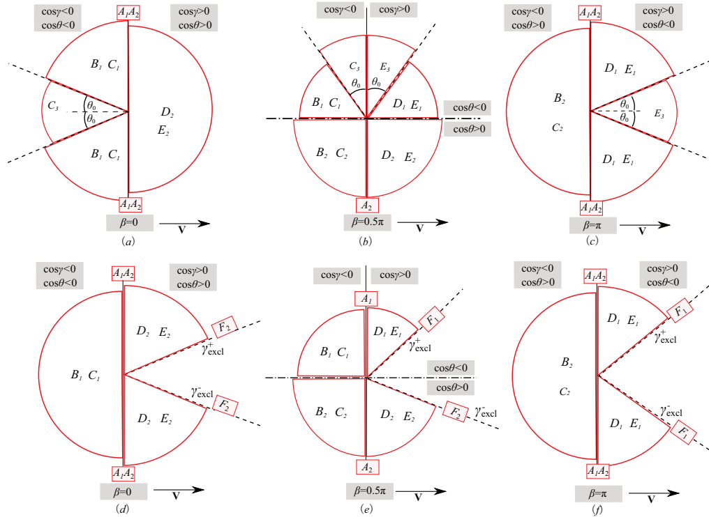
FIGURE 6. Examples showing different far-field waves occurring in different sectors of the \gamma plane for \beta = 0 (a,d), \beta = \pi/2 (b,e) and \beta = \pi (c,f). Above (a-c): \tau < \tau_{\text{Res,min}} and \omega_0 < S . A cutoff sector of total angle 2\theta_0 appears within which there are no A, B or D waves. Below (d-f): \tau > \tau_{\text{Res,min}} and \omega_0 > S . For \tau above the Doppler resonance, no waves exist within a sector of forward directions. In all figures the source's direction of motion, \gamma = 0 , is towards the right. Labels within each sector refer to graphical solutions of the dispersion relation as shown in Fig. 5
