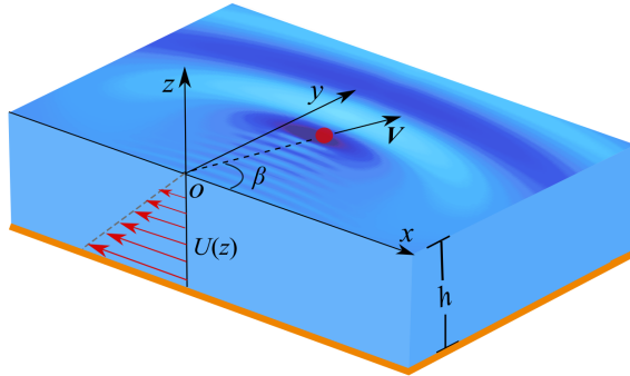
FIGURE 1. Geometry: a surface pressure distribution of oscillating strength travels with velocity \mathbf{V} , making an angle \beta with the \mathbf{x} axis. A depth dependent shear current U(z) = Sz , parallel to the \mathbf{x} axis, is present beneath the surface.
