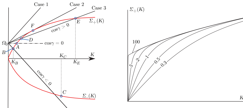
FIGURE 4. a: Graphical solutions of Eq. (3.2) in different situations. See text for discussion and details. b: Behaviour of \Sigma_+(K) as H tends to infinity, when \cos \theta < 0 is assumed ( \text{Fr}_{\text{sb}} \cos \theta = -2 in the figure). Values of H shown as numbers on respective graphs.
