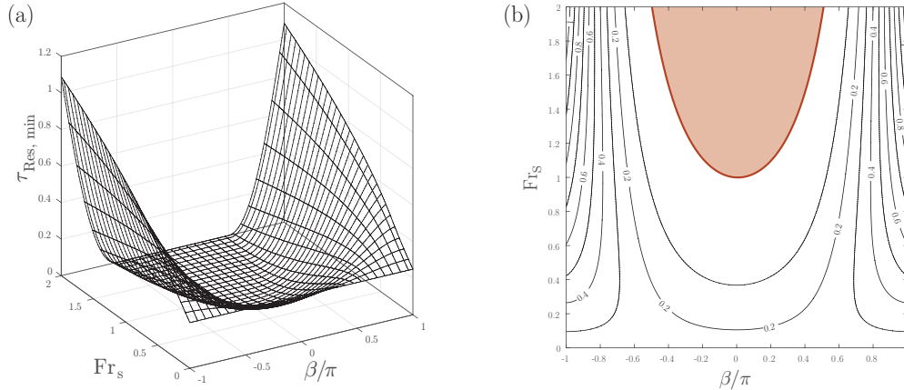
FIGURE 8. Smallest dimensionless resonance frequency \tau_{\text{Res},\min} as a function of \text{Fr}_s and \beta , (a) 3D plot and (b) contour plot. The shaded region satisfies Eq. (4.18), and here \tau_{\text{Res},\min} = 0 .
