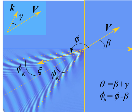
FIGURE 2. Definition of angles. \theta is the angle of the wave vector in the xy coordinate system, \gamma is relative to the sources direction of motion. \phi_\beta is the angle between \mathbf{V} and spatial position \boldsymbol{\xi} in the coordinate system where the disturbance is at rest.
