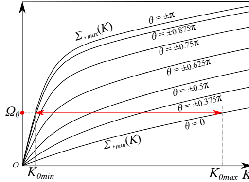
FIGURE 3. Graphical solutions of Eq. (3.2) when V = 0 .
