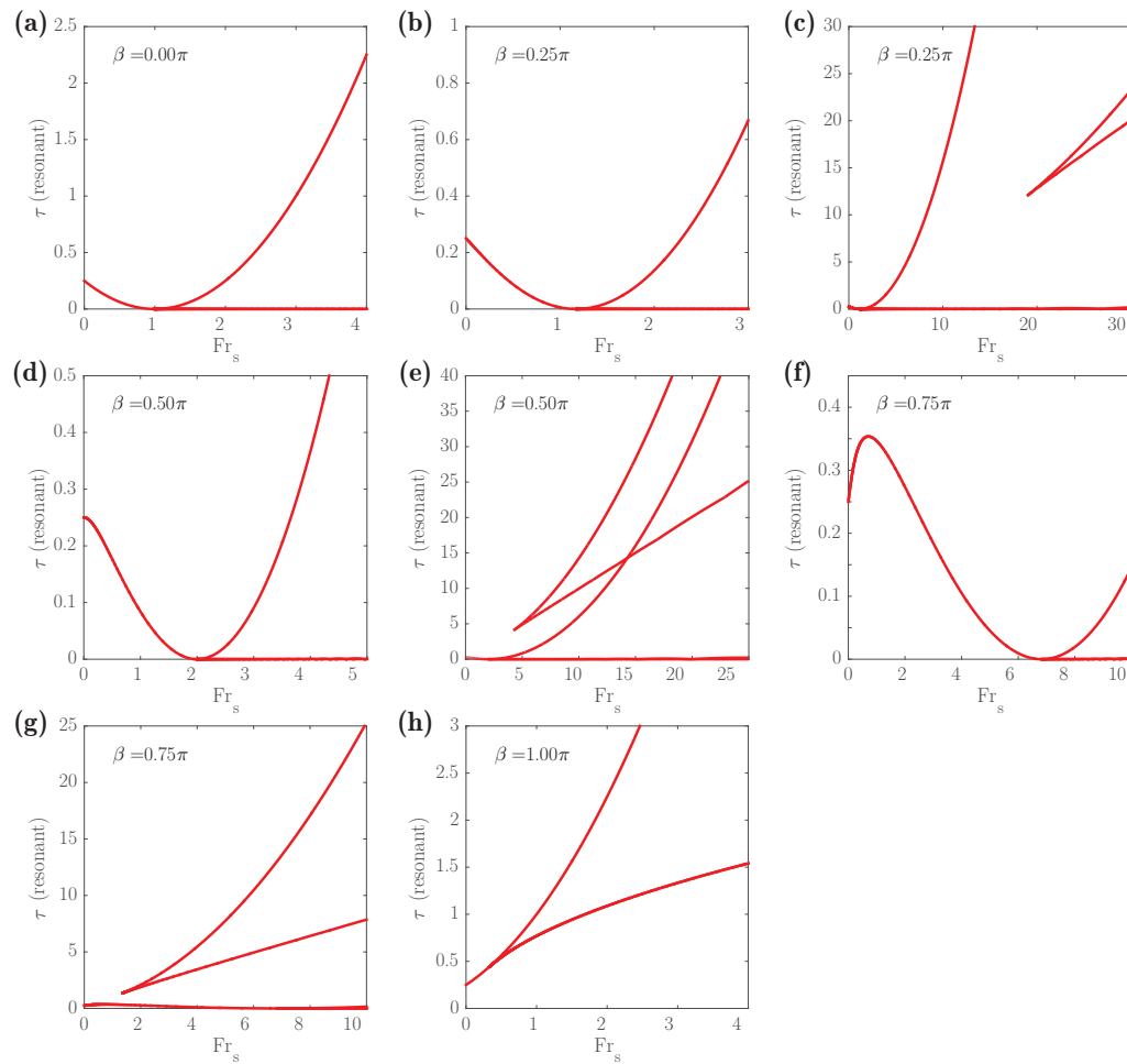
FIGURE 11. Doppler resonant frequencies \tau_{Res} as a function of Fr_s for different directions of motion, \beta . Where two panels show the same \beta (Panels b and c, d and e, and f and g), the first is a zoom of behaviour for small and moderate Fr_s while the second shows the full picture appearing at large Fr_s .
