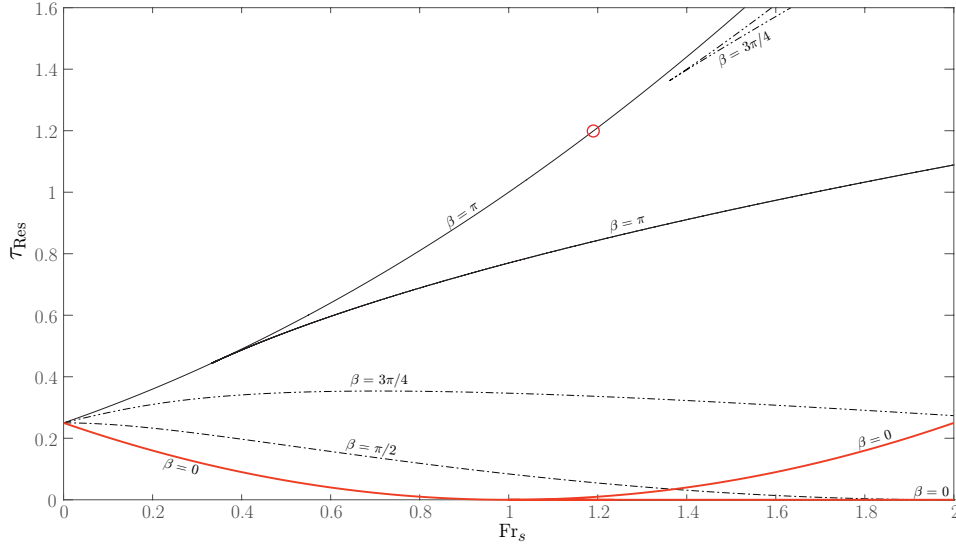
FIGURE 9. Resonance frequencies \tau_{\text{Res}} in different directions of motion \beta for moderate values of \text{Fr}_s . The highest branch of resonant values for \beta = \pm\pi (marked with a circle) corresponds to the 2D result of Tyvand & Lepperød (2015).
