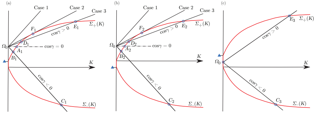
FIGURE 5. Graphical solutions of dispersion relation (3.2) in infinite water depth. Intrinsic frequencies \Sigma_{\pm}(K, \gamma) are the curved lines, K \text{Fr} \cos \gamma are the straight lines. Intersections of the two are wave solutions, marked with circles. The point (0, -\text{Fr}_{\text{sb}} \cos \theta) is marked with a triangle. The panels show situations 0 < -\text{Fr}_{\text{sb}} \cos \theta < \Omega_0 (a), -\text{Fr}_{\text{sb}} \cos \theta < 0 (b), 0 < \Omega_0 < -\text{Fr}_{\text{sb}} \cos \theta (c).
