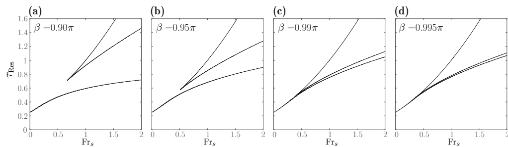
FIGURE 12. Doppler resonant frequencies \tau_{Res} as a function of Fr_s as \beta approaches \pi (or -\pi ).
