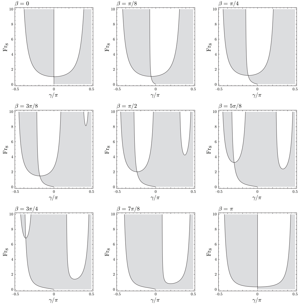
FIGURE 10. Solutions of \Phi'(\gamma) = 0 from Eq. (4.3). Shaded areas indicate \Phi'(\gamma) > 0 . To each solution of \Phi'(\gamma) = 0 (at \gamma = \gamma_{\text{Res}} , say) for a given \text{Fr}_s there exists a corresponding (not necessarily distinct) resonant \tau -value, \tau_{\text{Res}} = \Phi(\gamma_{\text{Res}}) , as plotted in Fig. 11.
