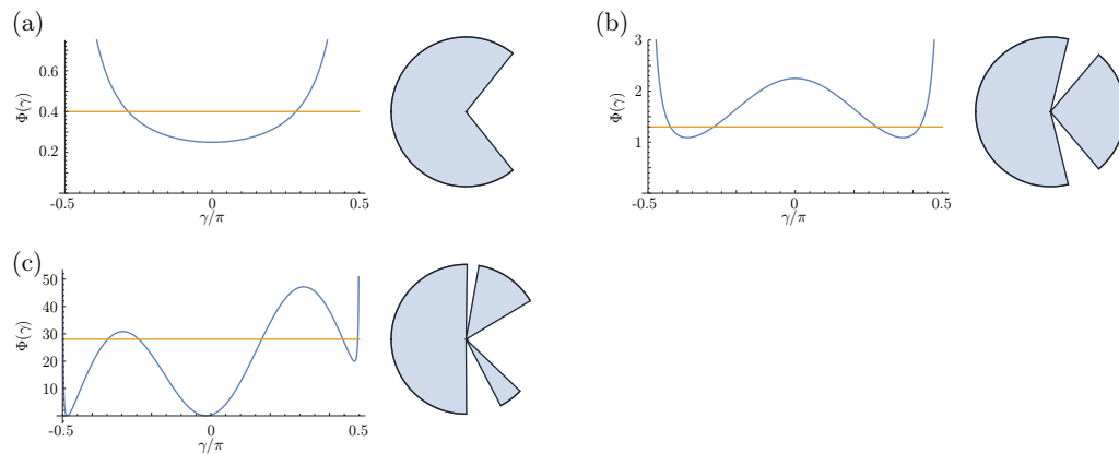
FIGURE 7. Sectors of propagation directions \gamma with no wave solutions. The graphs are plots of \Phi(\gamma) , the horizontal lines show the (arbitrarily chosen) value of \tau ; sectors where \Phi(\gamma) < \tau are excluded. Pie charts next to each graph illustrate excluded sectors (included sectors are shaded). We show in Section 4.5.2 that a resonant value of \tau is associated with each local maximum or minimum of \Phi(\gamma) ; if \Phi(\gamma) has a local extremum at \gamma_{\text{Res}} , then \tau_{\text{Res}} = \Phi(\gamma_{\text{Res}}) . (a) The case without shear, \text{Fr}_s = 0 , \tau = 0.4 . (b) Moderate case with two excluded sectors, \text{Fr}_s = 2 , \beta = \pi , \tau = 1.3 . (c) Extreme case with three excluded sectors, \text{Fr}_s = 20 , \beta = \pi/2 , \tau = 28 .
