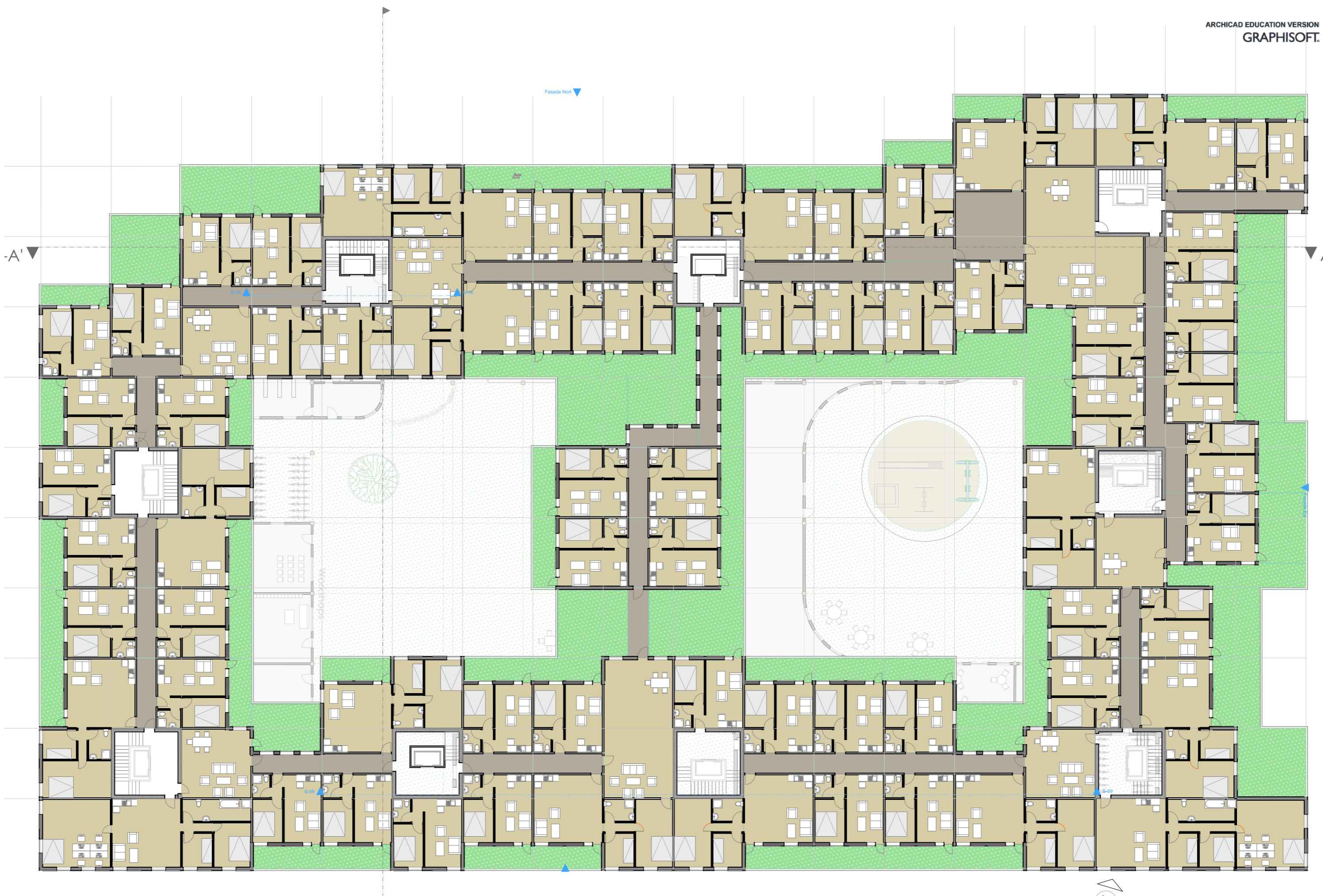
Plan Second floor
