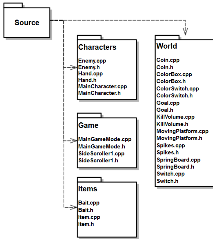
Figure 8.2: The folder structure of the source files
