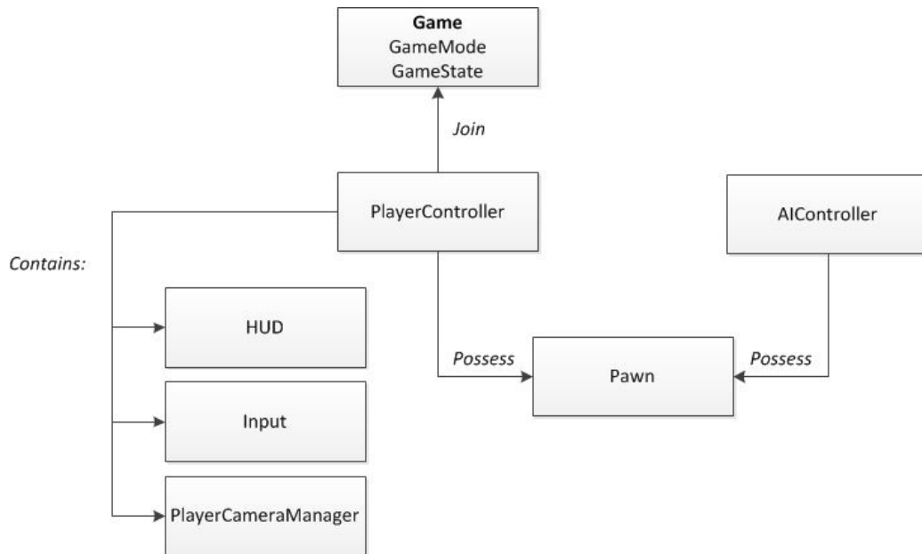
Figure 8.1: The relationship between the game framework classes [66]
