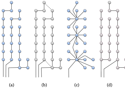
Figure 3.2: Four example clustering designs [Zhao et al., 2006].
