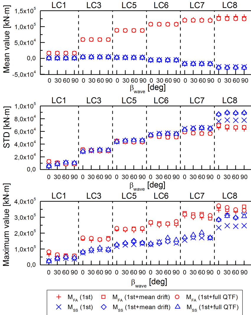
Figure 5.11: Mean value, standard deviation and maximum value of the tower base fore-aft bending moment M_{FA} and side-side bending moment M_{SS} as a function of wave direction \beta_{wave} for all load cases [60].
