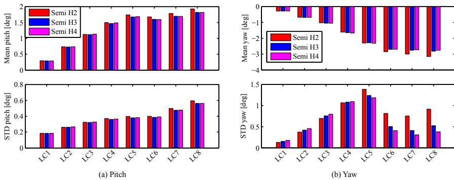
Figure 5.2: The mean value and standard deviation of the pitch and yaw motions of three floating VAWTs in turbulent wind and irregular wave conditions [23].
