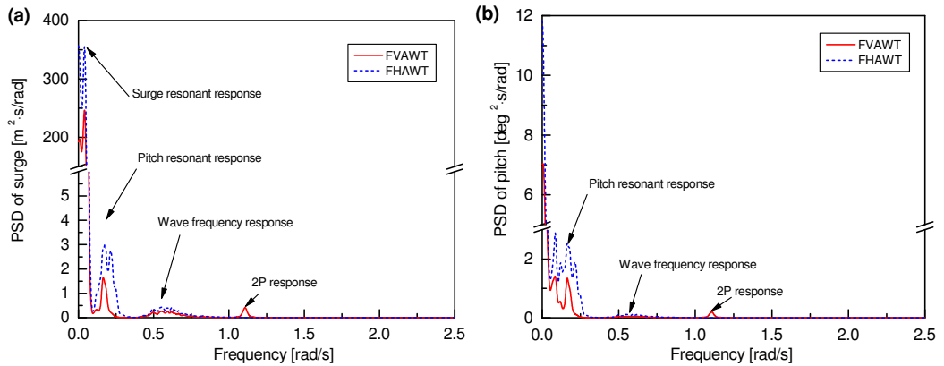
Figure 9: Power spectra of the platform (a) surge and (b) pitch motions for the FHAWT and FVAWT in LC3.3 with U_w=10 m/s.
