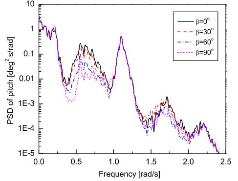
Fig. 6. Power spectra of pitch motions for the semi FVAWT with consideration of full QTF at different wave direction in LC 3.
