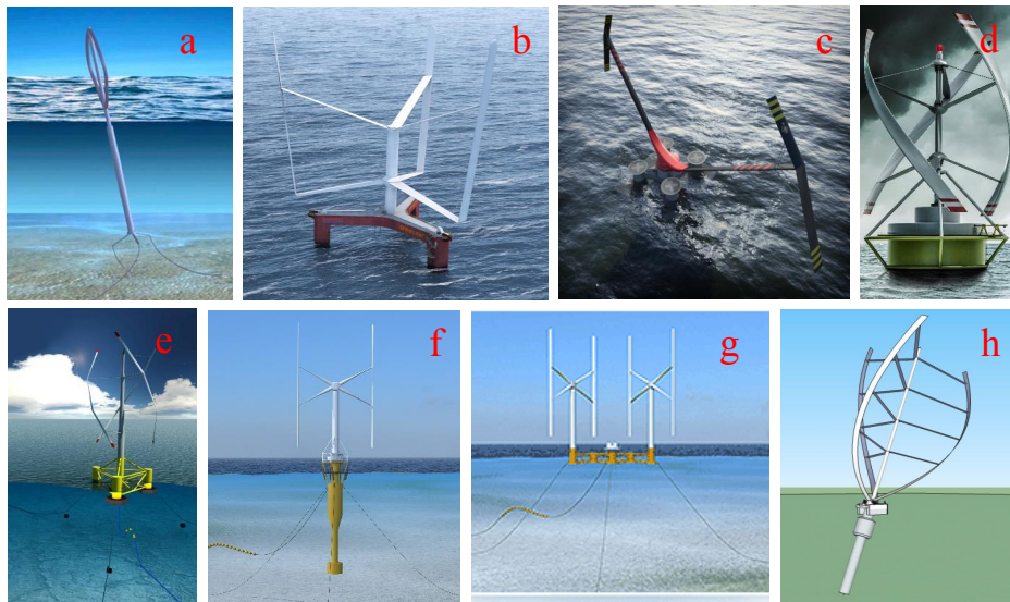
Figure 1.4: Current floating VAWT concepts: (a) DeepWind concept (b) Spinfloater (c) Aerogenerator X (d) Gwind concept (e, f, g) INFLOW concepts (h) floating tilted axis concept, see details in Table 1.1.
