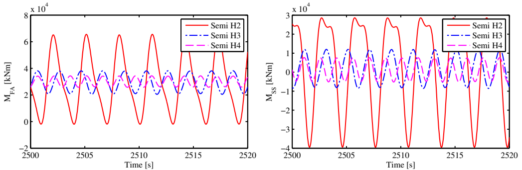
Figure 8: Time history of the tower base fore-aft and side-side bending moments of the three floating VAWTs in the steady wind condition with a wind speed of 10\text{ m/s} .
