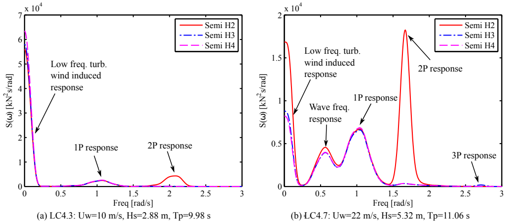
Figure 19: Power spectra of the tension in mooring line 2 of three floating VAWTs in (a) LC4.3 and (b) LC4.7.
