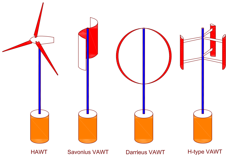
Figure 1.3: Horizontal and vertical axis wind turbines: HAWT, Savonius VAWT, Darrieus VAWT and H-type VAWT
