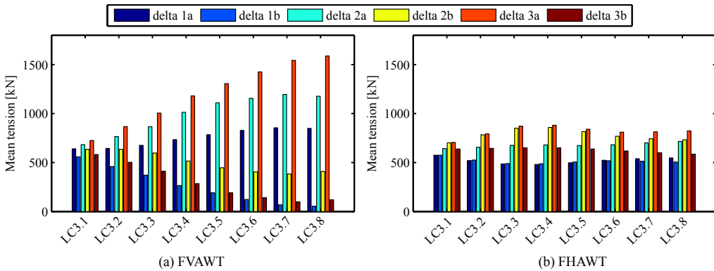
Figure 16: Mean values of the tension in the delta lines for the FFAWT and FVAWT
