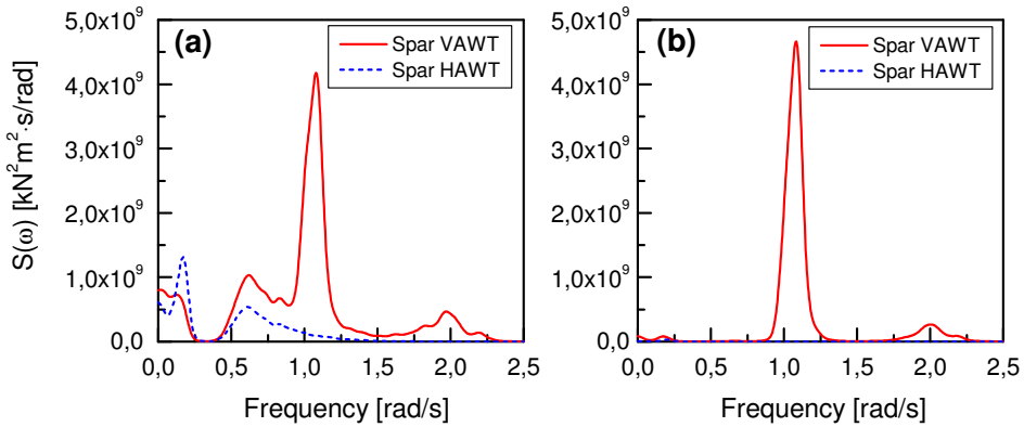
Figure 5.13: Power spectra of the tower base (a) fore-aft bending moment and (b) side-side bending moment for the spar HAWT and VAWT in LC5 with U_w = 14 m/s, H_s = 3.62 m, T_p = 10.29 s [70].
