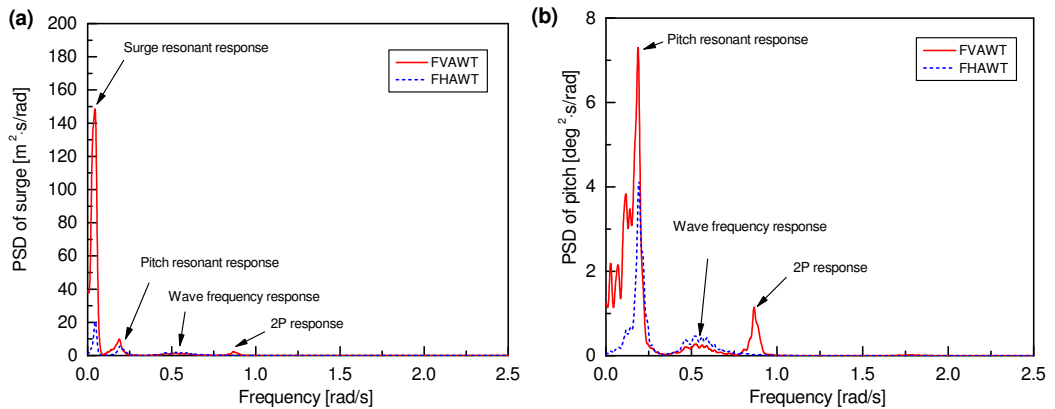
Figure 10: Power spectra of the platform (a) surge and (b) pitch motions for the FHAWT and FVAWT in LC3.7 with U_w=22 m/s.
