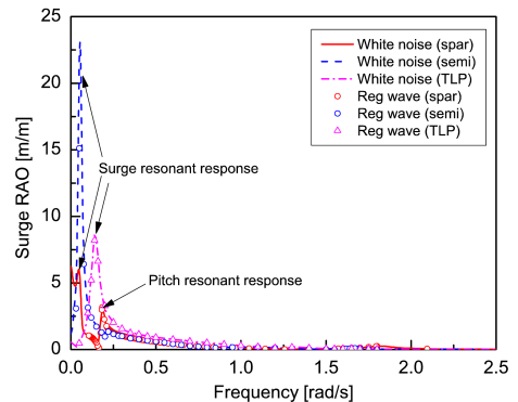
Fig. 3 Surge RAO of the three FVAWT concepts
