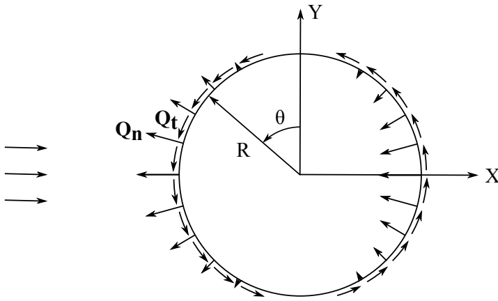
Figure 2: The actuator cylinder flow model representation of a VAWT with volume forces normal and tangential to the circle. Note that the force direction is from the VAWT not the flow. ( Madsen et al., 2013 )
