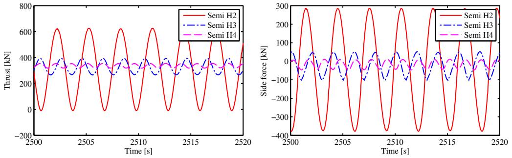
Figure 7: Time history of the thrust and side forces acting on the three floating VAWTs in the steady wind condition with a wind speed of 10\text{ m/s} .
