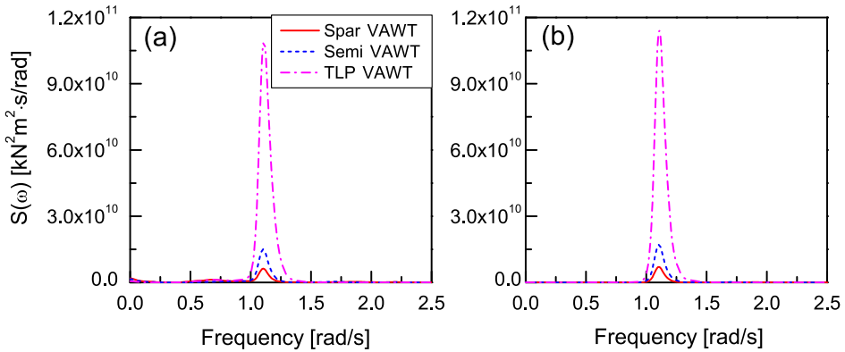
Figure 5.7: Power spectra of tower base (a) fore-aft and (b) side-side bending moment for the three floating VAWT concepts in turbulent wind and irregular wave condition with U_w = 14 m/s, H_s = 3.62 m, T_p = 10.29 s.
