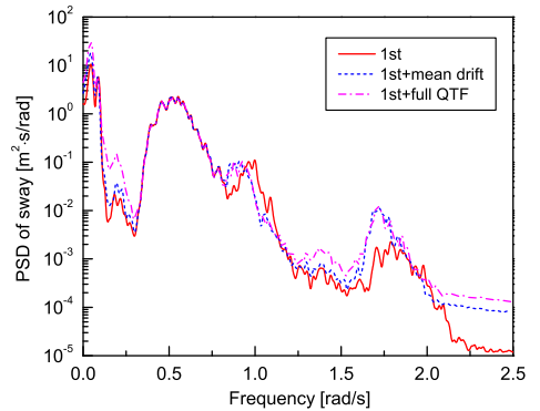
Fig. 8. Power spectra of sway motions for the semi FVAWT with wave direction of 90 degree in LC 6 under different consideration of hydrodynamic loads.
