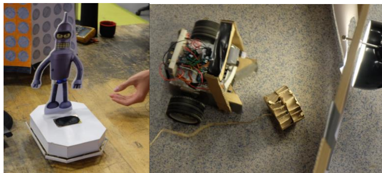
Figure 3. To the left, “Bender”, has incorporated a speaker and microphone with amplifier circuits and interrupt bumpers along three sides. To the right, “the Cleaner”, is returning a puck to its place next to the white wall in a crate.
