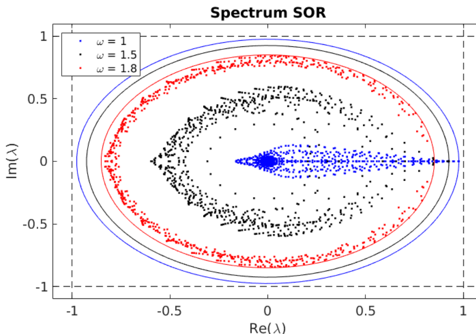
Figure 3.3: Spectrum of the iteration matrix G_{SOR} for different over-relaxation parameters \omega . The solid lines marks the spectral radii. A 20 \times 20 grid was used.
