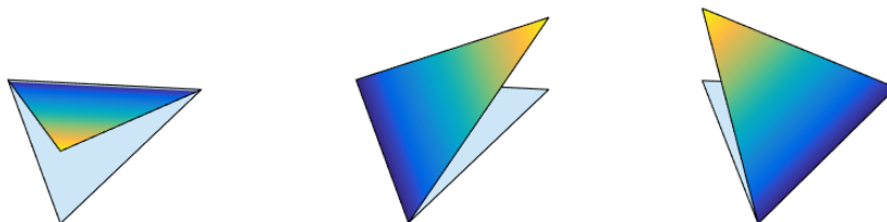
Figure 2.4: Linear nodal basis functions on a triangular element.
