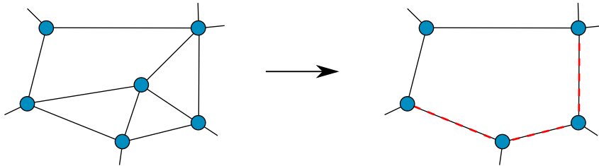
Figure 3.10: One step of the incomplete Cholesky factorization leading to the IC(0) preconditioner. Only already existing couplings are modified, all others are ignored.
