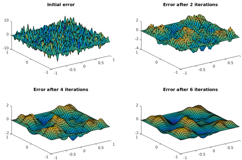
Figure 4.1: Gauss-Seidel smoothing on a normally distributed initial error for Laplace's equation.
