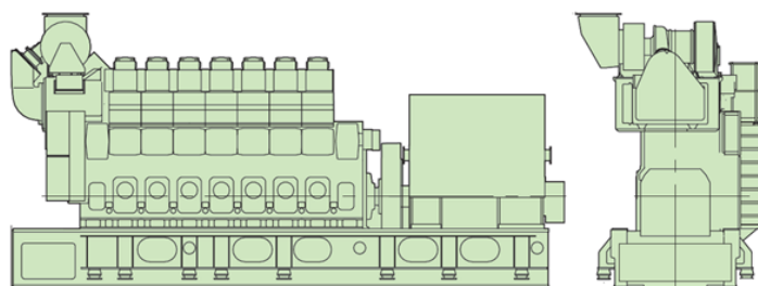
Figure 5.6: MAN Marine Diesel Engine [29]
