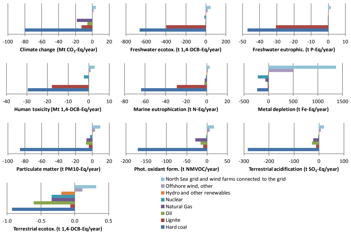
Fig. 3. Net potential environmental burdens (positive axis) or benefits (negative axis) of GDv05 relative to ITD20. The length of the bars represent, for eight power transmission or generation technologies individually, the total indicator results for GDv05 less the corresponding results for ITD20, measured on an average annual basis for an assumed lifetime of 30 years. Ecotox. = Ecotoxicity, Eutropic. = Eutrophication, Phot. oxidant form. = Photochemical oxidant formation.
