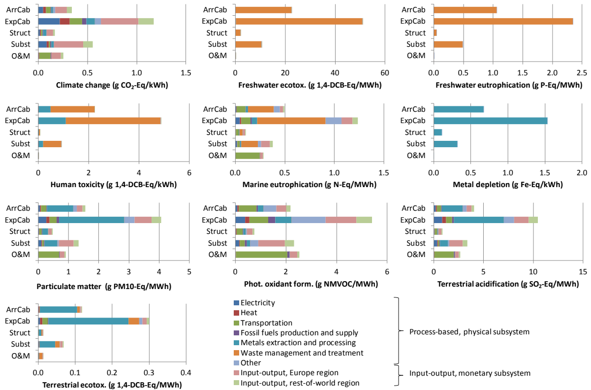
Fig. 2. Impact indicator results by five components and nine stressor sources per kWh or MWh transmitted (GDv05). Ecotox. = Ecotoxicity, Phot. oxidant form. = Photochemical oxidant formation. Components: ArrCab = Array cables, ExpCab = Export cable, Struct = Substructure and topside for substation offshore, Subst = Electrical equipment (voltage source converter, transformer, breakers and switchgear) for substations offshore and onshore, O&M = Operations and maintenance.
