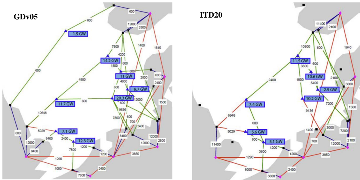
Fig. 1. Schematic representations of North Sea grids in GDv05 and ITD20 for the year 2030. Red lines represent existing transmission capabilities; blue (onshore) and green (offshore) lines are new or upgraded links. Transmission capabilities for each line are shown in units of MW. Nominal outputs of offshore wind park clusters are given in blue rectangles (clusters comprise multiple wind parks). Source: adapted from Huertas-Hernando et al. (2011).
