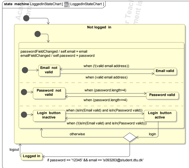
Figure 6.18: Login statechart.
