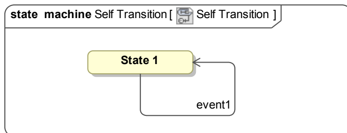
Figure 4.9: Self-transition
