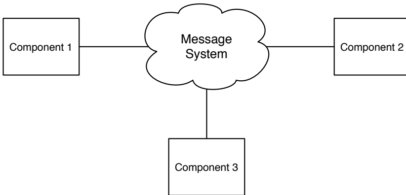
Figure 4.1: Messaging system
