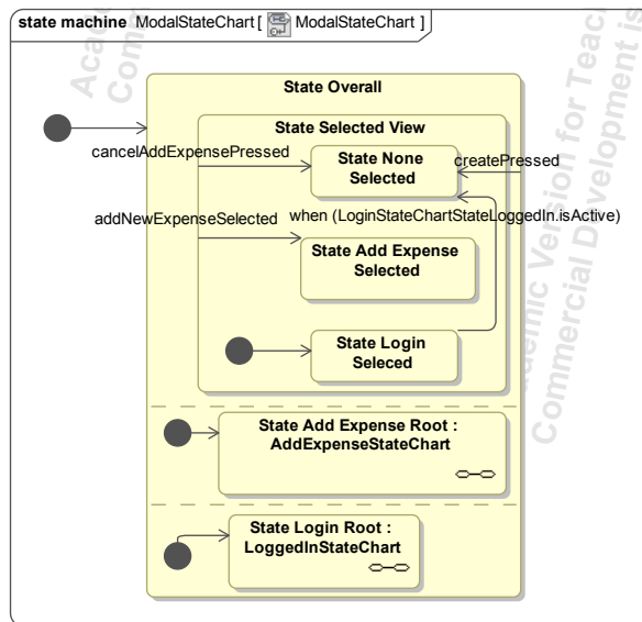
Figure 6.16: Modal statechart.
