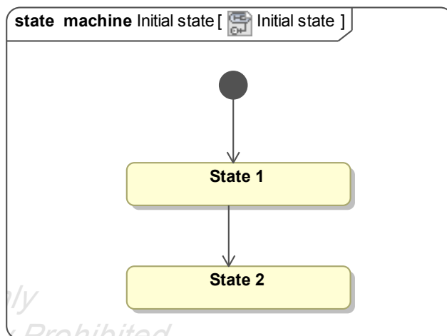
Figure 4.11: Initial transition
