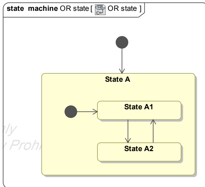
Figure 4.12: OR state
