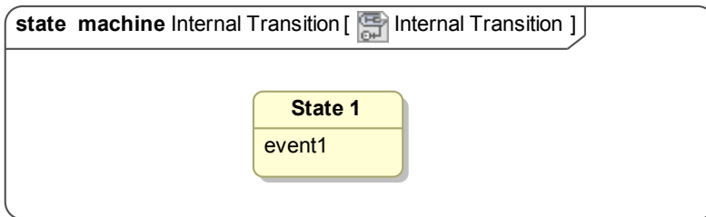
Figure 4.10: Internal transition
