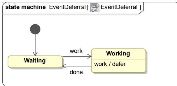
Figure 4.19: Event deferral
