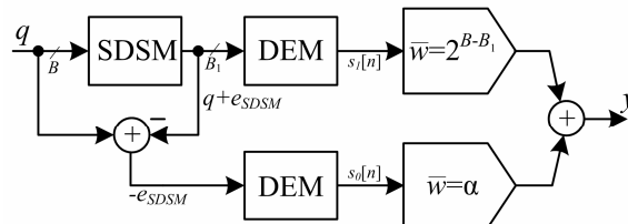
Figure 61: DEM and DAC segmentation with SDSM
