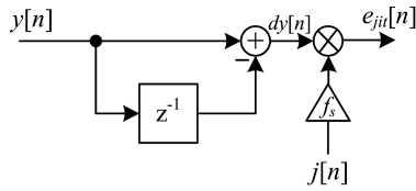
Figure 11: Error area model for jitter error simulation
