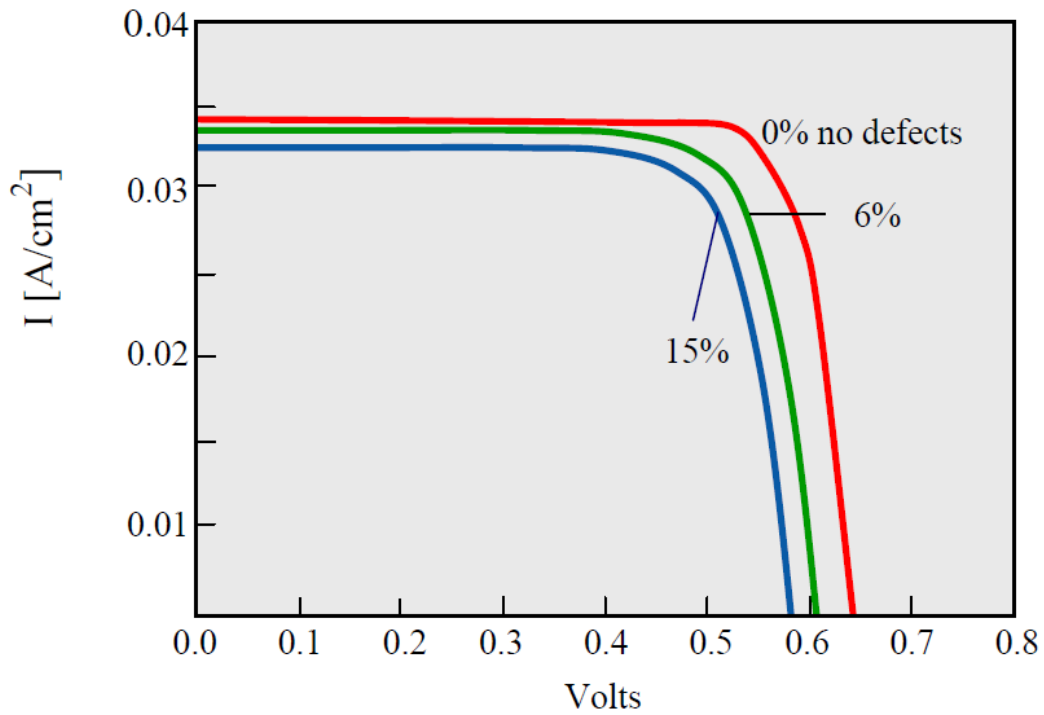
Figure 9: A comparison of calculated I-V characteristics of three cells with 0%, 6%, and 15% of area covered by defects from [13].
