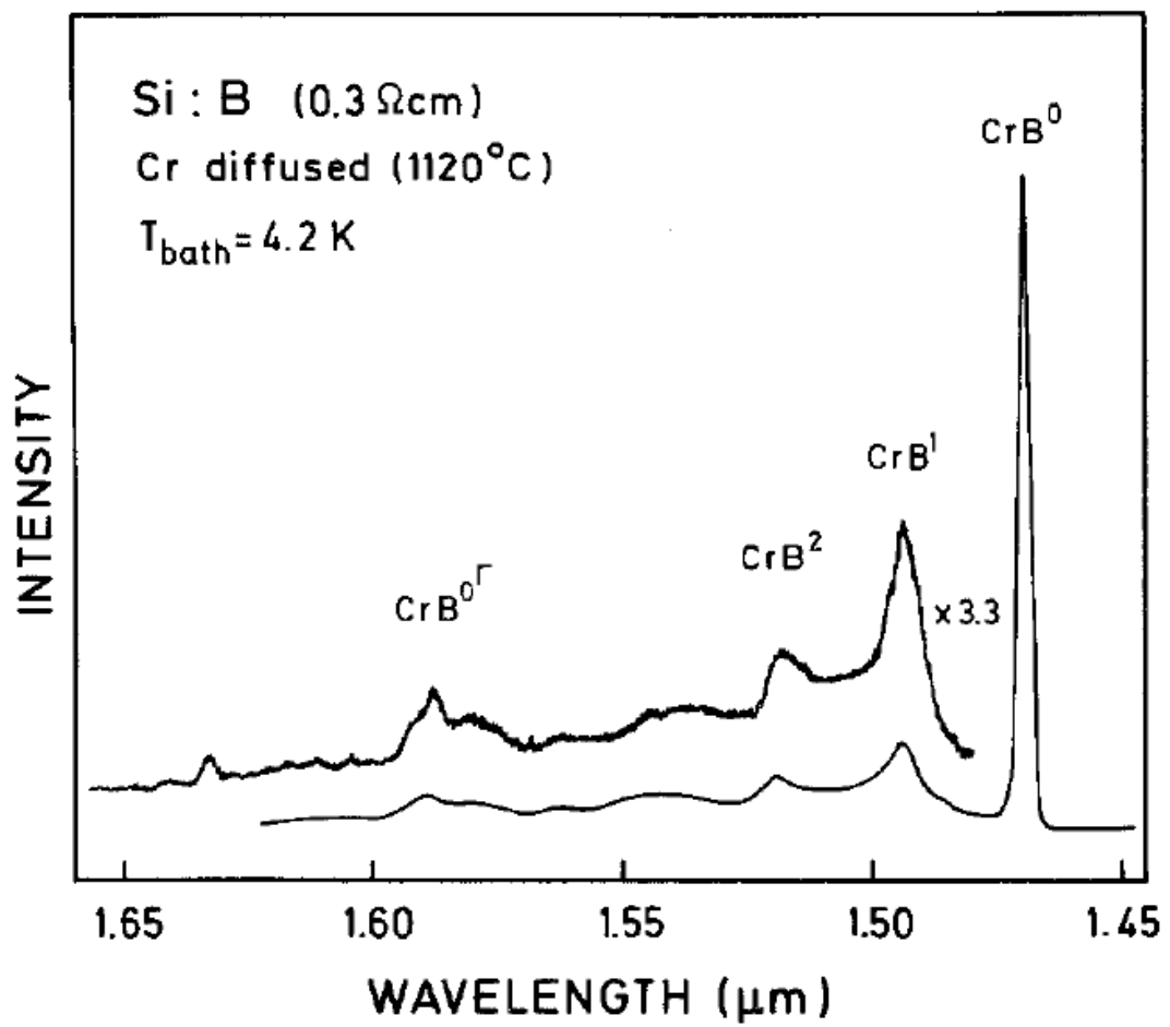
Figure 80: Chromium diffused Boron doped Si sample from [10]
