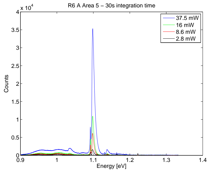
Figure 28: Sample R6-Q3-210 A - pumped with different intensities at 22 K in a defect free area (Area 5 in figure 23). Results are Savitzky-Golay filtered for easier comparison.
