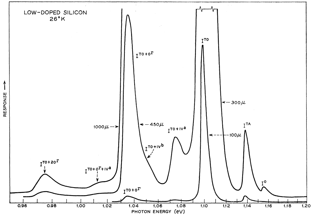
Figure 74: Intrinsic/low doped ( 2 \cdot 10^{14} \text{cm}^{-3} P atoms) Si PL from [6]
