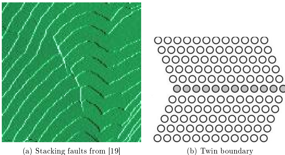
Figure 13: Area defects
