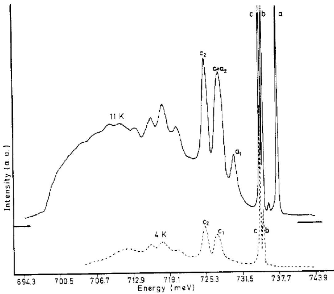
Figure 78: Iron diffused Si sample at two different temperatures from [8]
