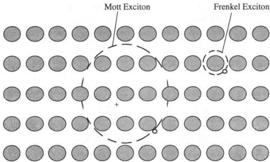
Figure 16: The Mott-Wannier exciton usually free to move together through the crystal, and is weakly bound, with an average electron-hole distance large in comparison with the lattice constant. An ideal Frenkel exciton will travel as a wave throughout the crystal, but the electron is always close to the hole. Figure from [21]
