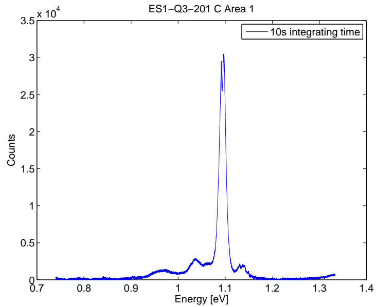
Figure 31: Sample ES1-Q3-201 C pumped with 128 mW at 12 K in a defect free area (Area 1 in figure 29).
