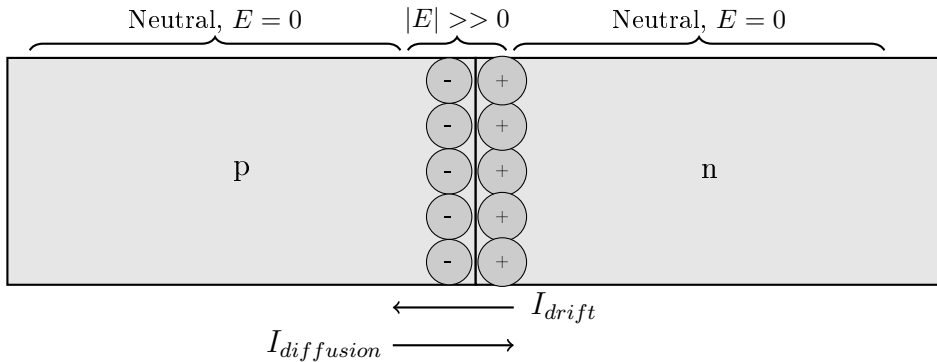
Figure 6: Depletion area
