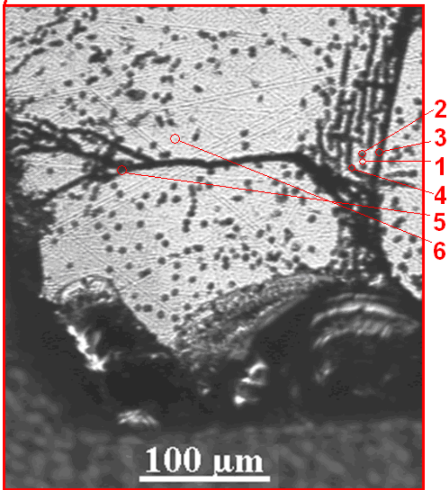
Figure 29: Sample ES1-Q3-201 C 48 - picture taken using light microscope. Marked areas are spots where photoluminescence has been measured.
