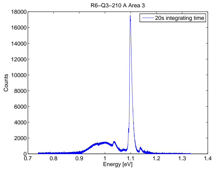
Figure 26: Sample R6-Q3-210 A - pumped with 128 mW at 10 K in a defect free area (Area 3 in figure 23).
