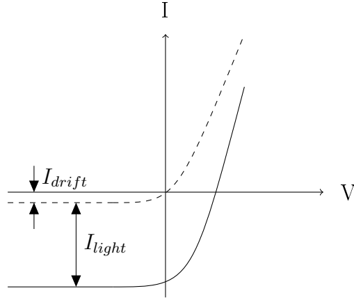
Figure 7: Current-voltage characteristics for a solar cell
