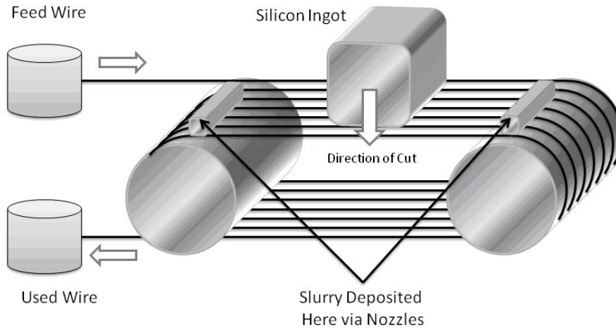
Figure 11: Wafer wire saw (figure from [2])
