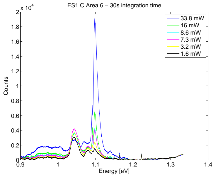
Figure 36: Sample ES1-Q3-201 C pumped with different intensities at 22 K in a grain boundary (Area 6 in figure 29). Results are Savitzky-Golay filtered for easier comparison.
