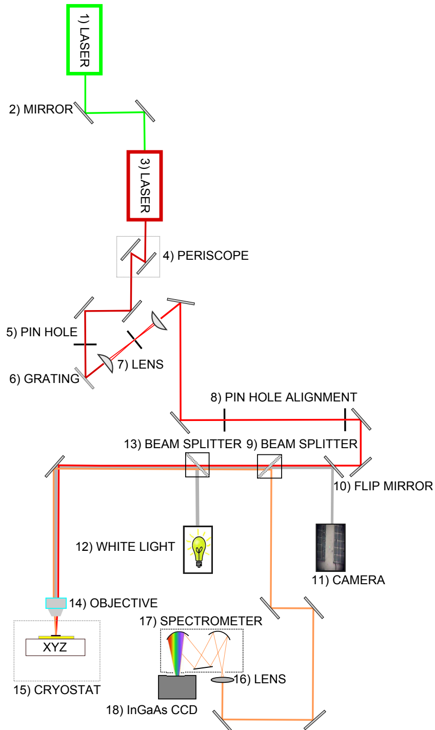
Figure 22: Lab setup
