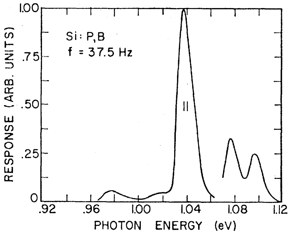
Figure 77: Boron ( 3 \cdot 10^{16} \text{cm}^{-3} ) and phosphorus ( 6 \cdot 10^{16} \text{cm}^{-3} ) doped Si PL specter from [7] at 4.2 K
