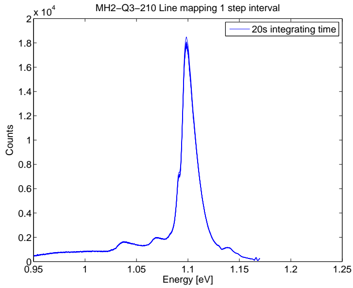
Figure 46: Sample MH2-Q3-210 B2 pumped with 128 mW at 14 K line map using 10 small steps, on line L1 in figure 37.
