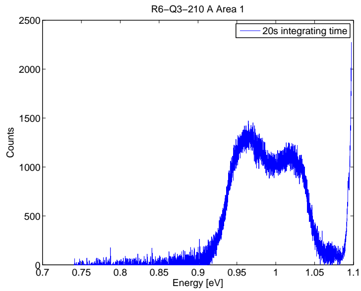
Figure 24: Sample R6-Q3-210 A - pumped with 128 mW at 10 K in a dislocation line (Area 1 in figure 23).
