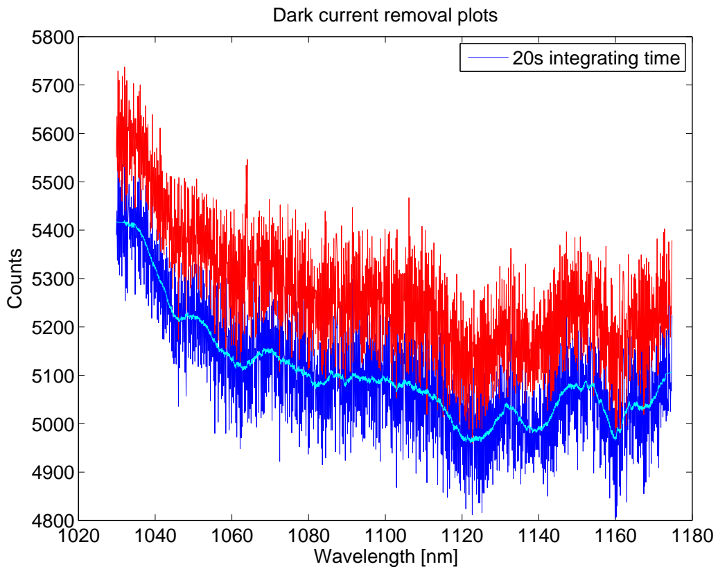
Figure 51: Dark current (blue) and dark current + background noise (red) with Savitzky-Golay filtered noise floor estimation (cyan)
