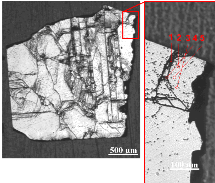
Figure 23: Sample R6-Q3-210 A - picture taken using light microscope. Marked areas are spots where photoluminescence has been measured.
