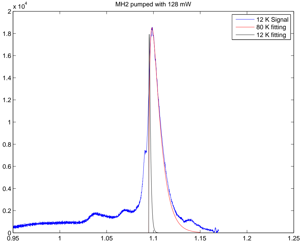
Figure 70: Temperature fitting using equation 25 on MH2 results from line map in figure 46
