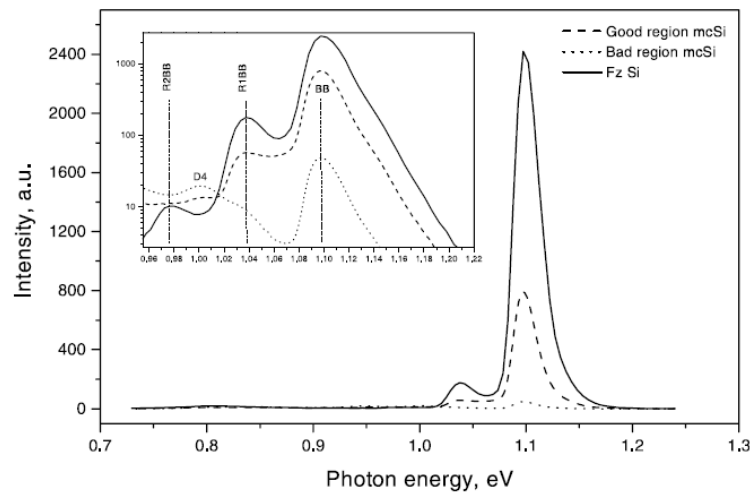
Figure 82: Comparison of the spectra in high and low quality regions of mc-Si with FZ-Si from [12]
