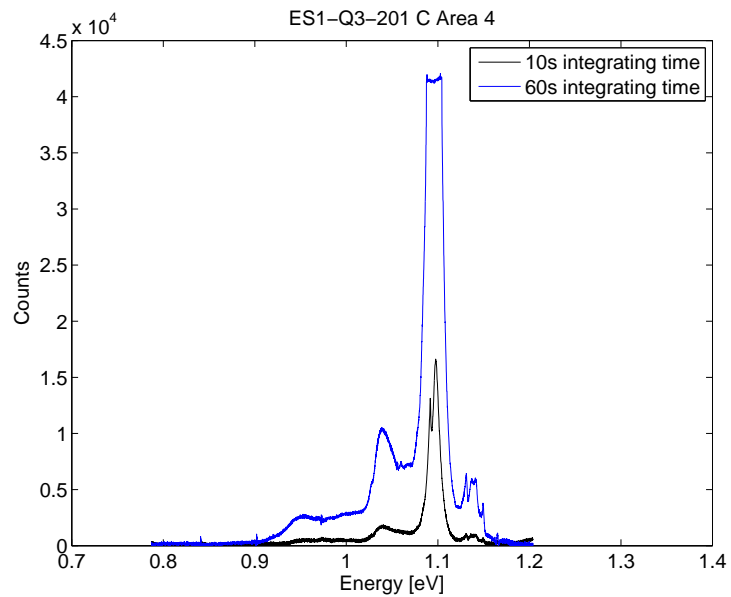
Figure 34: Sample ES1-Q3-201 C pumped with 128 mW at 14 K in a dislocation line (Area 4 in figure 29). For 60s integration, the main TO line around 1.1eV is saturating the camera.
