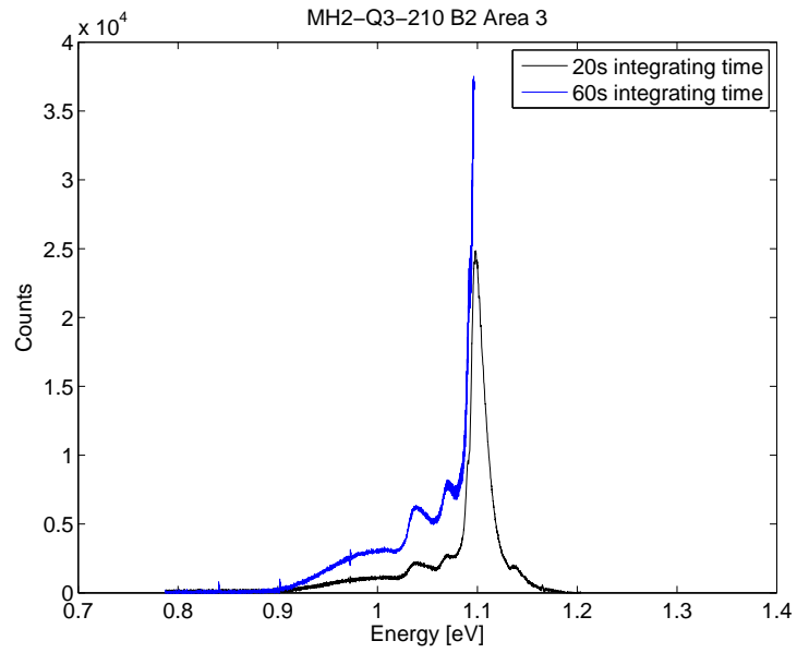
Figure 42: Sample MH2-Q3-210 B2 pumped with 128 mW at 12 K in a defect dot (Area 3 in figure 37) with 20s integration time (black) and 60s integration time (blue). The 60s integration time has an estimated mean dark current offset subtracted, in addition to measured dark current due to a change in the dark current in between measurements.
