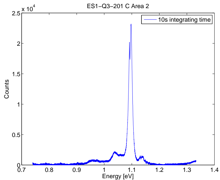
Figure 32: Sample ES1-Q3-201 C pumped with 128 mW at 12 K in a defect dot (Area 2 in figure 29).
