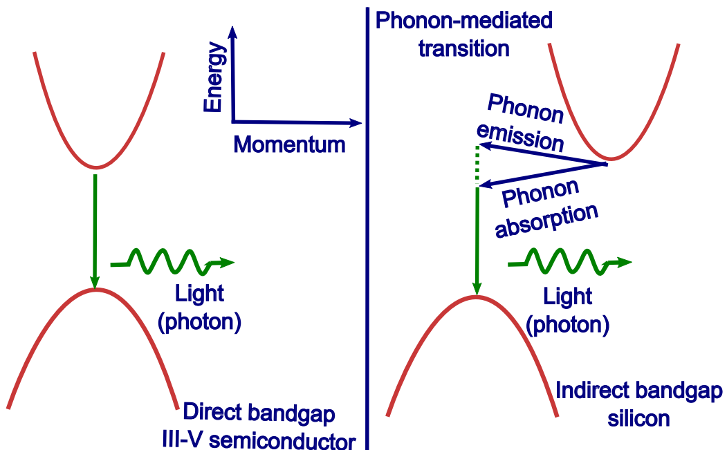
Figure 5: Direct and indirect recombination (figure from [1])
