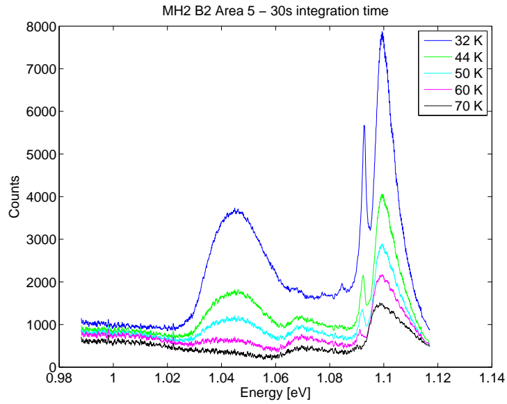
Figure 45: Sample MH2-Q3-210 B2 pumped with 16 mW at different temperatures in a defect free area (Area 5 in figure 37). Results are Savitzky-Golay filtered for easier comparison.
