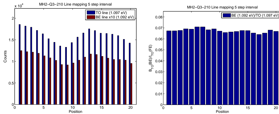
Figure 66: Sample MH2-Q3-210 B2 pumped with 128 mW at 14 K line map using 20 small steps exactly 5 times larger than in figure 65. Looking at TO and BE line only from results in figure 47.
