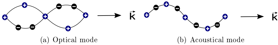
Figure 15: Transverse phonon modes
