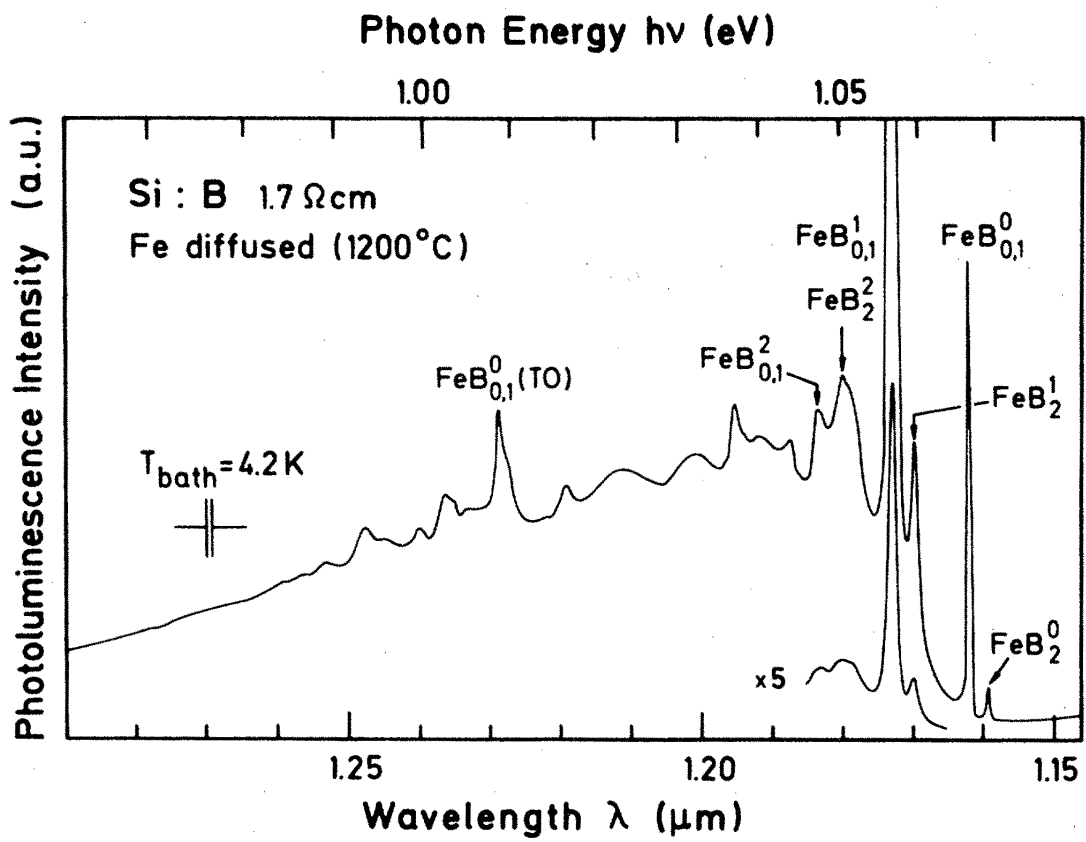
Figure 79: Iron diffused boron doped Si sample from [9]
