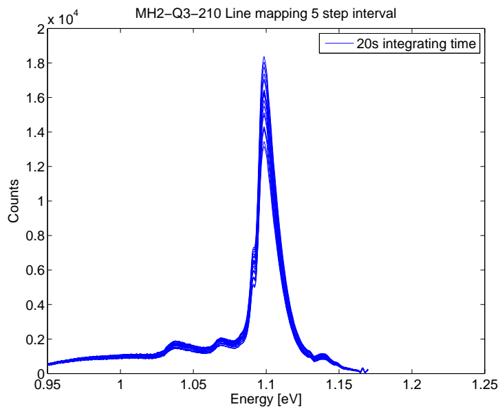
Figure 47: Sample MH2-Q3-210 B2 pumped with 128 mW at 14 K line map L2 in figure 37 using 20 steps exactly 5 times larger than in figure 46.
