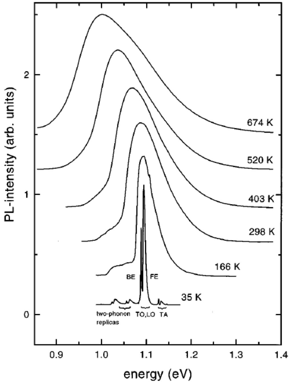
Figure 19: Normalized photoluminescence spectra of a 0.5 \Omega cm boron doped Si sample with surface passivation by a 100 nm thermal oxide, recorded at different temperatures from [5]
