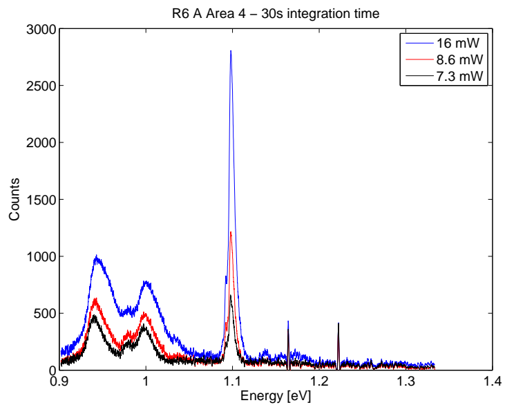
Figure 27: Sample R6-Q3-210 A - pumped with different intensities at 22 K in a grain boundary (Area 4 in figure 23). Results are Savitzky-Golay filtered for easier comparison.
