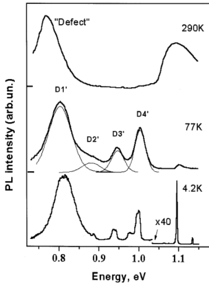
Figure 81: Dislocation related luminescence from mc-Si at different temperatures. The spectrum at 77 K is deconvolution numerical to resolve four individual Gaussian peaks. From [11].
