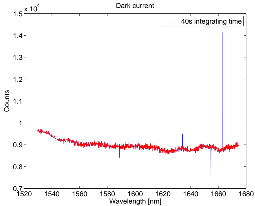
Figure 49: Dark current signal from the camera with defective pixel correction in red using a random center wavelength
