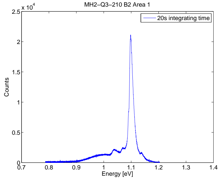
Figure 40: Sample MH2-Q3-210 B2 pumped with 128 mW at 12 K in a defect free area (Area 1 in figure 37).
