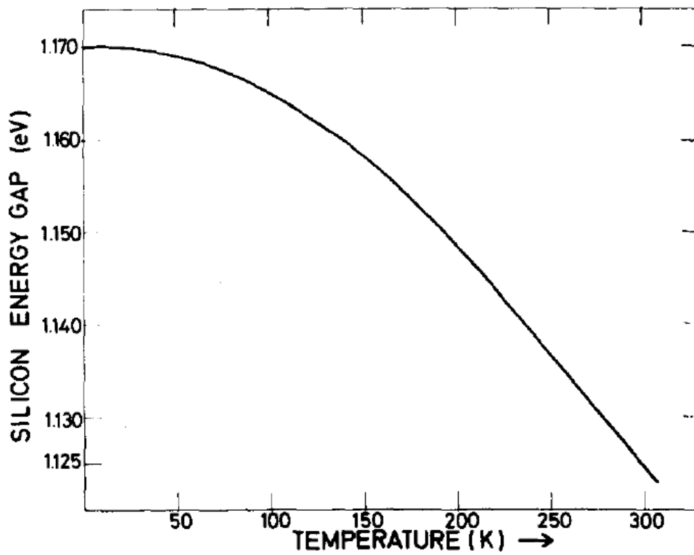
Figure 18: Temperature dependence of the intrinsic energy gap from [4]
