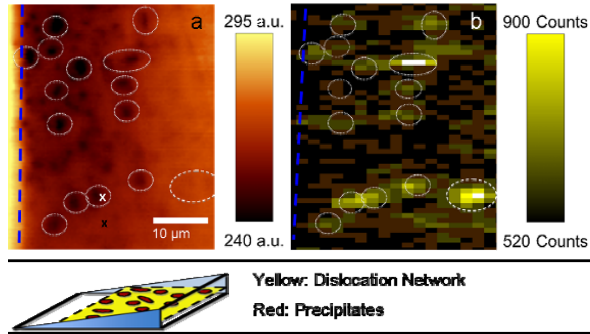
Figure 21: Bottom: Scheme of the sample preparation with the polished angle. Top: A Intensity of the BB PL peak at room temperature (a), and of the iron X-ray K\alpha fluorescence (b) from [23]. The dislocation network intersects the surface to the right of the dashed blue line. The white circles show recombination active precipitates.
