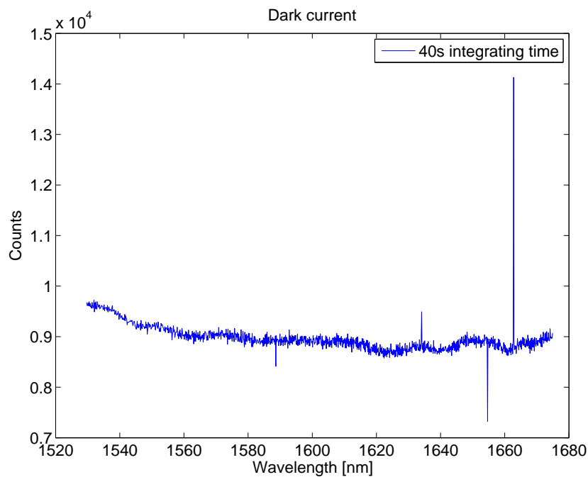
Figure 48: Dark current signal from the camera with defective pixels with shutter closed, and CCD at -75^{\circ}\text{C} using a random center wavelength
