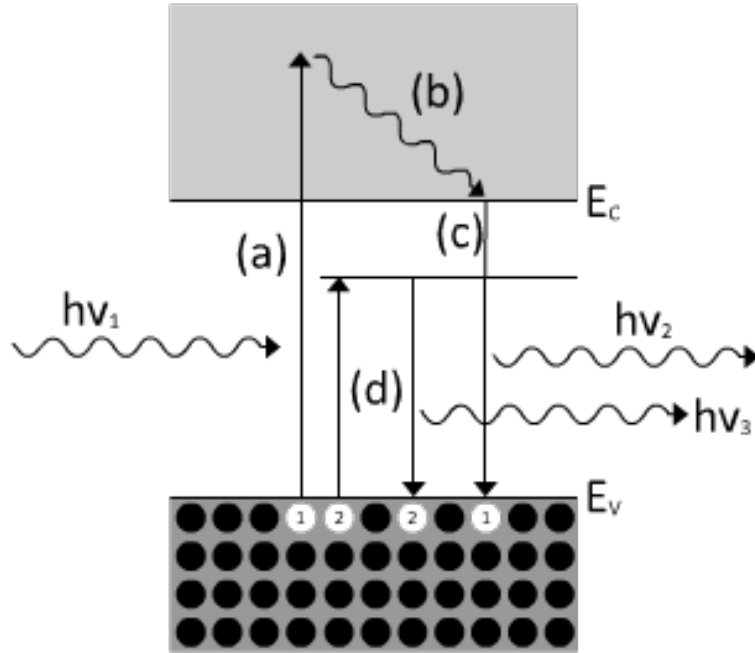
Figure 14: Excitation and recombination [3]
