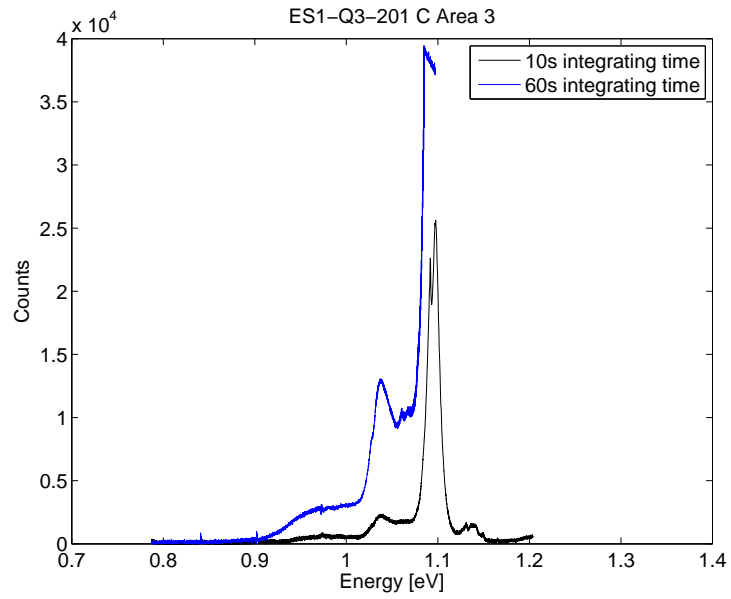
Figure 33: Sample ES1-Q3-201 C pumped with 128 mW at 12 K in a grain boundary (Area 3 in figure 29). For 60 s integration time, the main TO line at 1.1 eV is saturating the camera.
