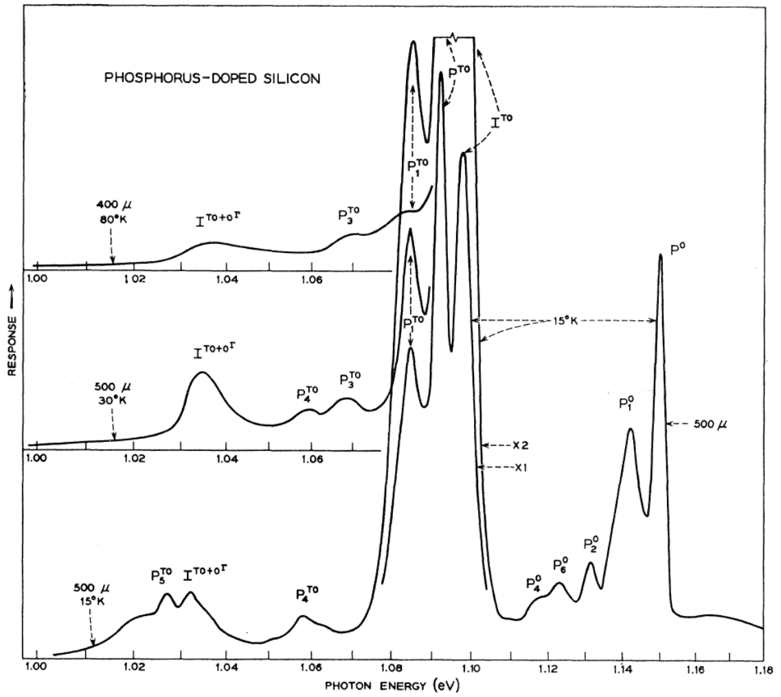
Figure 76: Phosphorus doped ( 8 \cdot 10^{16} \text{cm}^{-3} ) Si PL specter from [6]
