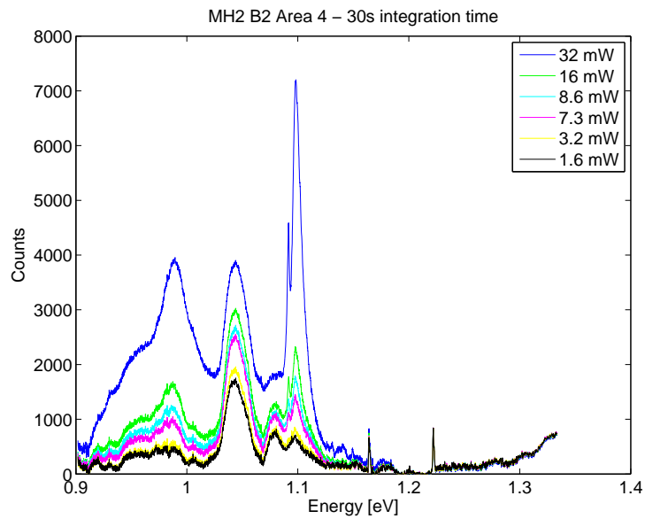
Figure 43: Sample MH2-Q3-210 B2 pumped with different intensities at 27 K in a grain boundary (Area 4 in figure 37). Results are Savitzky-Golay filtered for easier comparison.
