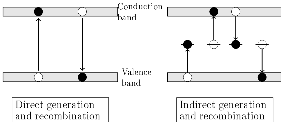
Figure 4: Generation and recombination
