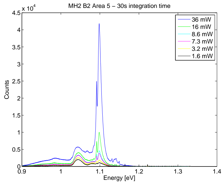
Figure 44: Sample MH2-Q3-210 B2 pumped with different intensities at 27 K in a defect free area (Area 5 in figure 37). Results are Savitzky-Golay filtered for easier comparison.
