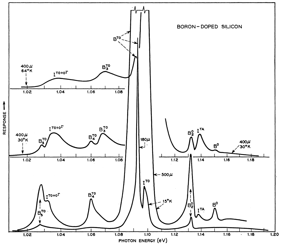
Figure 75: Boron doped ( 6 \cdot 10^{16} \text{cm}^{-3} ) Si PL spectrum from [6]
