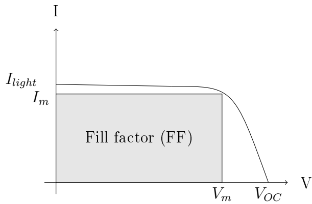
Figure 8: Current-voltage characteristics with fill factor
