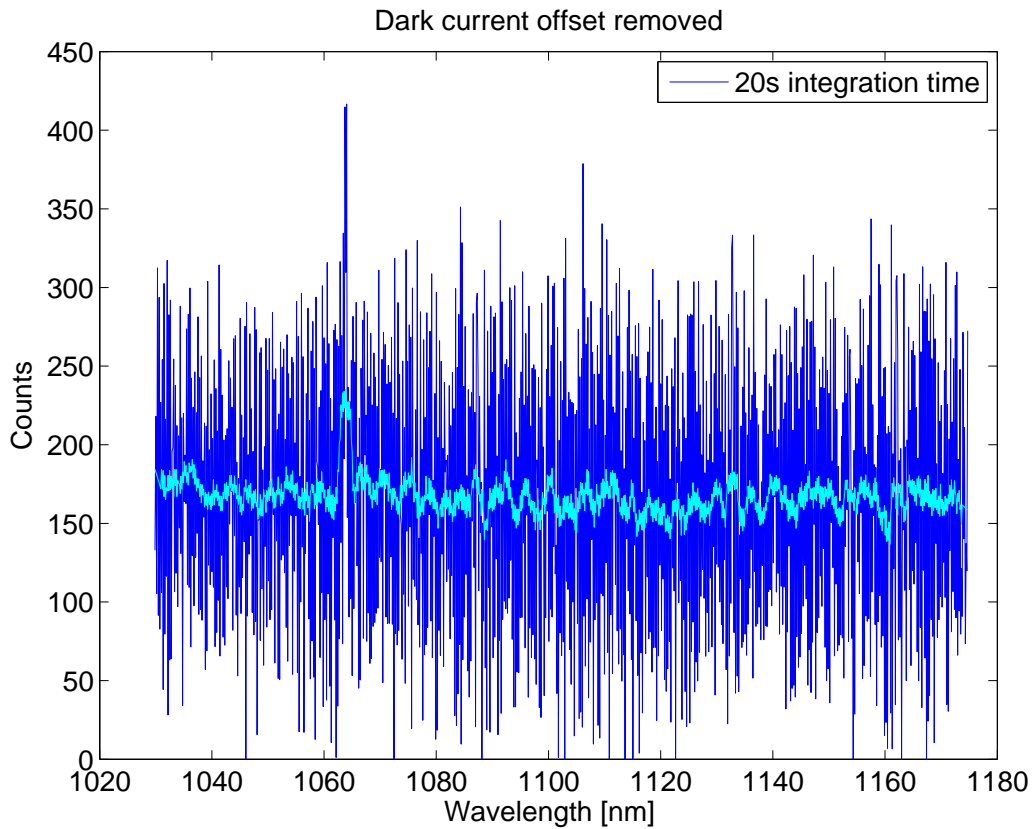
Figure 52: Dark current removed from background noise (blue), and Savitzky-Golay filtered signal (cyan)
