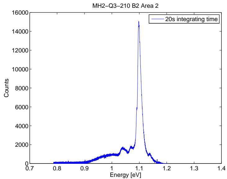
Figure 41: Sample MH2-Q3-210 B2 pumped with 128 mW at 12 K in a dislocation line (Area 2 in figure 37).
