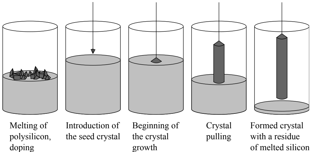
Figure 10: Czochralski process
