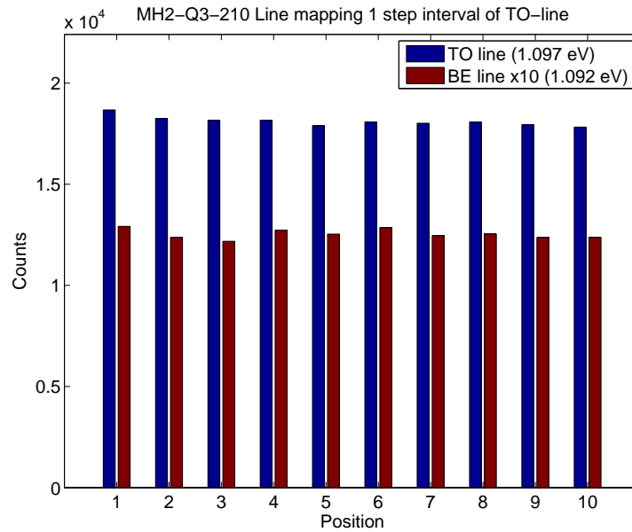
Figure 65: Sample MH2-Q3-210 B2 pumped with 128 mW at 14 K line map using 10 small steps, looking at TO and BE line only from results in figure 46.
