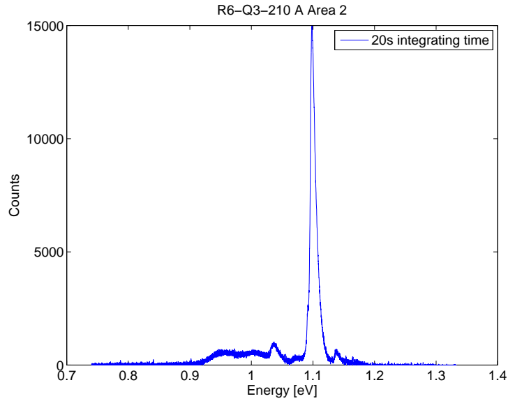
Figure 25: Sample R6-Q3-210 A - pumped with 128 mW at 10 K in a defect dot (Area 2 in figure 23).
