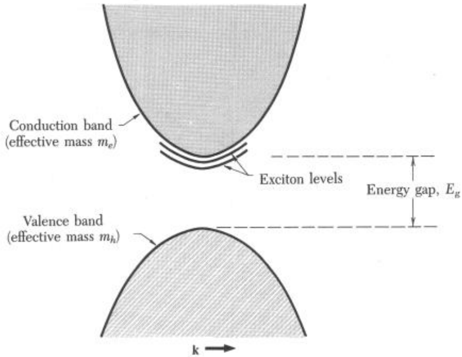
Figure 17: Exciton levels in relation to the conduction band edge for a simple band structure with both conduction and valence band edges at \vec{k}=0 . Figure from [22]
