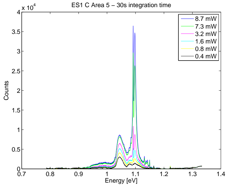
Figure 35: Sample ES1-Q3-201 C pumped with different intensities at 22 K in a defect free area (Area 5 in figure 29). Results are Savitzky-Golay filtered for easier comparison.
