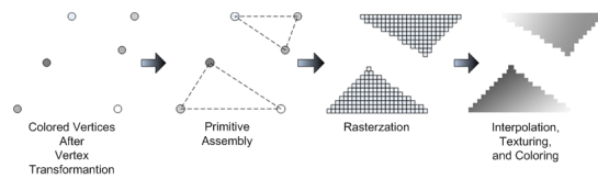
FIGURE E.3: In the graphics pipeline stages the initial data are colored before making the primitives. The primitives can be triangles or lines. By rasterizing and interpolating the primitives, a visible object is made. Figure are from [18].
