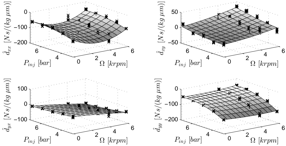
Figure 12: Identified damping coefficients as function of injection pressure P_{inj} ( 1bar = 0.1MPa ) and rotational speed \Omega , along with 2^{nd} order polynomial fit, assisting lines indicate 3D location of the parameter estimates.
