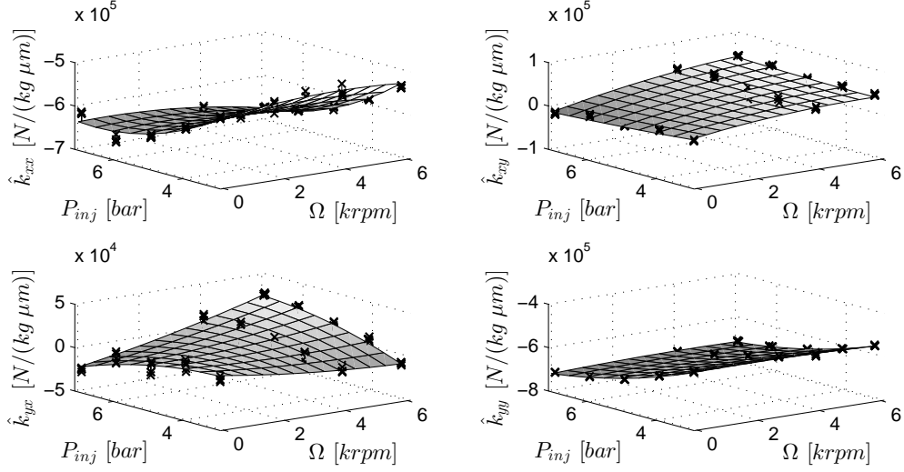
Figure 11: Identified stiffness coefficients as function of injection pressure P_{inj} ( 1bar = 0.1MPa ) and rotational speed \Omega , along with 2^{nd} order polynomial fit, assisting lines indicate 3D location of the parameter estimates.
