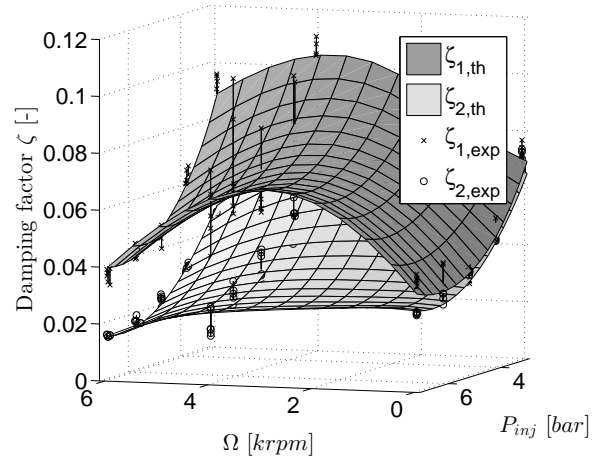
Figure 17: Damping factors of experimentally identified models and the linear parameter varying model Eq. 17 over varying speed and injection pressure, ( 1\text{bar} = 0.1\text{MPa} ).
