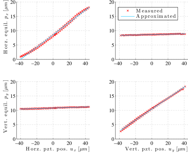
Figure 5: Steady state characterization of input-output gains at \bar{P}_{inj} = 6bar , \bar{\Omega} = 0rpm : the experimental data reveal a linear mapping from \mathbf{u} to lateral disc position \mathbf{p} .
