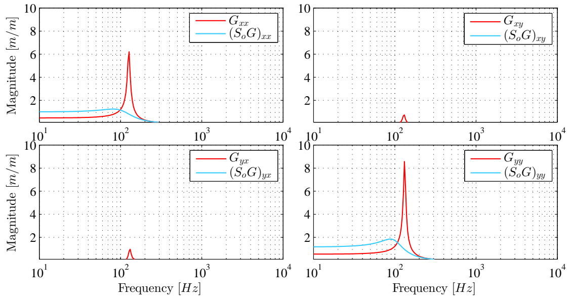
Figure 21: Bode magnitude diagram for the open loop system G and closed input disturbance response S_o G for the controller K_{pl} .
