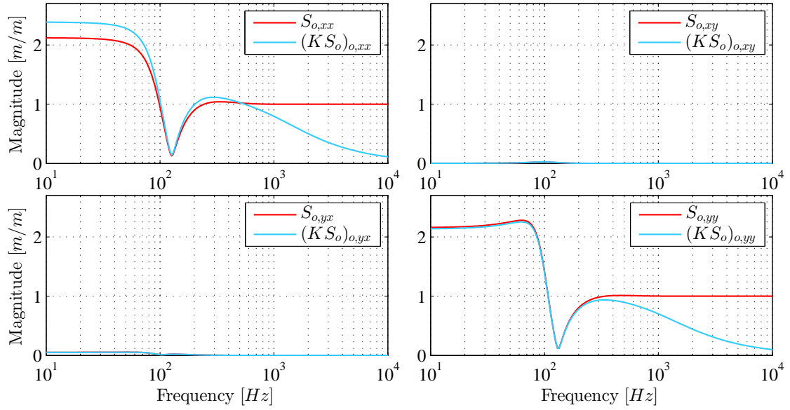
Figure 20: Output sensitivity S_o and closed loop controller sensitivity K_{pl}S_o for the controller K_{pl} .
