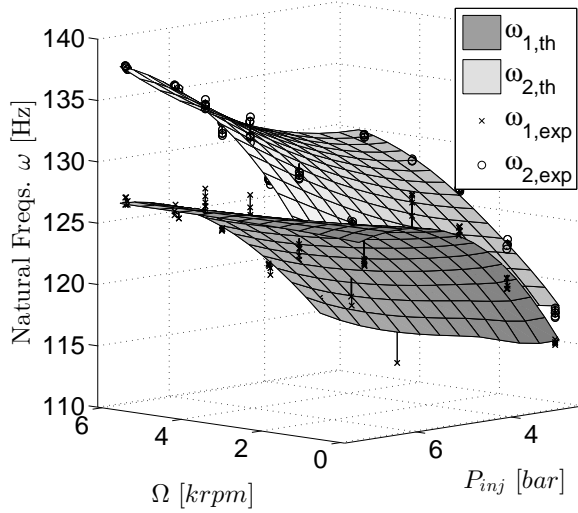
Figure 16: Natural frequencies of the experimentally identified models and the linear parameter varying model Eq. 17 over varying speed and injection pressure, ( 1\text{bar} = 0.1\text{MPa} ).
