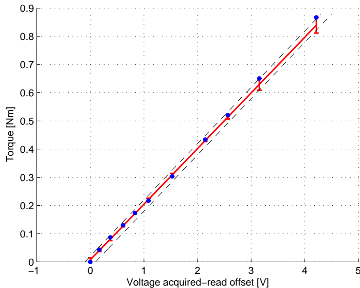
Figure 3.13: Typical torque transducer calibration curve.
