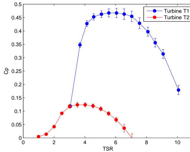
Figure 3.18: Power coefficient curves for the two turbine models running with a downstream separation distance of 3D. The second turbine curve is obtained with the first turbine running at optimum TSR. The errorbars represent the evaluated accuracy.
