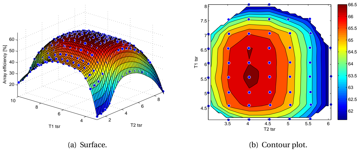
Figure A.6: Array efficiency (Configuration B: 5D downstream distance and low turbulence background level).
