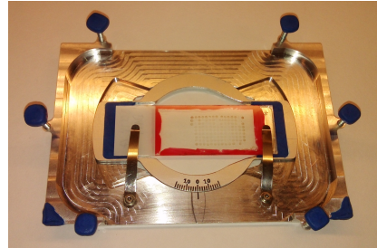
(b) Sample holder with adjustment of specimen-plane.
