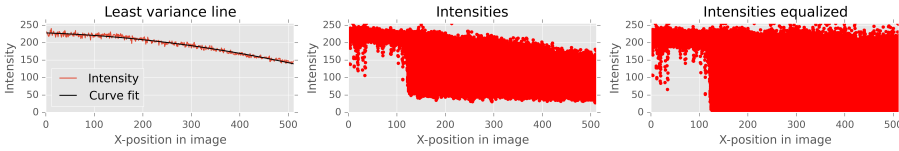
Figure 3.2: (a) Intensities for the line with least variance of figure 3.1(b). The curve is fitted to a second degree polynomial to supress noise. (b) Intensities for image in figure 3.1(b). Each dot represents a pixel. (c) Intensities for the equalized image in figure 3.1(c). Each dot represents a pixel. Note that the intensities is both spread across the whole intensity range (0-255) and the skewness is fairly straightened out.
