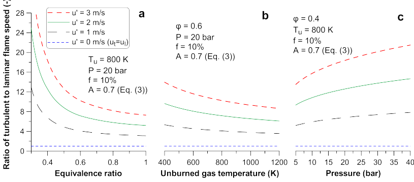
Figure 2.4: Effect of (a): equivalence ratio, (b): unburned gas temperature, and (c): pressure and turbulence intensity, on the ratio of turbulent to laminar flame speed under engine-relevant conditions (Rakopoulos et al. [33]).
