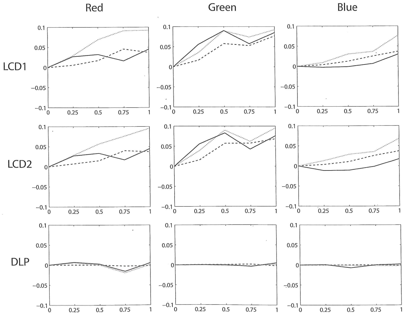
Figure 9. Channel interaction for three displays. The horizontal axis represents the input value of the denoted channel, while the vertical axis represents the calculated interaction value. The solid black line is the interaction found when the two other channels are kept at maximum input value, while the dashed and the dotted lines are when the a or b , respectively, is set to 0 when computing the interaction metric.
