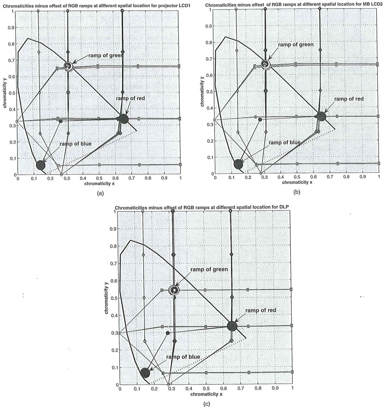
Figure 7. Illustration of the chromaticity constancy for the projectors at different locations, in (a) for projector LCD1, in (b) for projector LCD2 and in (c) for the DLP projector. In each figure the x and y chromaticity values are shown twice: once as a regular chromaticity diagram and second in the background of the figure in line and square versus the ramp digital steps in horizontal axis for the chromaticity x and in line and diamond versus the ramp digital steps in vertical axis for the chromaticity y. For clarity, the chromaticity of the average offset over the various locations has been used in the graphs.
