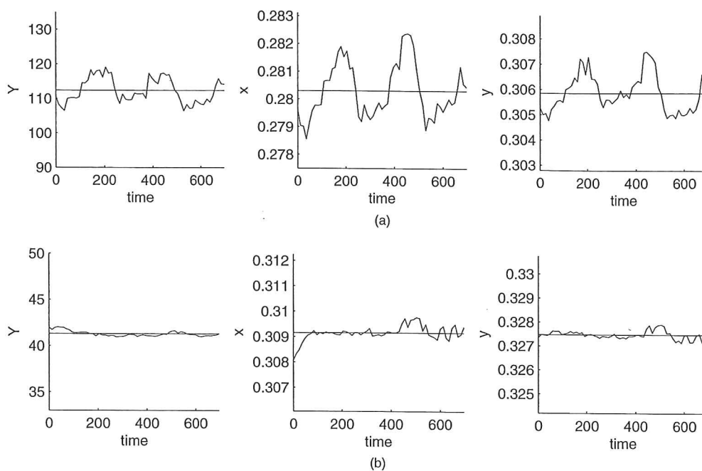
Figure 2. Visualizations of the temporal shift for the DLP and one of the LCD tested projectors. The ordinate boundaries of these graphs correspond to the 20% error around the mean for Y and the 1% around the mean for x and y . One can notice that the DLP is less stable than the LCD. However, both devices appear to be stable enough to be used in normal applications. We can notice that for the LCD projector, there is an optimal time between the warming up time and a overheat time.
