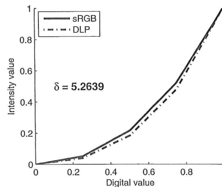
Figure 6. Normalized response curve of the DLP projector compared with the normalized sRGB response curve. The indicator \delta is the surface between both curves \times 1000 .
