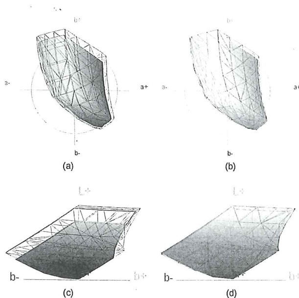
Figure 4. The gamut boundaries for two of the projectors at the position with the highest luminance (wireframe) compared with the gamut of the top left corner (solid and wireframe). CIELAB measurement values were computed relatively to the global white point for (a) and (c), while (b) and (d) utilizes the white point of each location.
