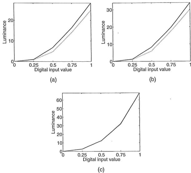
Figure 8. The luminance of the gray ramp (solid line) compared with the sum of the individual ramps (dashed line) for the three projectors.
